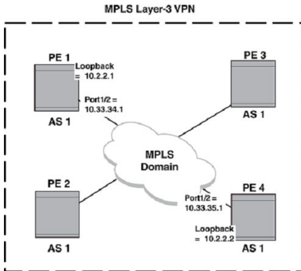
Figure 36: IBGP example
