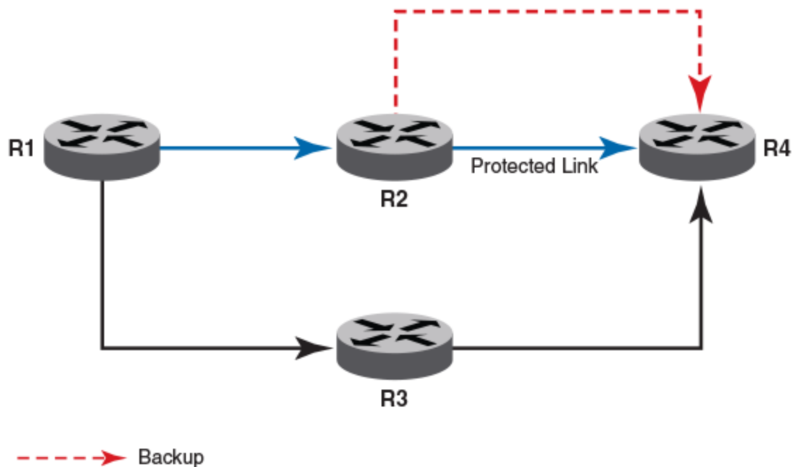
Figure 22: Link protection
