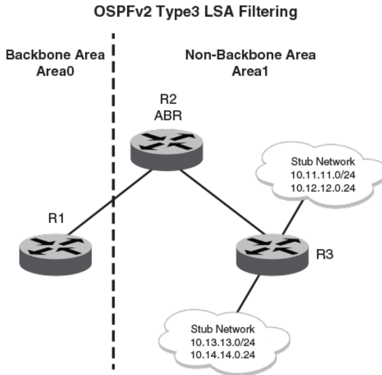
Figure 57: OSPFv2 type 3 LSA filtering
