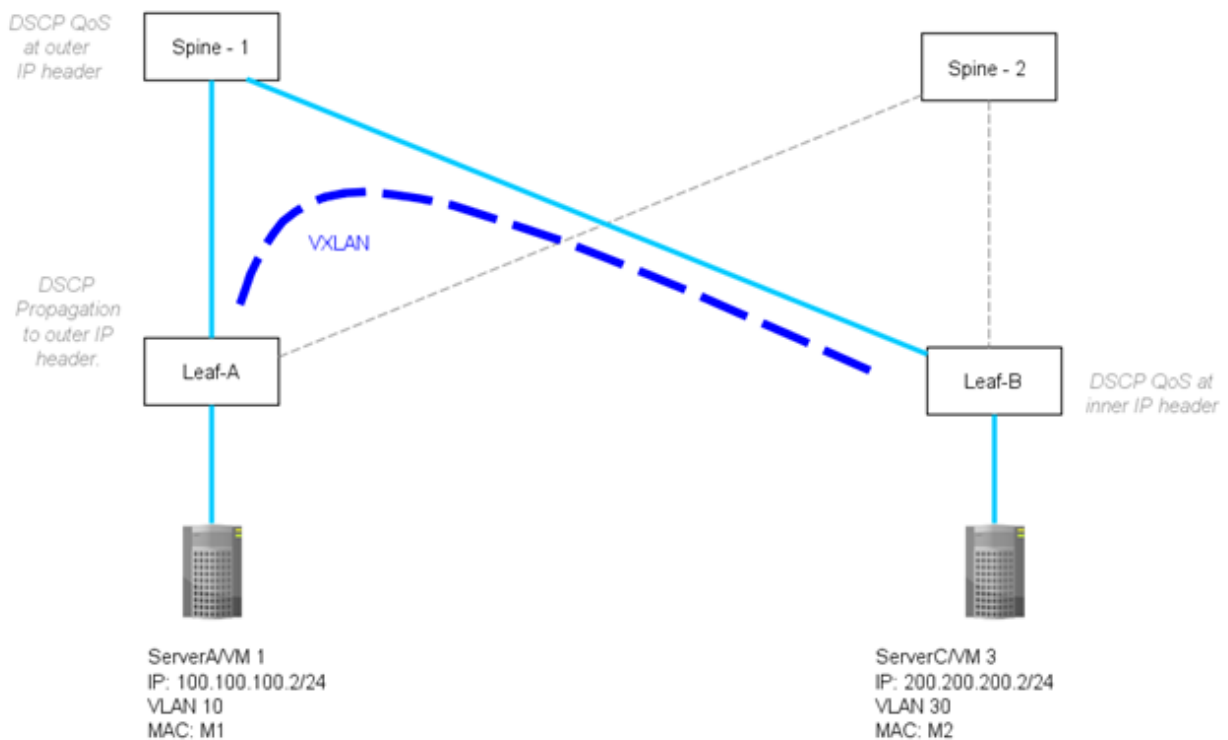
Figure 70: VXLAN L3 gateway support of intersubnet communication
