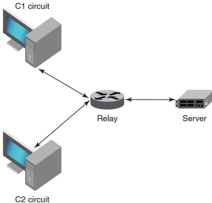
Figure 37: IP DHCP relay function
