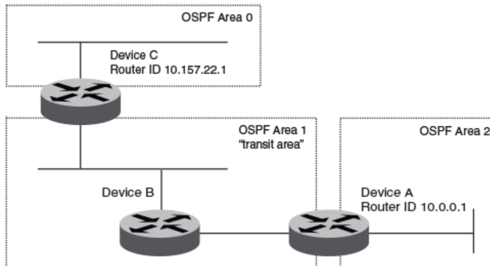
Figure 56: Defining OSPF virtual links within a network
