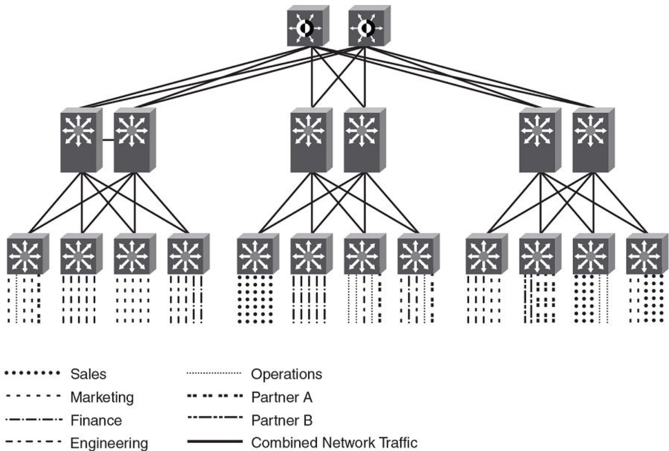
Figure 48: Generic high-level Multi-VRF topology
