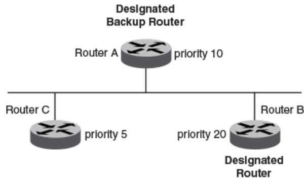
Figure 54: Designated and backup router election
