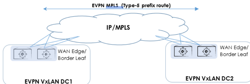
Figure 33: EVPN Type-5 prefix route termination and reorigination on the WAN edge
