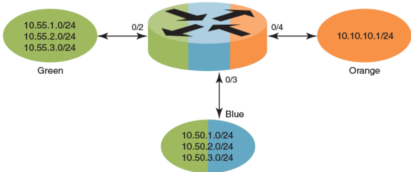
Figure 50: Static inter-VRF route leaking
