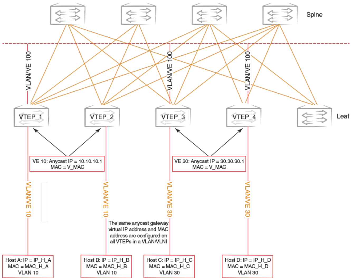
Figure 35: Static anycast gateway
