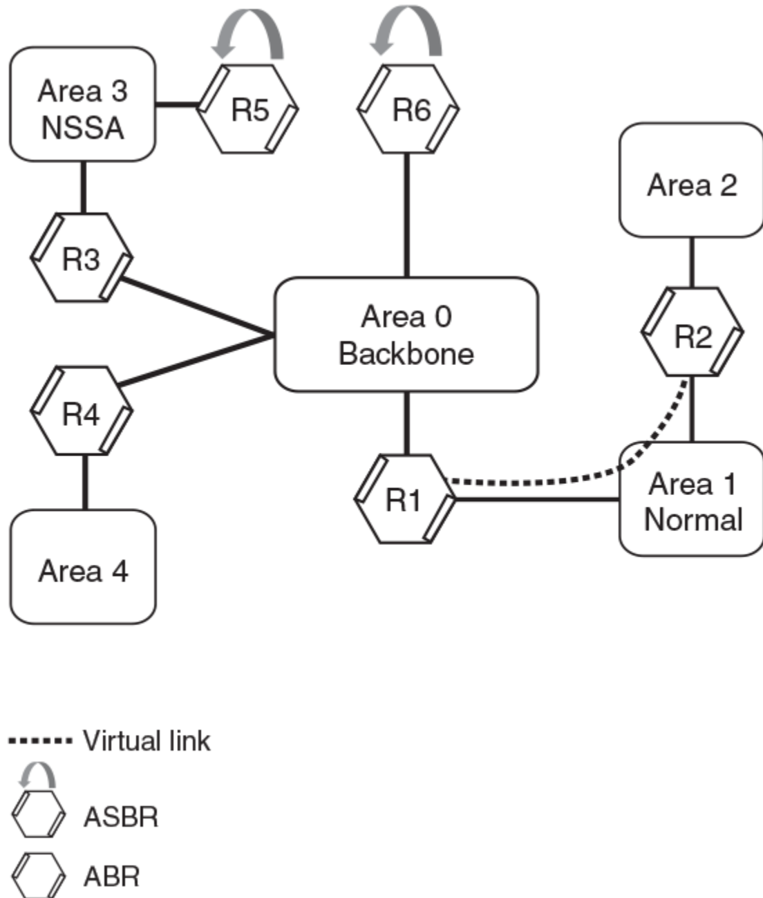
Figure 58: OSPFv3 virtual link
