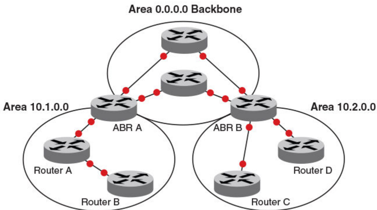
Figure 53: OSPF operating in a network
