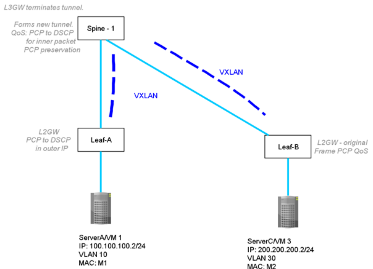
Figure 69: QoS for VXLAN Layer 2 and Layer 3 gateway interconnections
