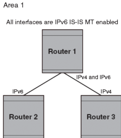
Figure 46: IS-IS non-congruent topology
