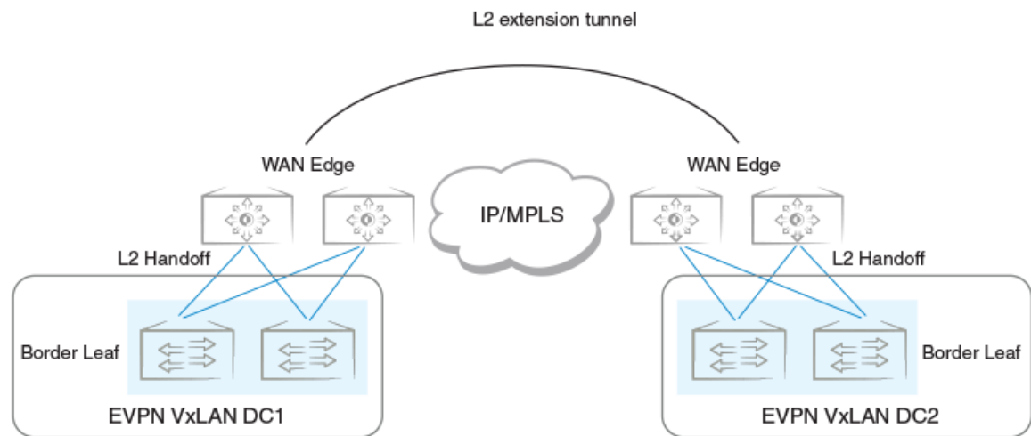
Figure 31: Layer 2 handoff-based DCI
