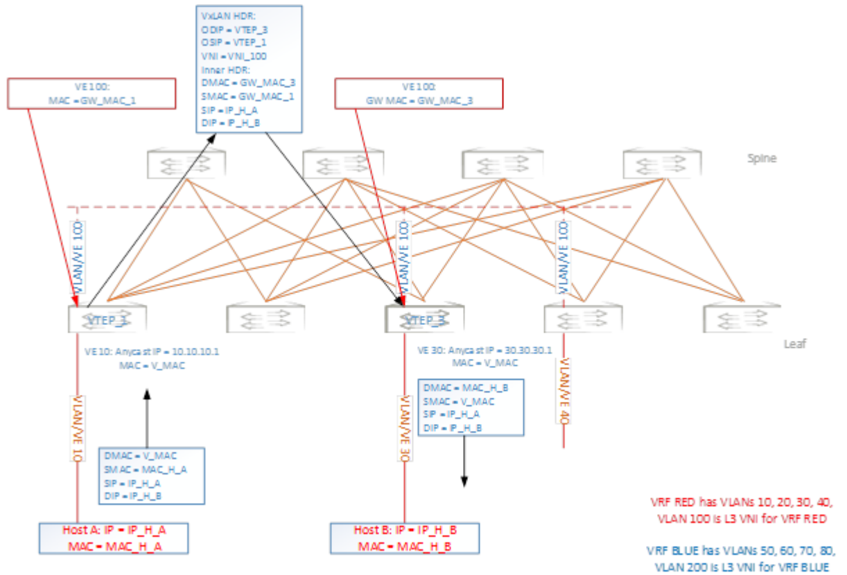
Figure 67: Layer 3 VNI on a single VTEP
