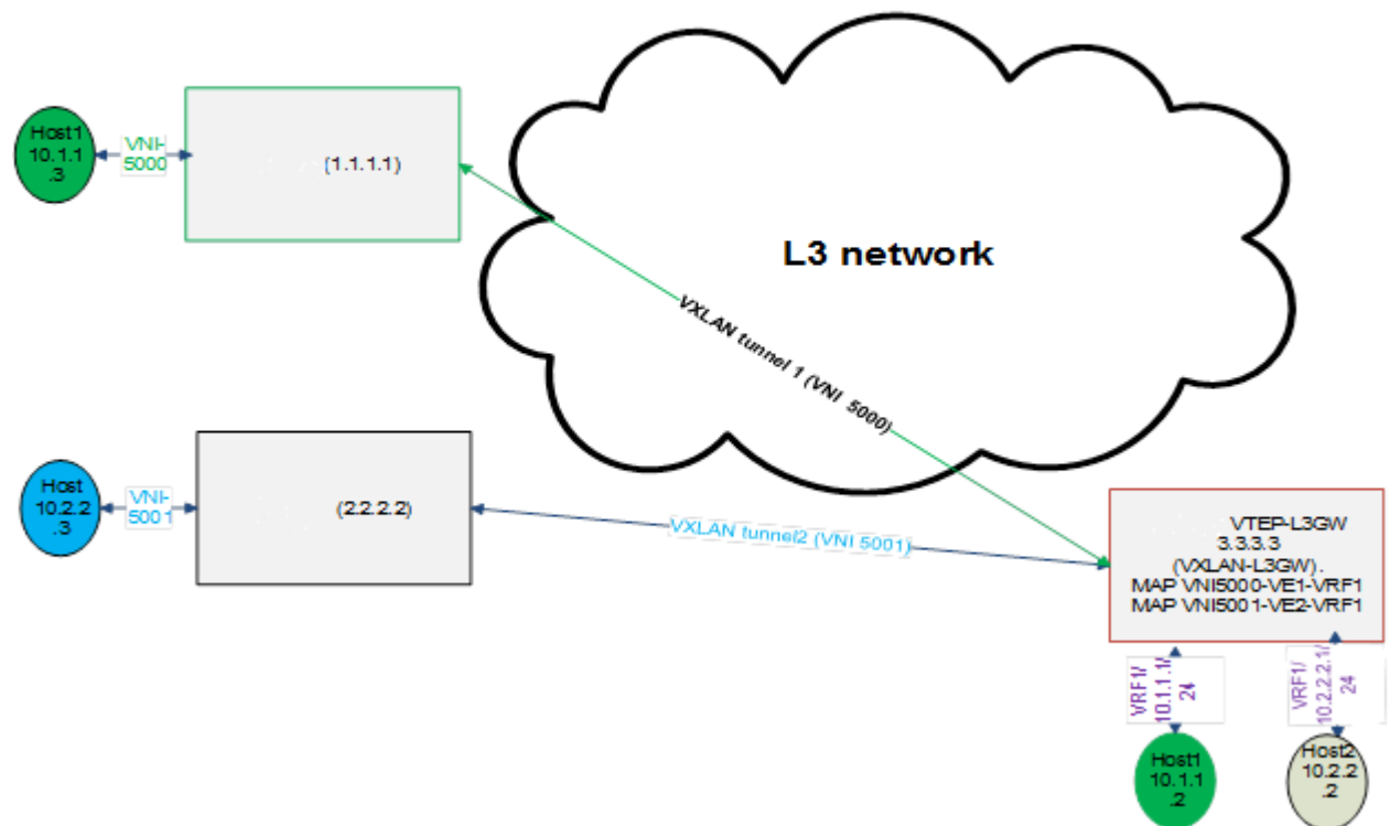
Figure 66: Static L3GW topology
