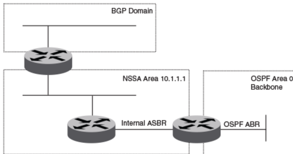
Figure 55: OSPF network containing an NSSA
