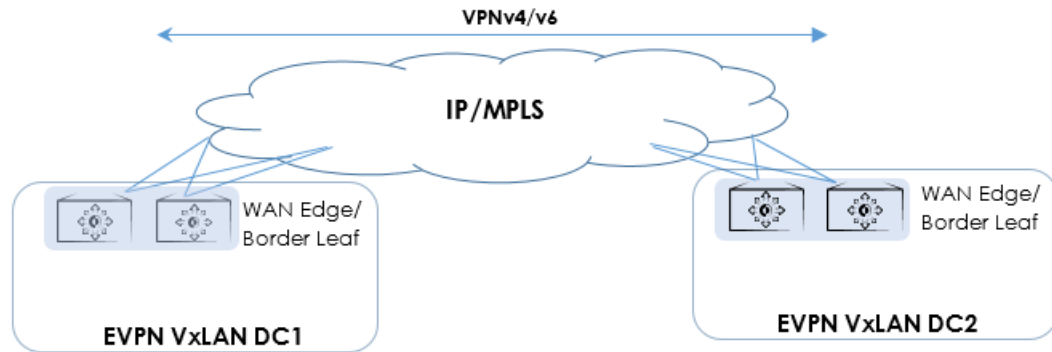
Figure 34: Data center Layer 3 interconnect with EVPN VXLAN and VPNv4/v6
