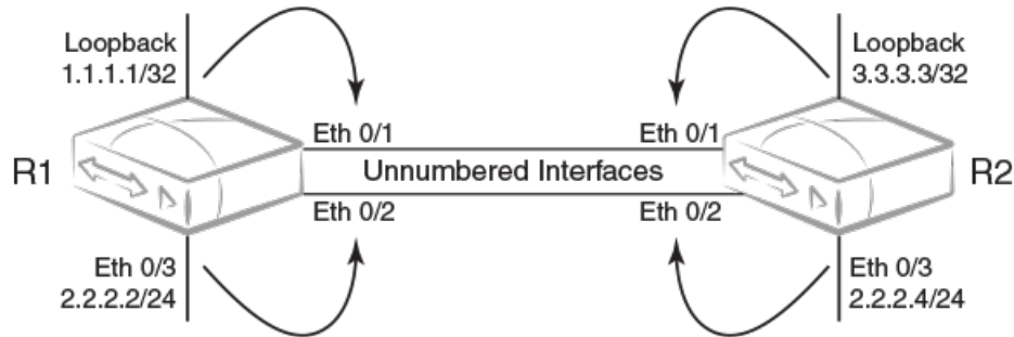
Figure 36: IP unnumbered and donor interfaces
