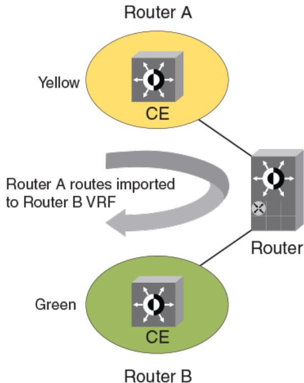
Figure 52: Dynamic inter-VRF route leaking
