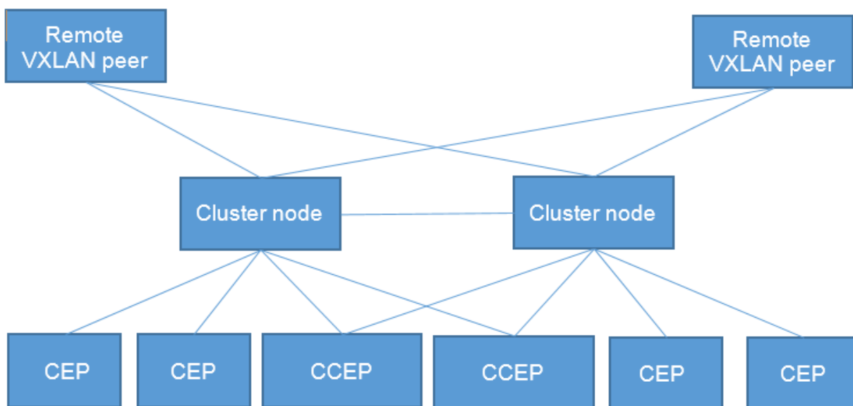
Figure 2: LVTEP topology
