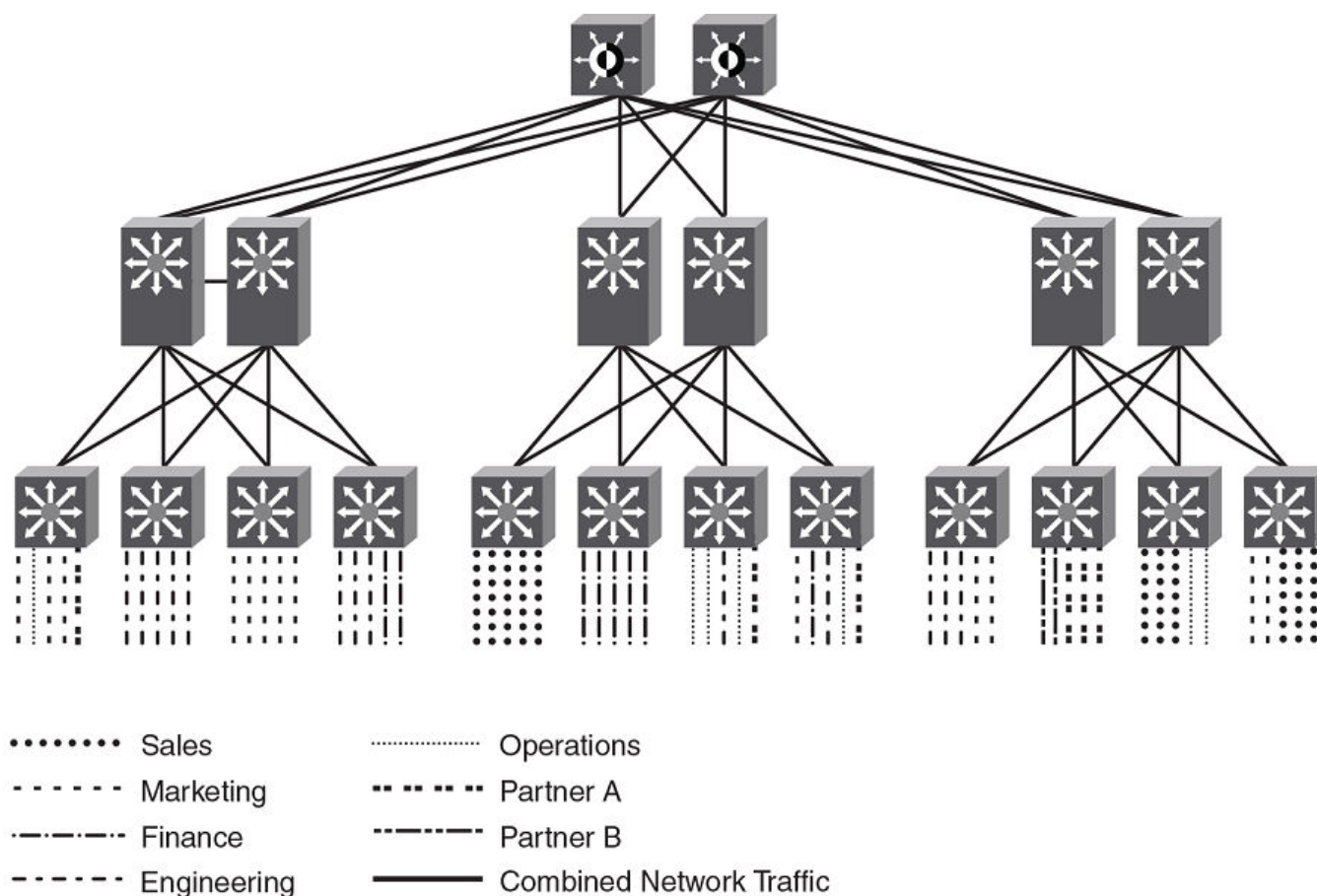
Figure 49: Generic high-level Multi-VRF topology
