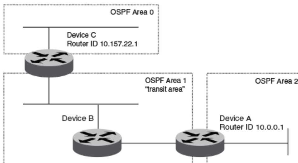
Figure 57: Defining OSPF virtual links within a network
