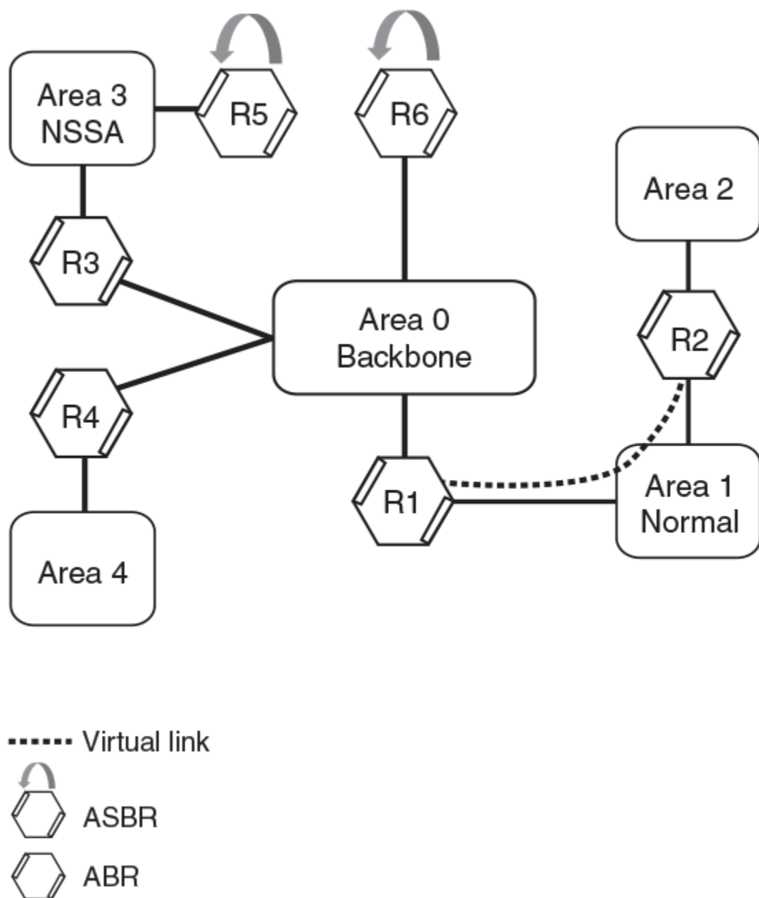
Figure 59: OSPFv3 virtual link
