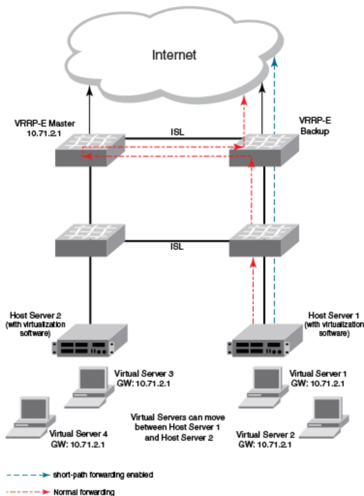
Figure 66: Short-path forwarding
