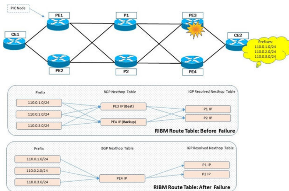
Figure 19: BGP PIC edge node failure
