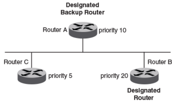
Figure 55: Designated and backup router election
