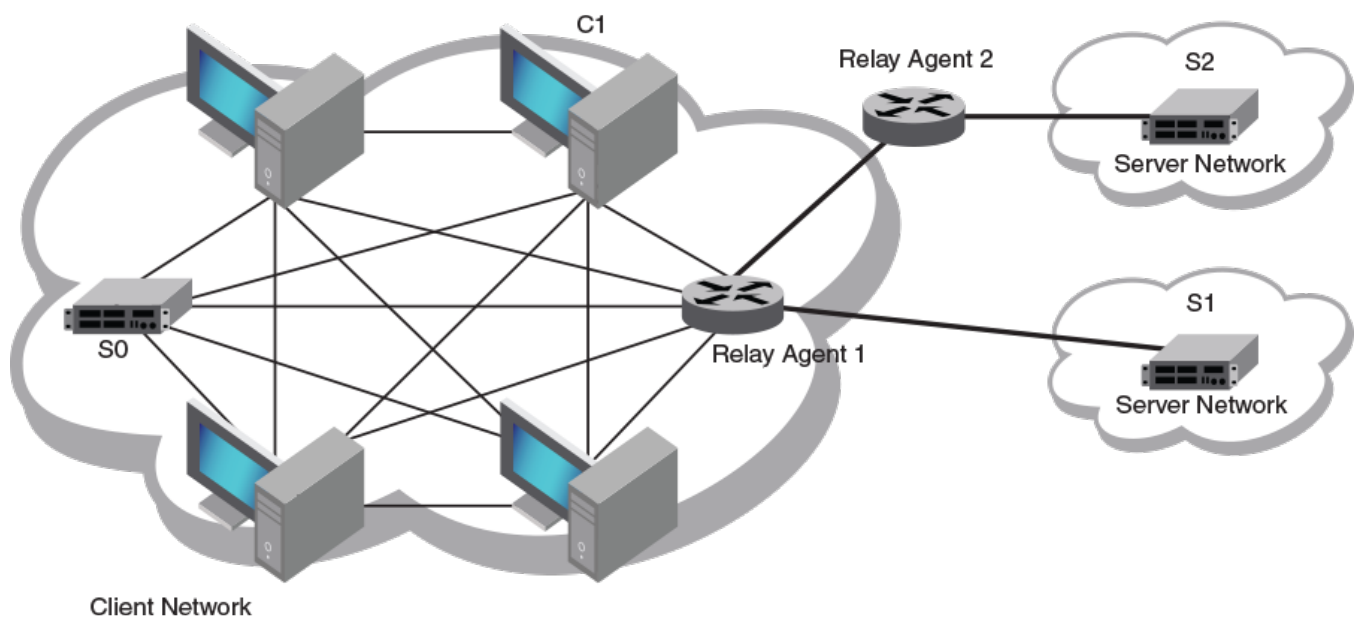
Figure 39: DHCP relay agent user scenarios
