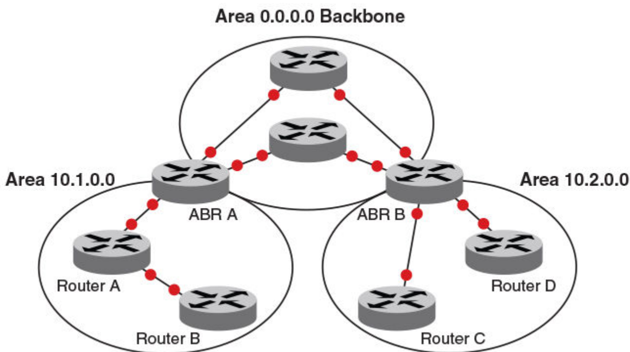
Figure 54: OSPF operating in a network
