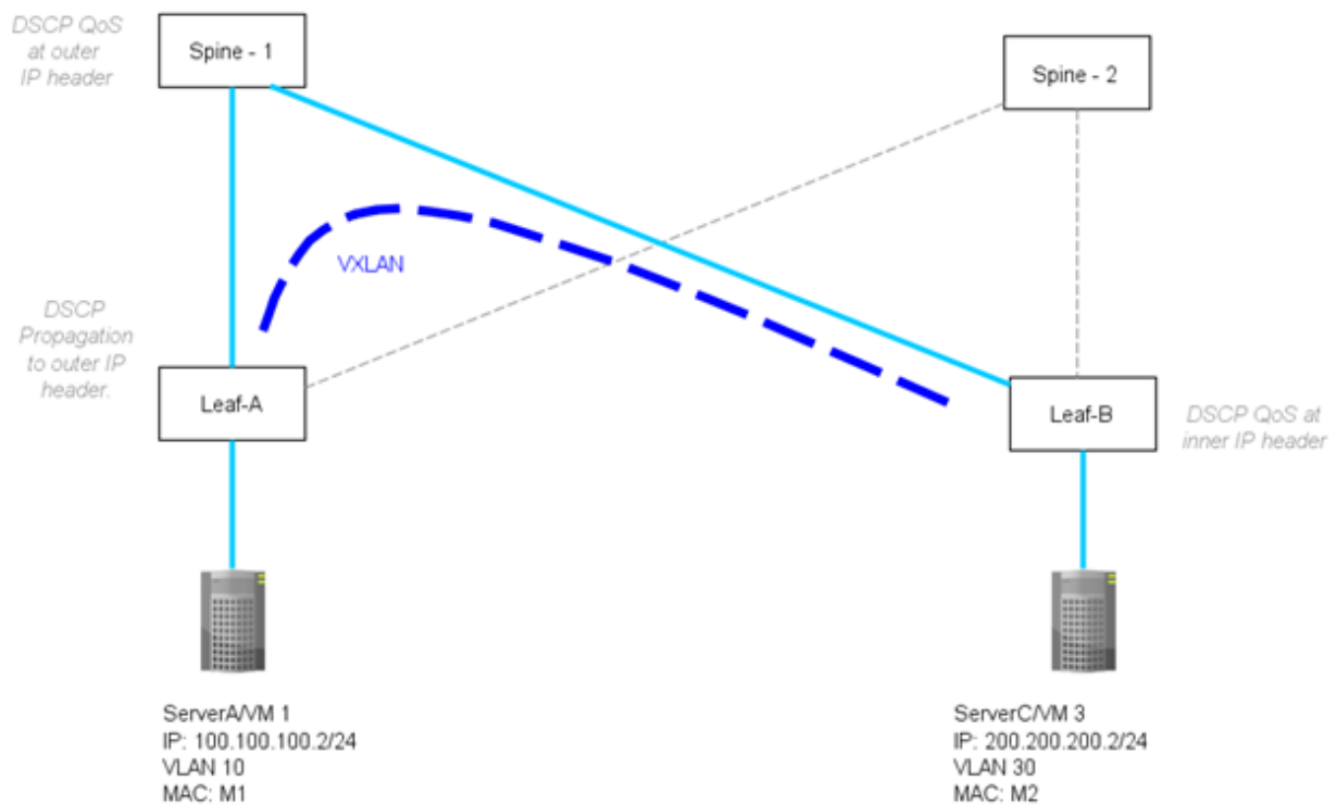
Figure 71: VXLAN L3 gateway support of intersubnet communication
