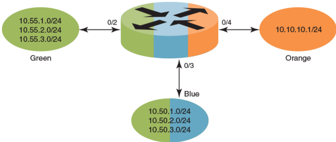
Figure 51: Static inter-VRF route leaking
