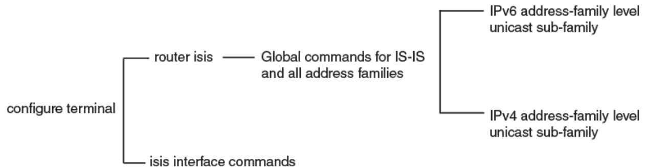
Figure 46: IPv6 IS-IS CLI levels
