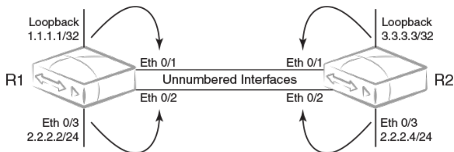
Figure 36: IP unnumbered and donor interfaces
