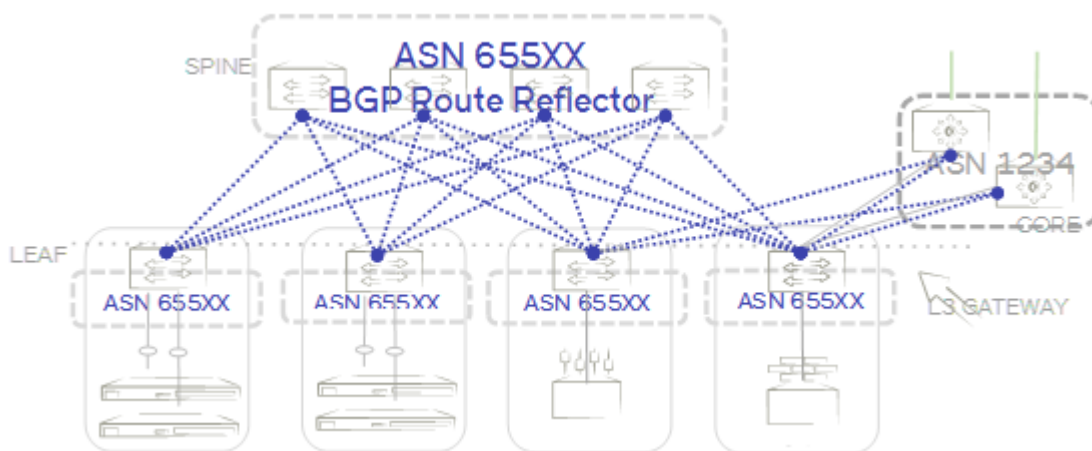
Figure 25: iBGP spine and leaf
