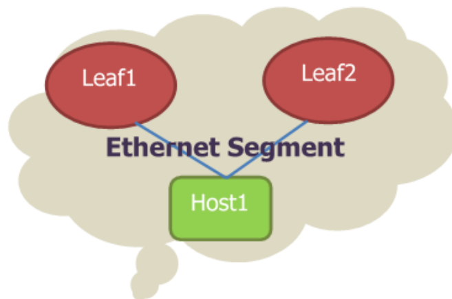
Figure 37: Ethernet Segment
