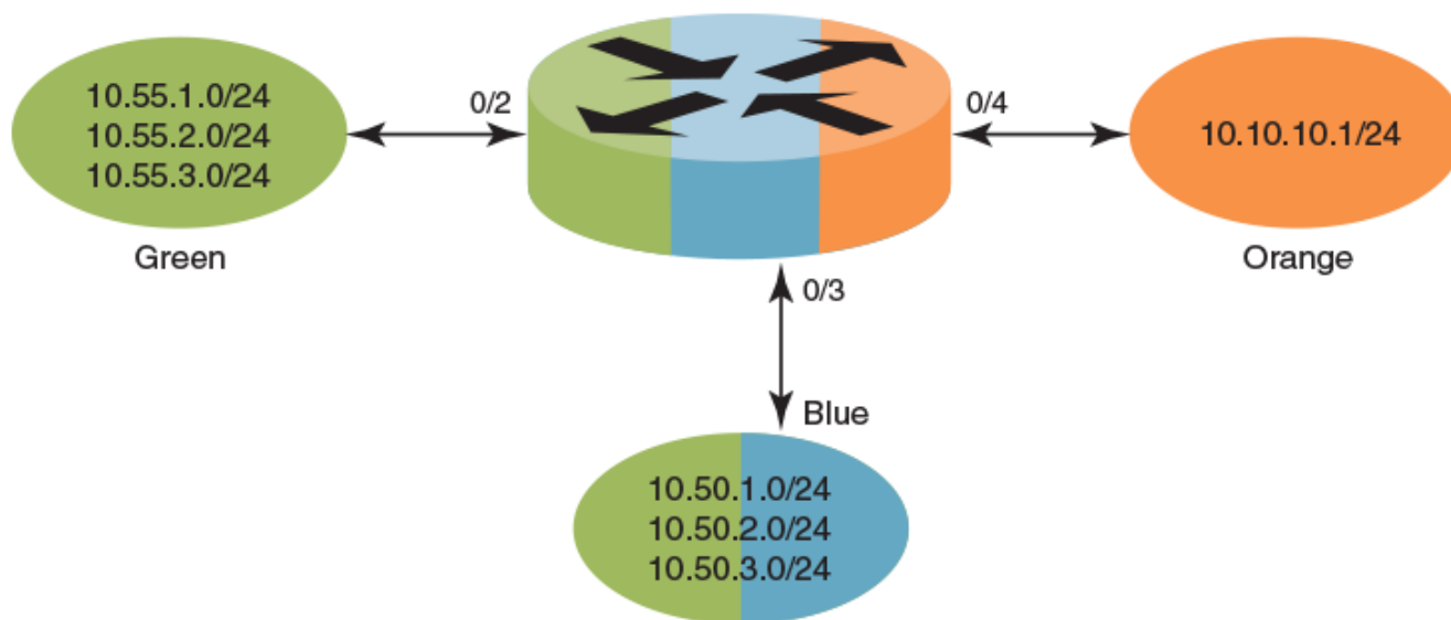
Figure 51: Static inter-VRF route leaking
