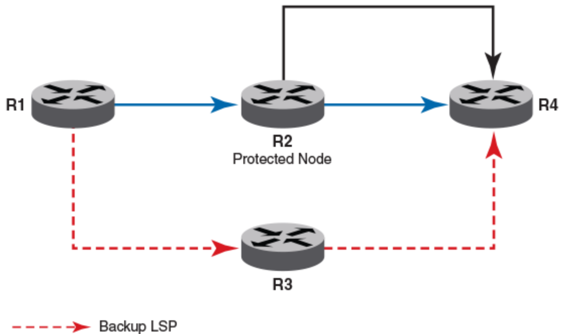
Figure 23: Node protection
