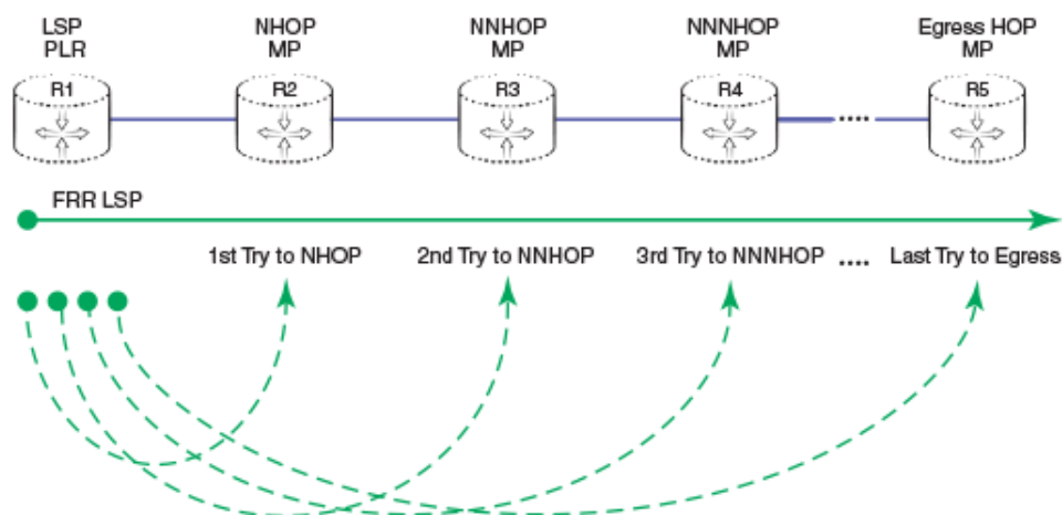
MergePoint selection order for LINK PROTECTION FRR (upon explicit link protection config)
