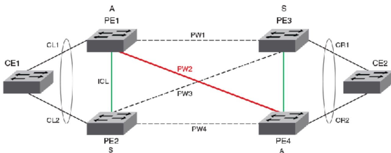
Figure 11: VLL MCT topology
