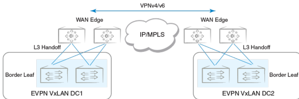
Figure 32: Layer 3 handoff-based DCI
