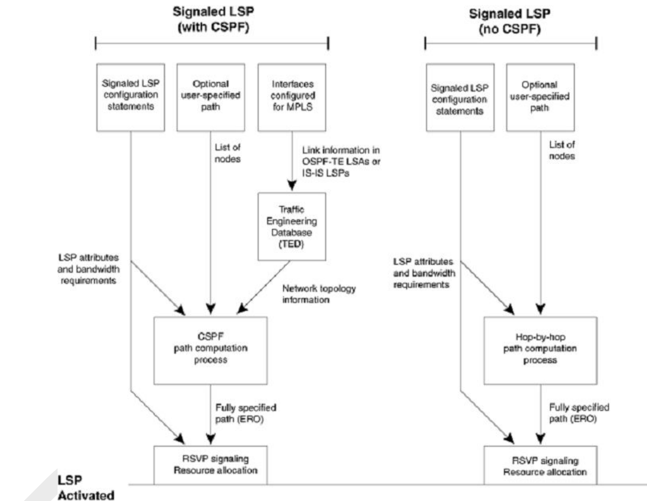
Figure 4: How traffic-engineered LSPs are configured, established, and activated
