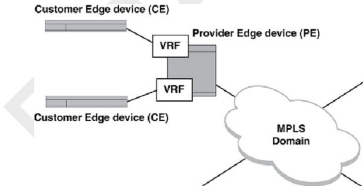
Figure 32: BGP or MPLS VPN components
