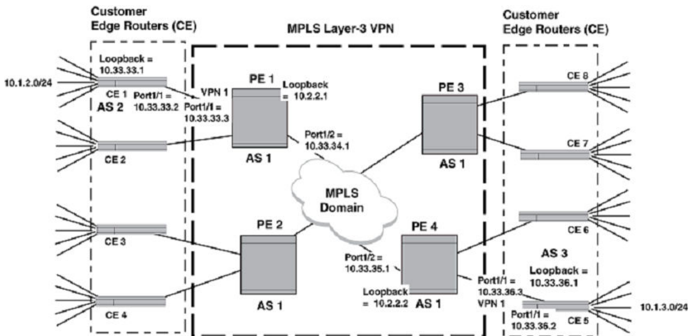
Figure 37: EBG to CE network example
