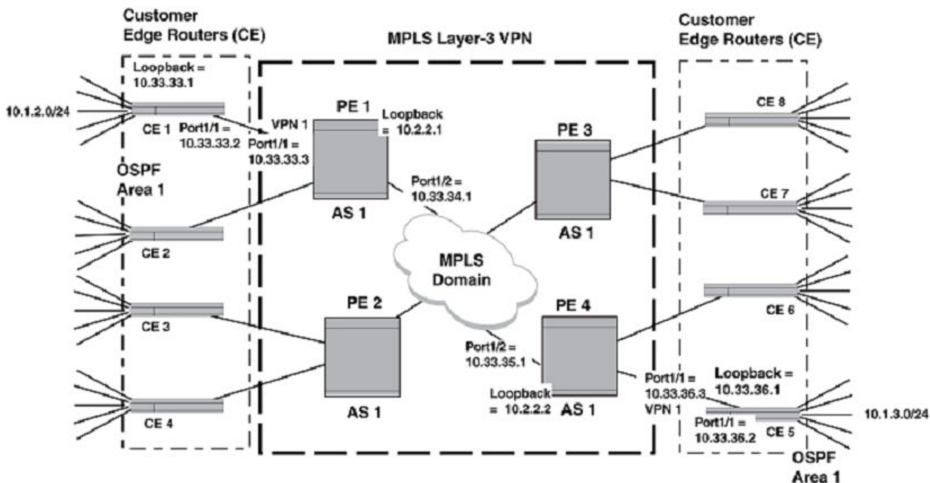
Figure 39: OSPF to CE network example
