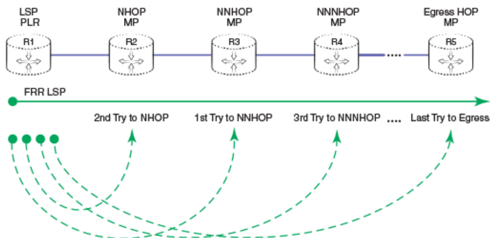
MergePoint selection order for NODE PROTECTION FRR (default behavior)
