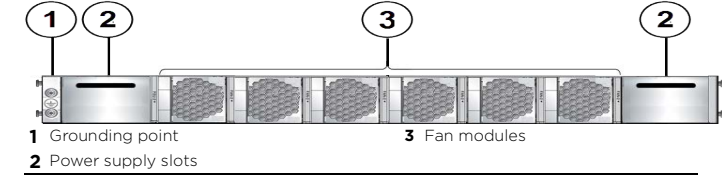
Figure 2 SLX 9250 Switch: Rear Panel
