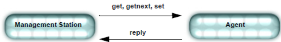
Figure 2: SNMP query
