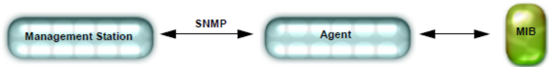
Figure 1: SNMP structure
