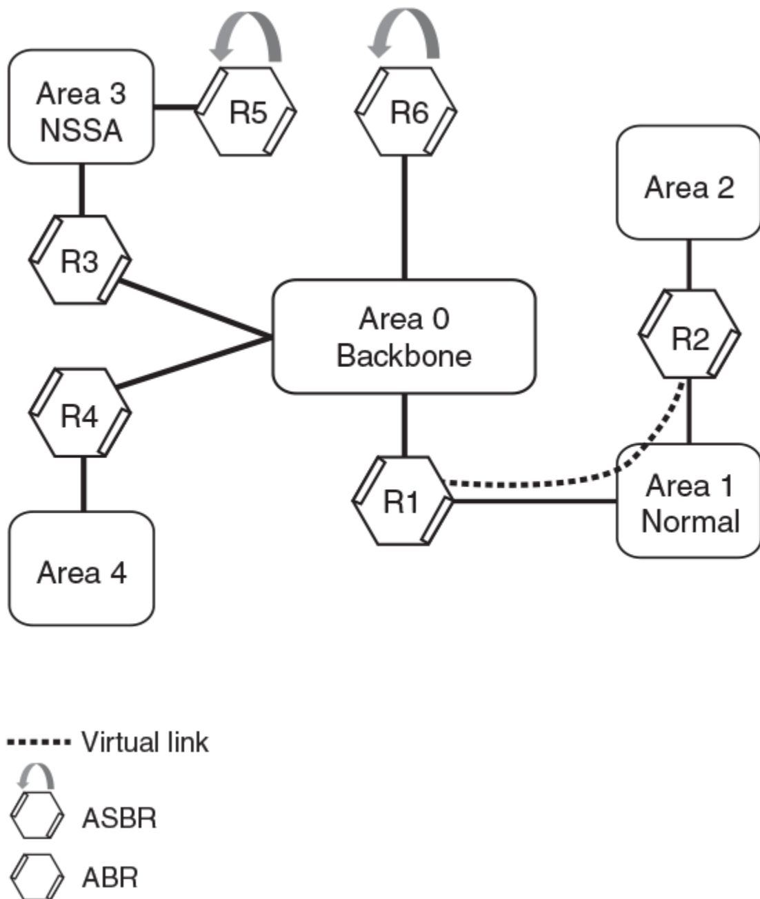
Figure 56: OSPFv3 virtual link
