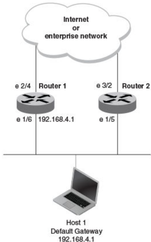
Figure 57: Single point of failure with Device 1 being the Host1 default gateway
