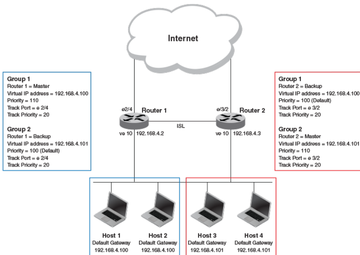
Figure 60: Two routers configured for dual redundant network access for the host
