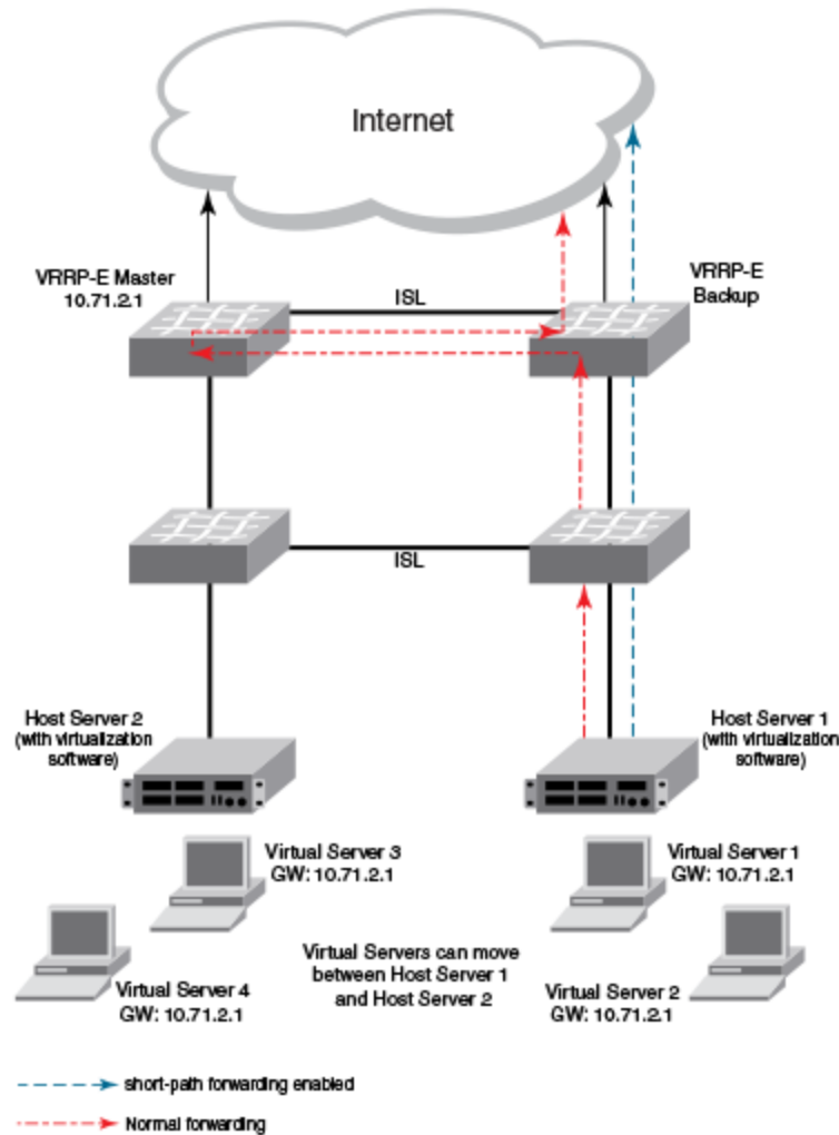
Figure 63: Short-path forwarding
