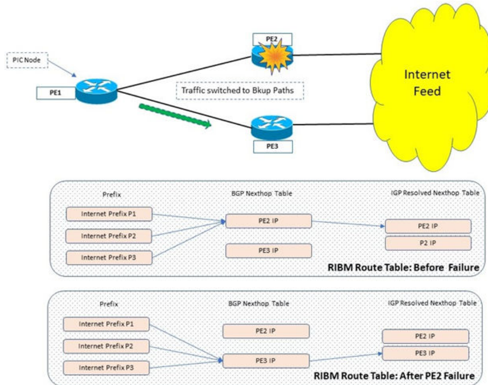
Figure 20: BGP with eBGP primary-to-backup failure
