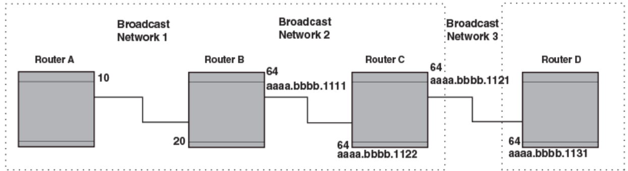
Figure 39: Each broadcast network has a Level-1 Designated IS and a Level-2 Designated IS
