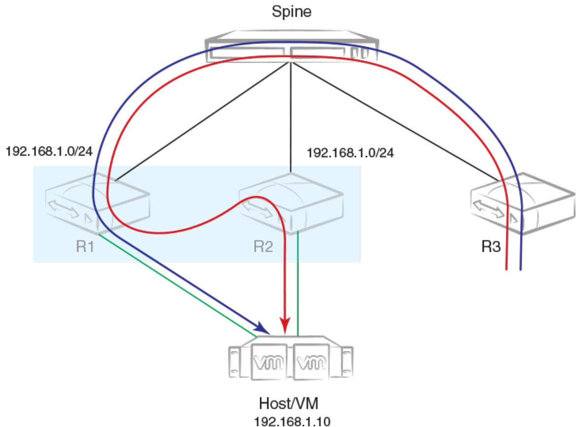
Figure 30: Avoiding traffic tromboning for EVPN Layer 3 traffic in an MCT cluster
