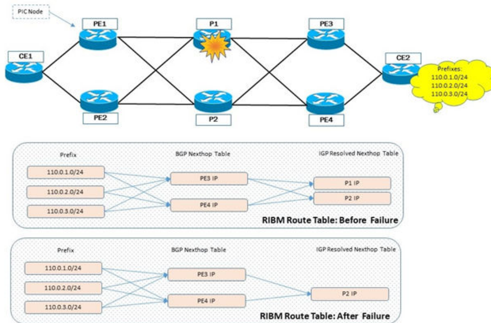
Figure 17: BGP PIC core node failure
