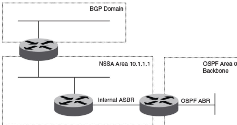
Figure 53: OSPF network containing an NSSA
