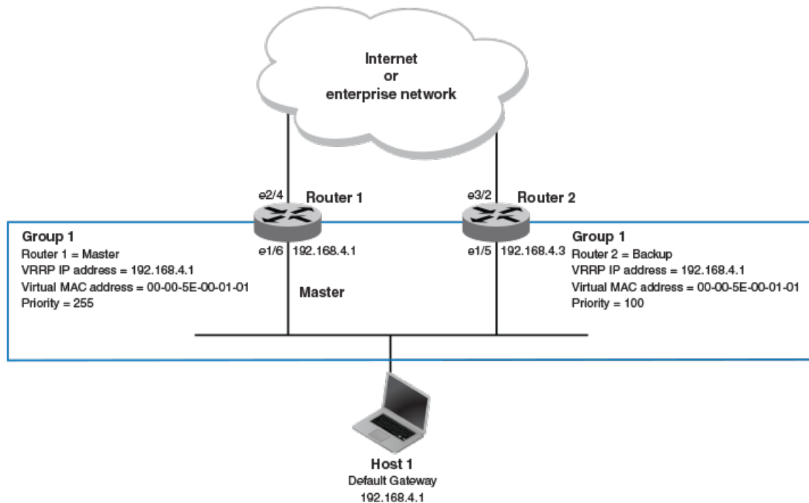
Figure 58: Devices configured as VRRP virtual routers for redundant network access for Host 1
