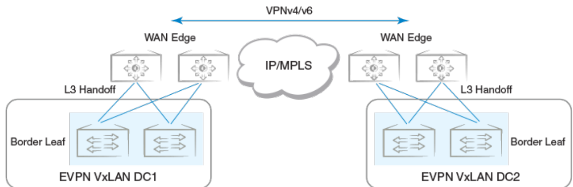
Figure 32: Layer 3 handoff-based DCI
