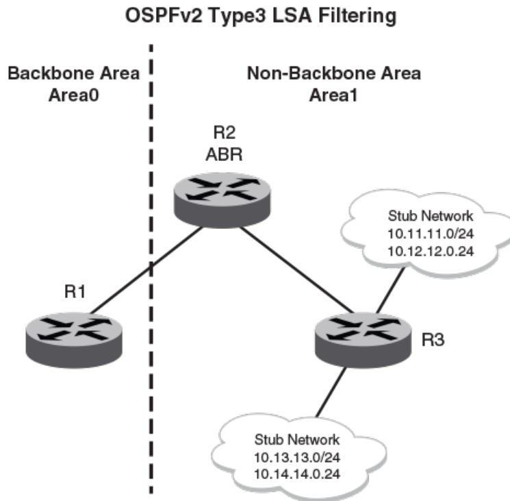
Figure 55: OSPFv2 type 3 LSA filtering
