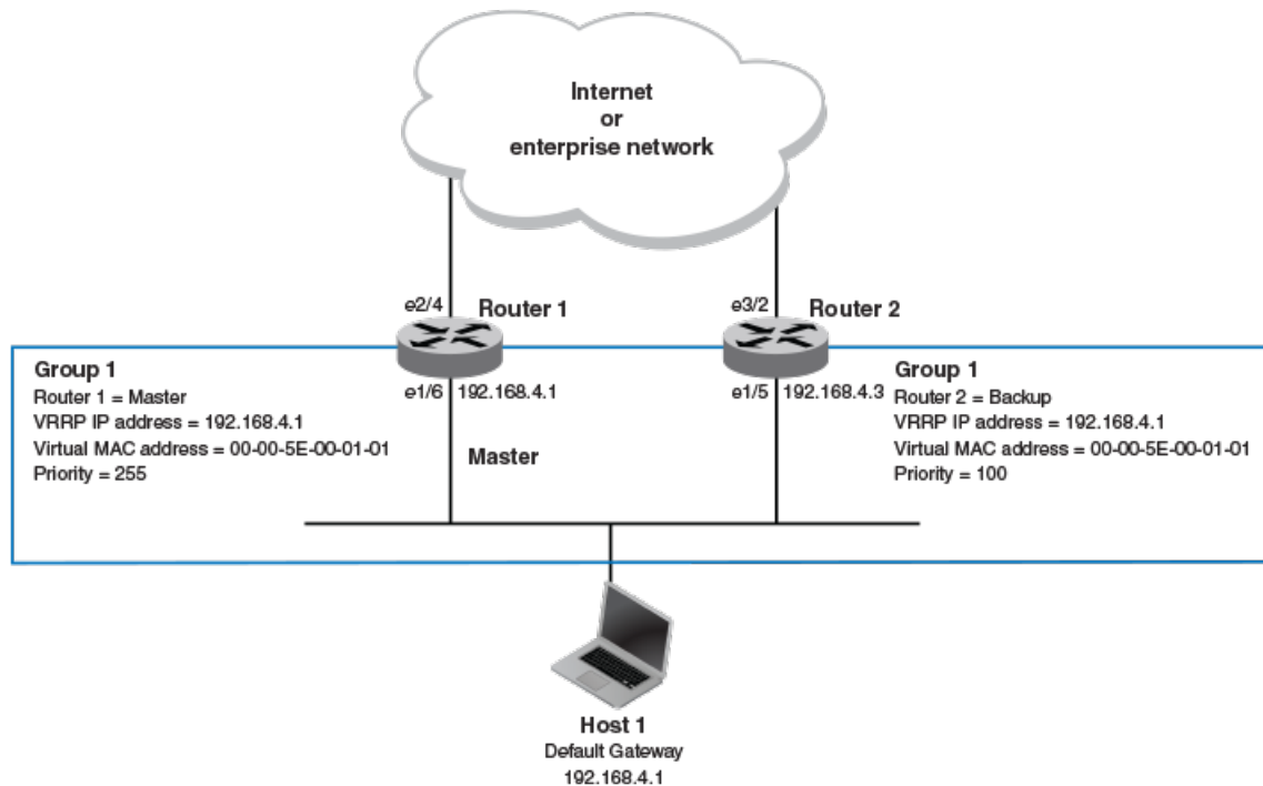
Figure 59: Basic VRRP topology
