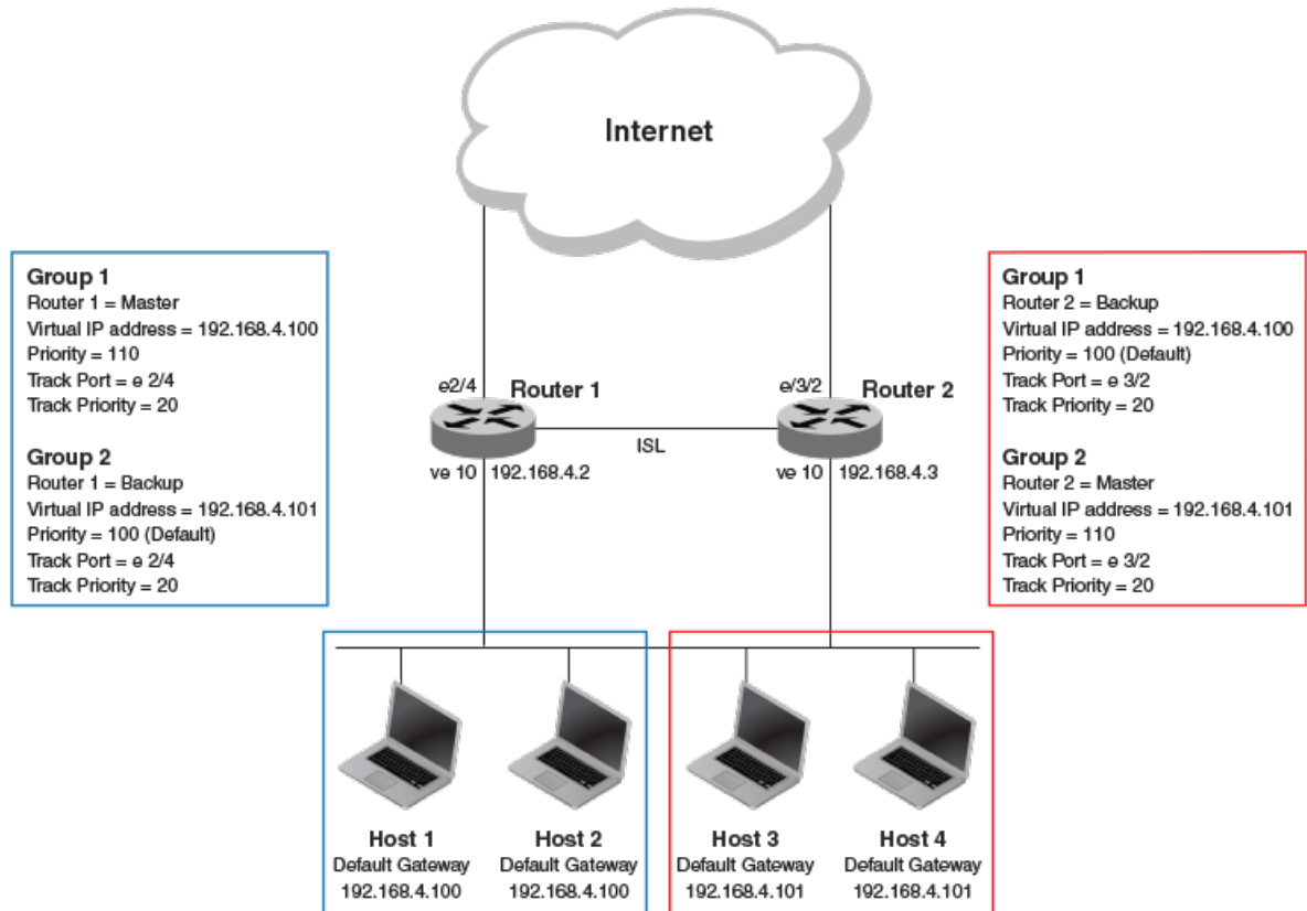
Figure 61: Multigroup VRRP routing topology
