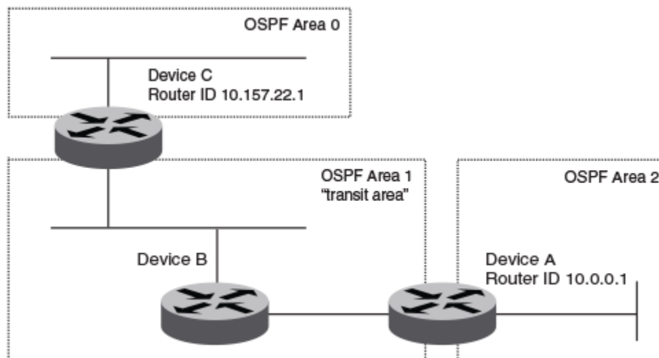
Figure 54: Defining OSPF virtual links within a network
