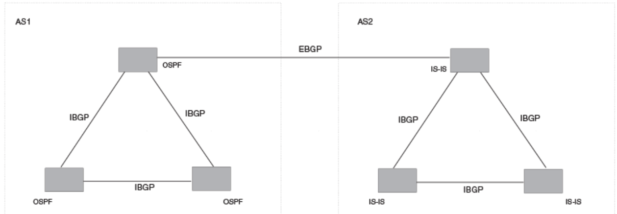
Figure 11: BGP4 autonomous systems
