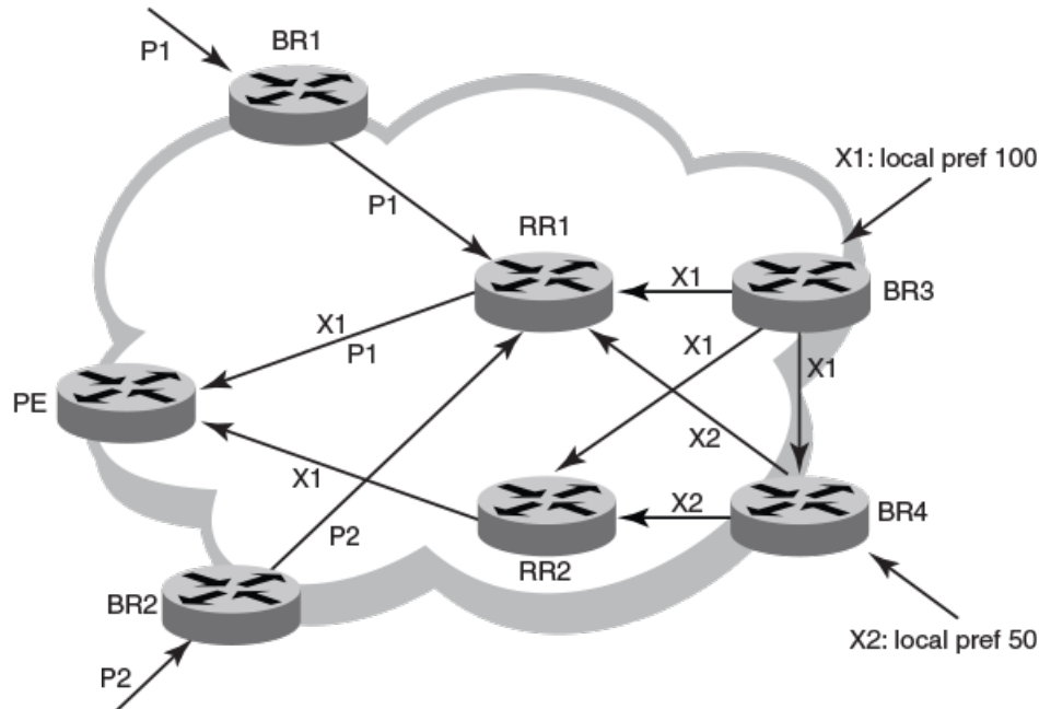
Figure 14: BGP path hiding
