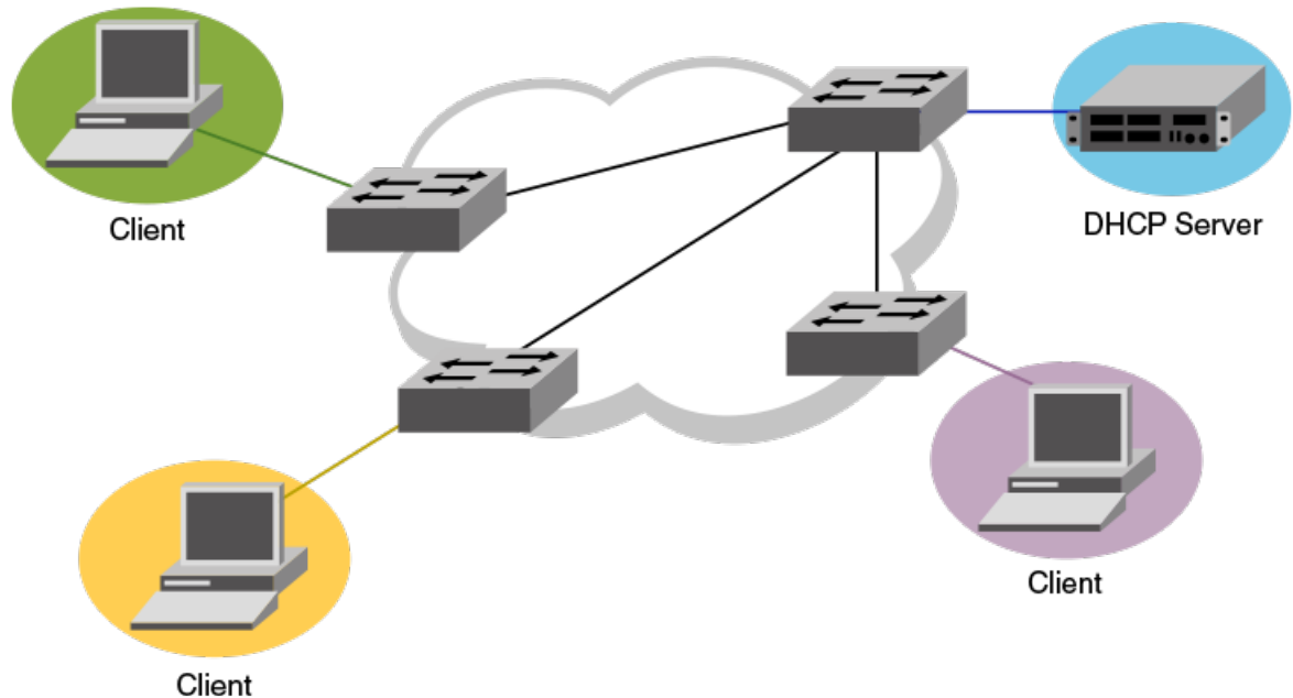
Figure 49: Inter-VRF route leaking example for connecting clients to a DHCP server in a different VRF.
