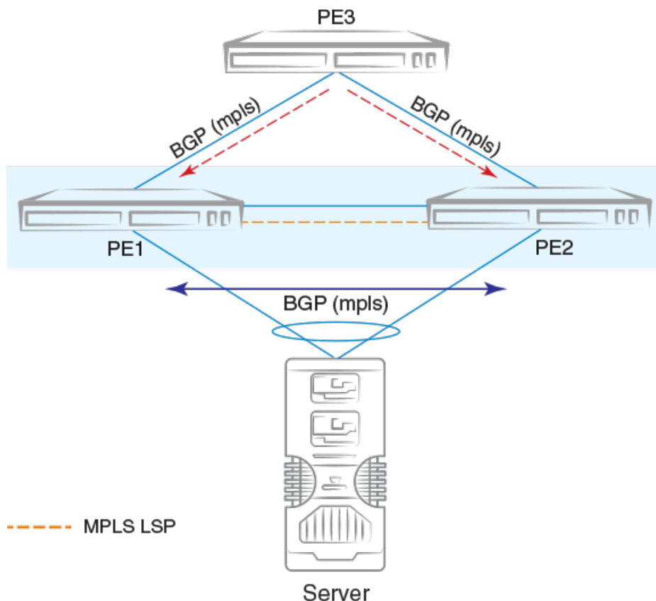
Figure 28: Aliasing in MPLS
