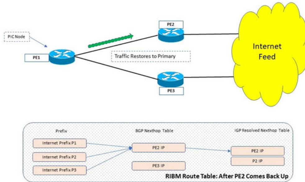
Figure 21: BGP with eBGP backup-to-primary failure
