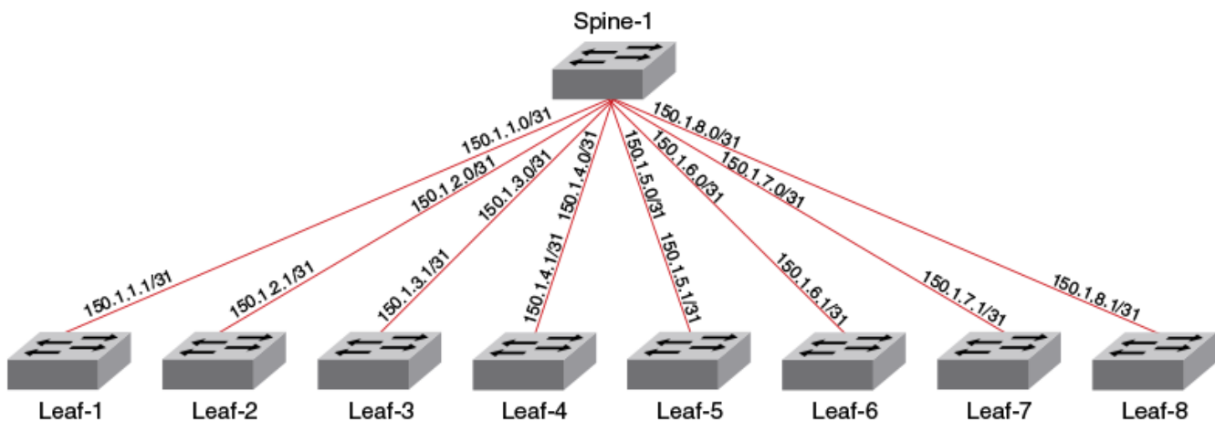
Figure 23: BGP session between spine and leaf nodes
