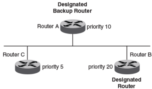
Figure 52: Designated and backup router election
