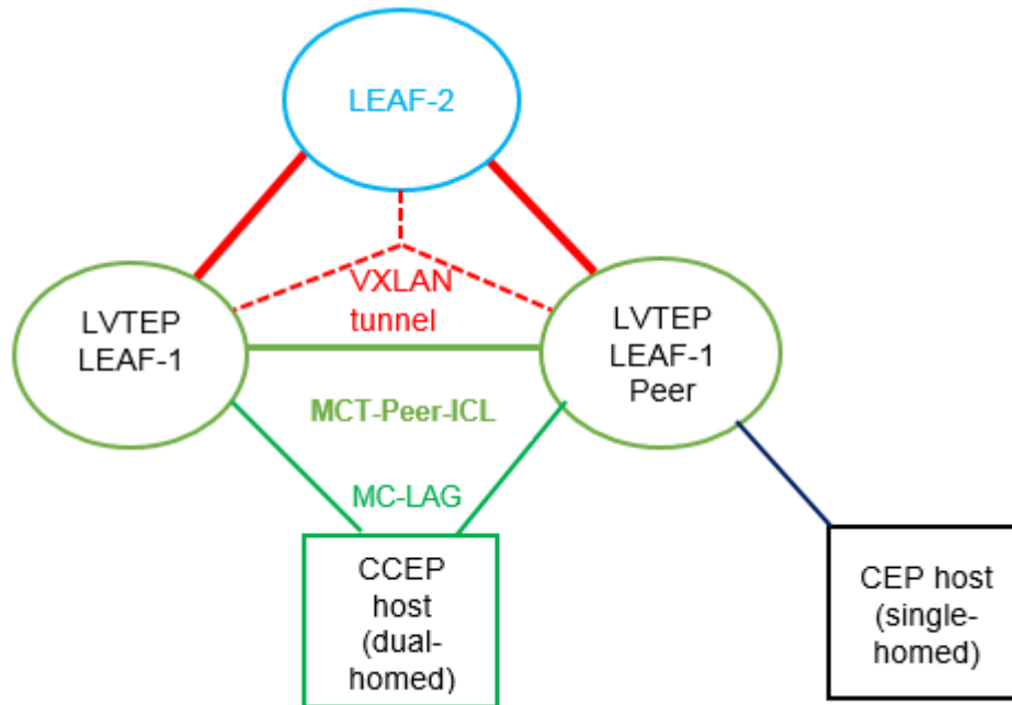
Figure 66: VXLAN LVTEP topology
