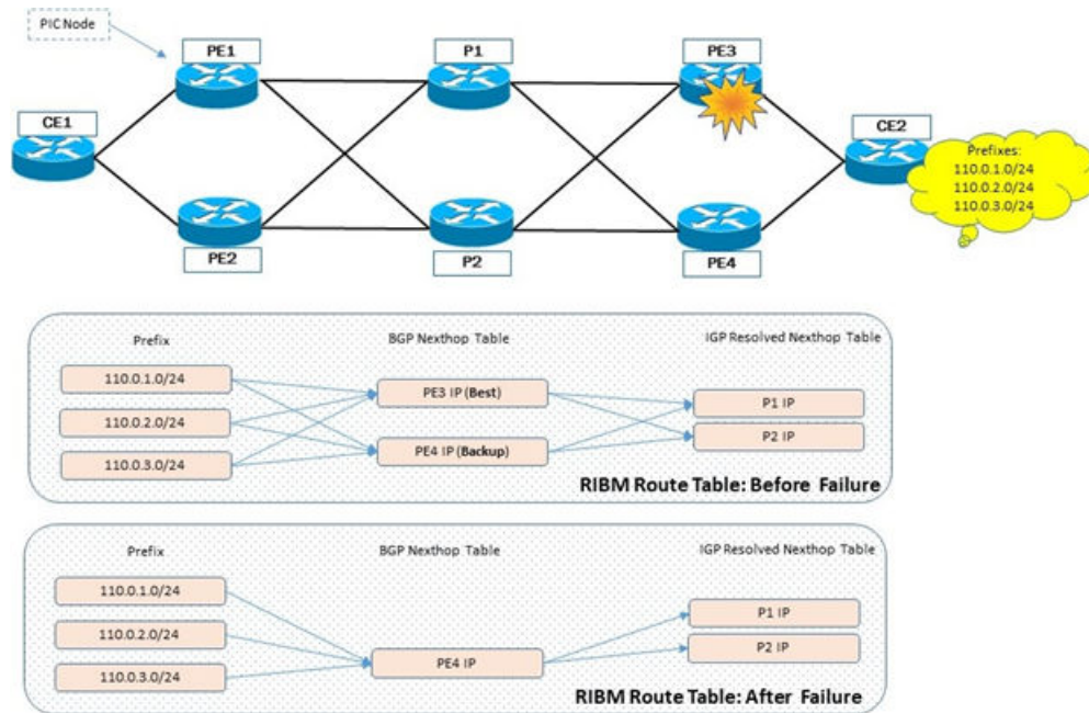
Figure 19: BGP PIC edge node failure
