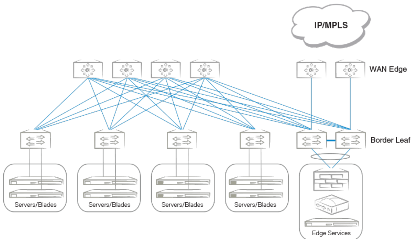
Figure 27: Border and service leaf
