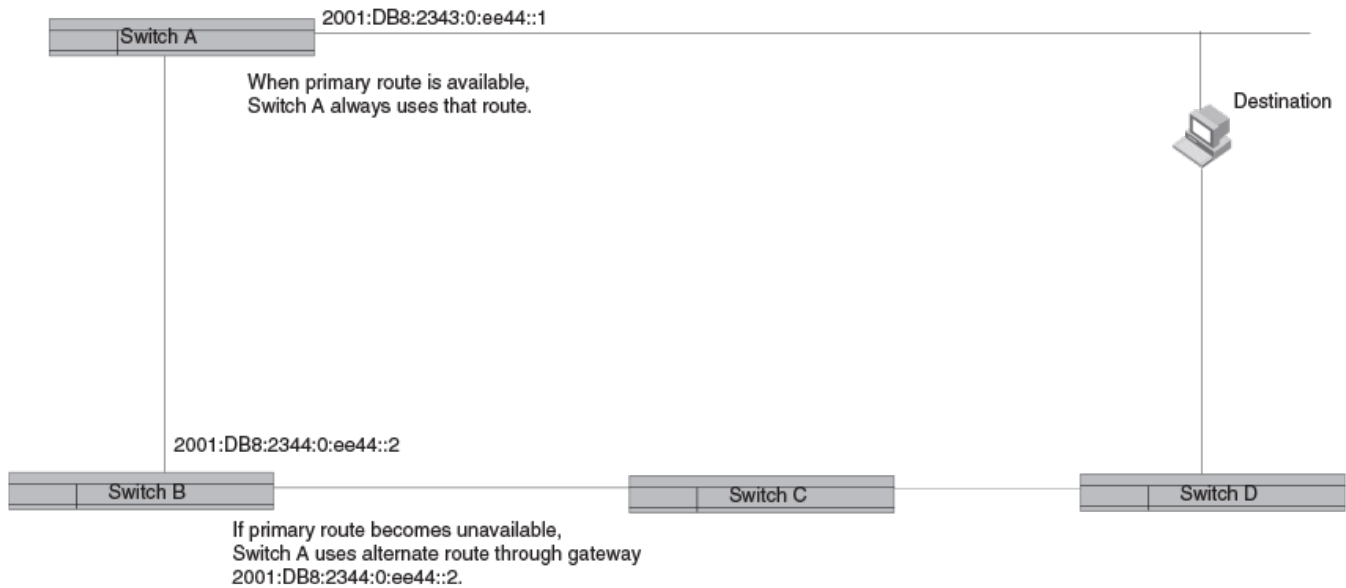
Figure 7: Two static routes to same destination
