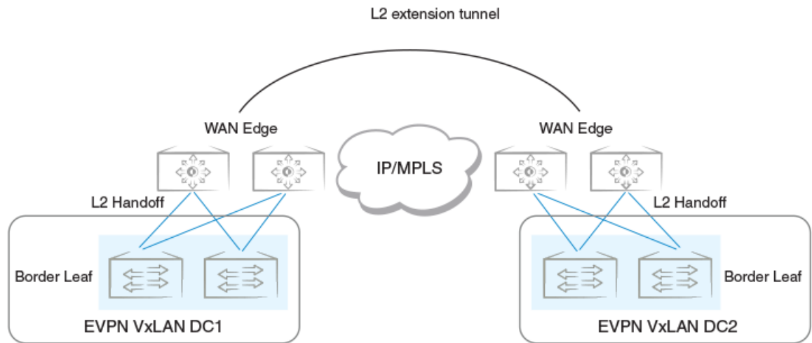
Figure 31: Layer 2 handoff-based DCI
