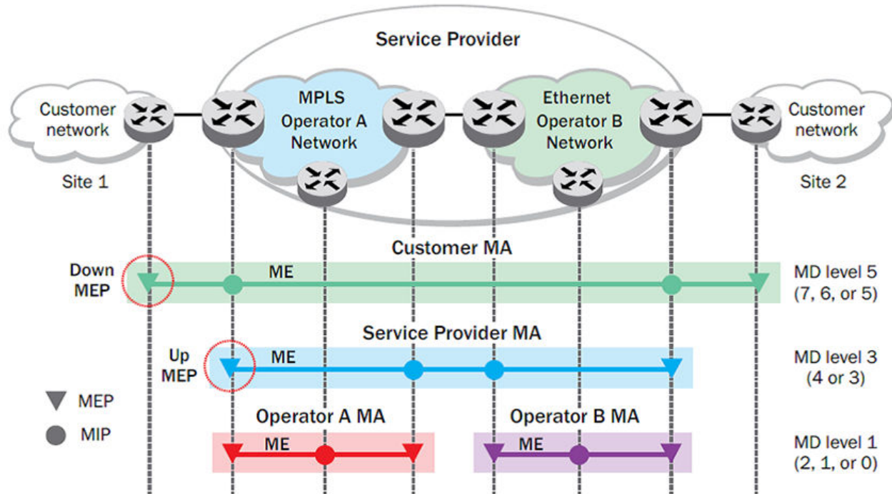
Figure 5: CFM deployment
