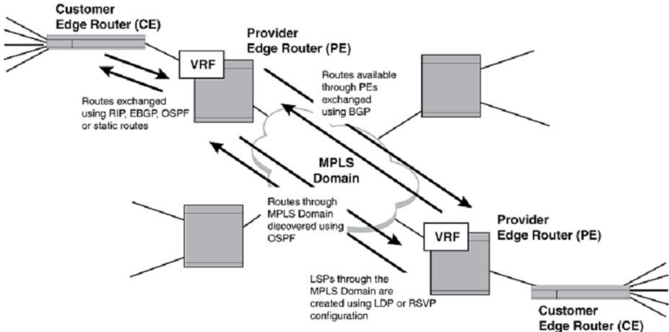
Figure 33: BGP or MPLS VPN route discovery
