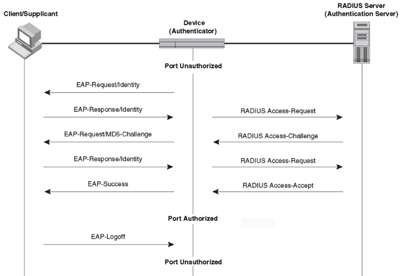
Figure 8: Message exchange between client/supplicant, authenticator, and authentication server
