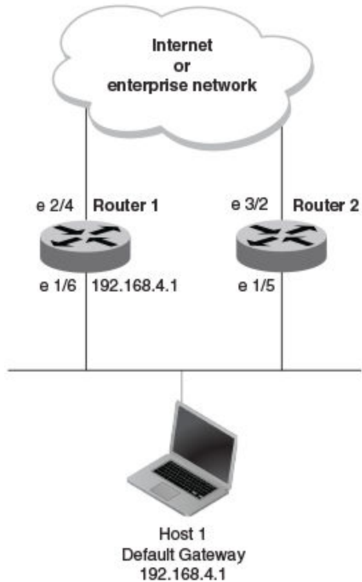
Figure 59: Single point of failure with Device 1 being the Host1 default gateway
