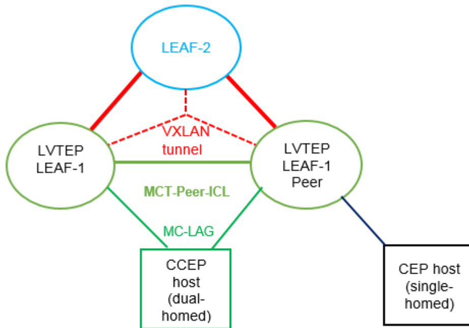
Figure 70: VXLAN LVTEP topology
