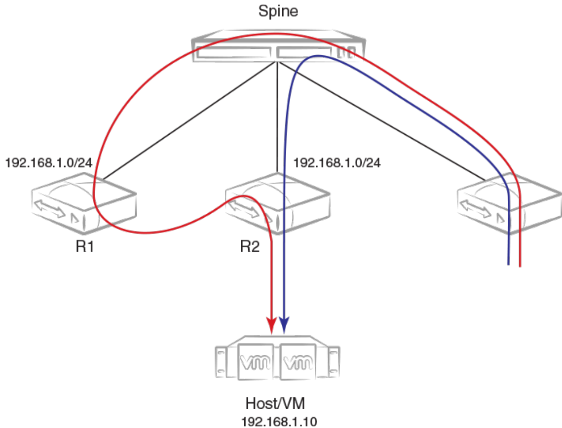
Figure 30: Avoiding suboptimal paths by converting MACIP routes to host routes
