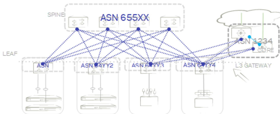
Figure 27: eBGP spine and leaf Border and service leaf
