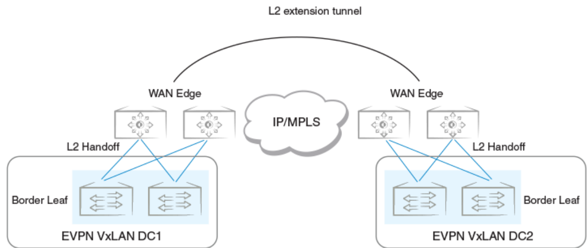
Figure 32: Layer 2 handoff-based DCI
