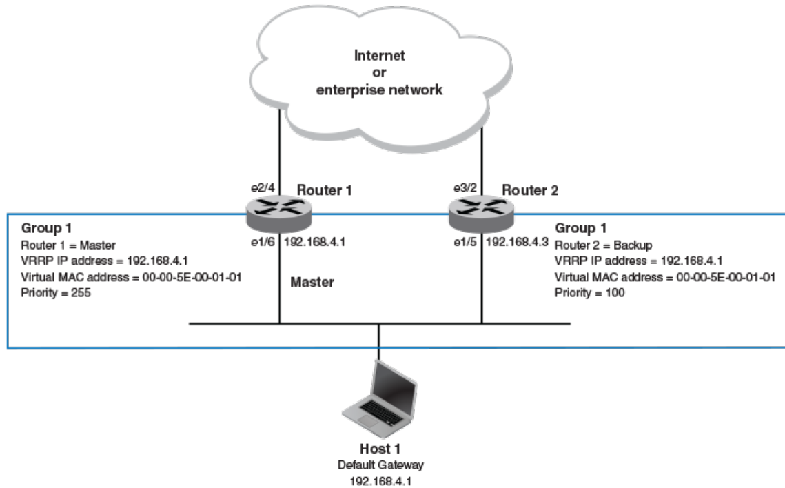
Figure 62: Devices configured as VRRP virtual routers for redundant network access for Host 1
