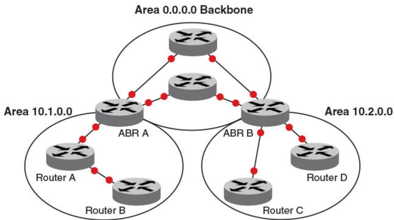
Figure 55: OSPF operating in a network
