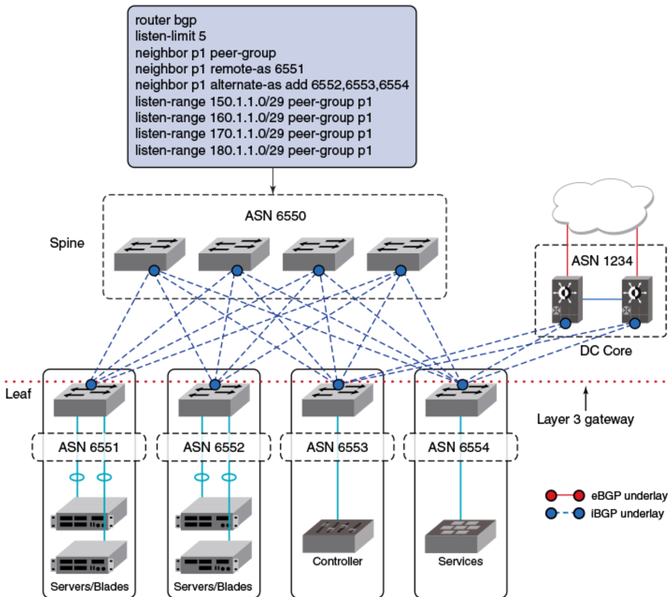
Figure 25: Minimum configuration at the spine level for BGP dynamic neighbors
