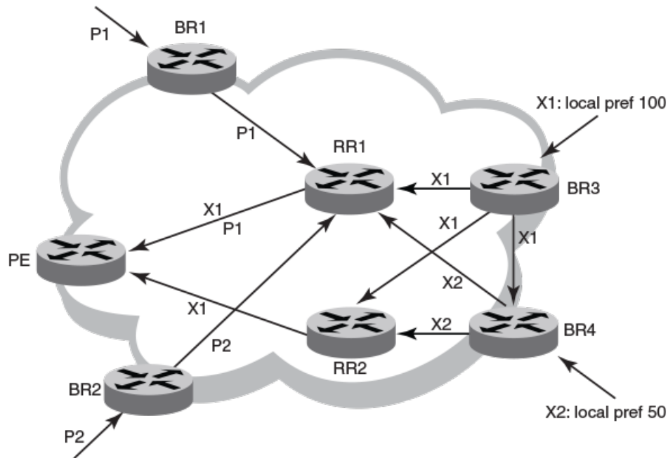
Figure 14: BGP path hiding
