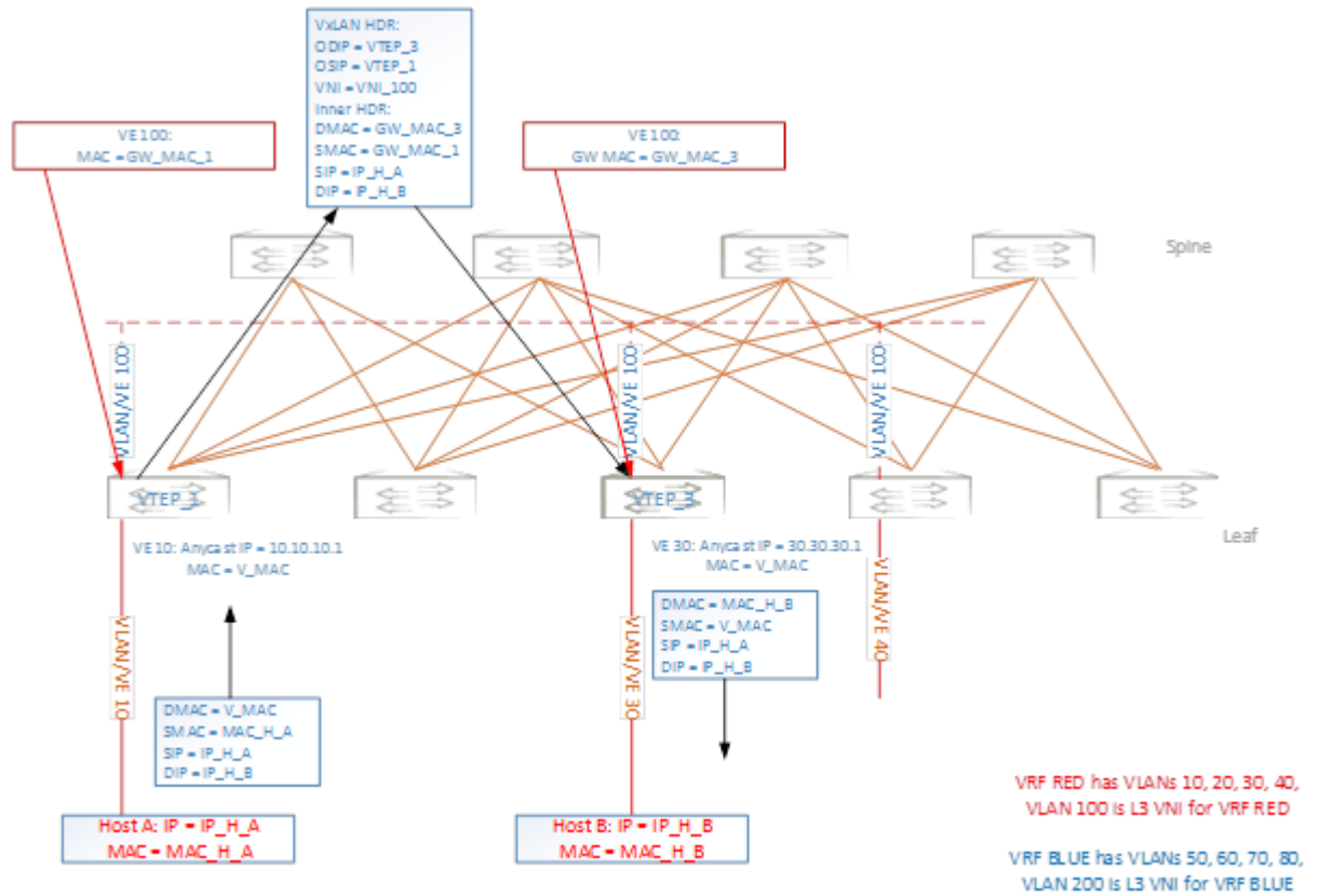
Figure 69: Layer 3 VNI on a single VTEP
