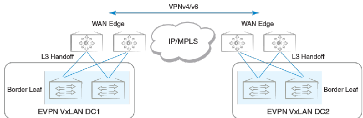
Figure 33: Layer 3 handoff-based DCI
