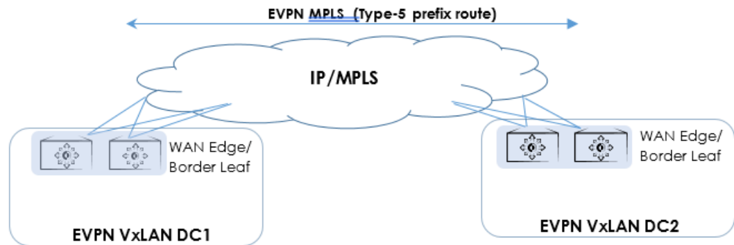
Figure 34: EVPN Type-5 prefix route termination and reorigination on the WAN edge
