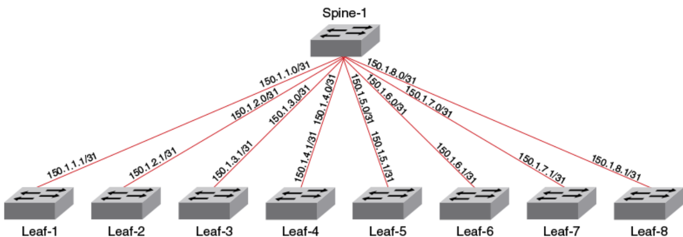
Figure 24: BGP session between spine and leaf nodes
