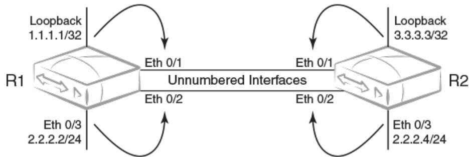
Figure 37: IP unnumbered and donor interfaces
