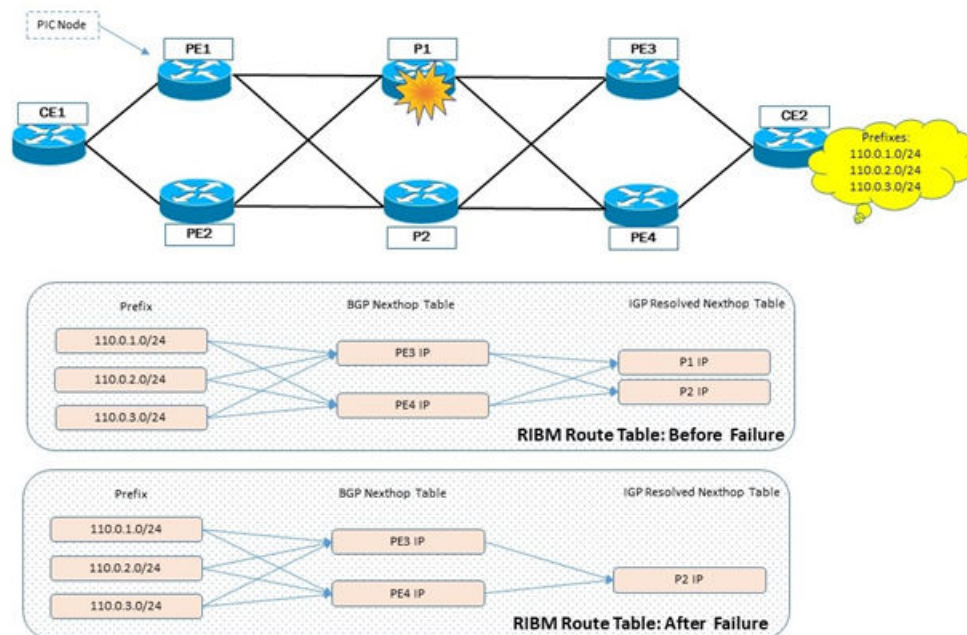
Figure 17: BGP PIC core node failure
