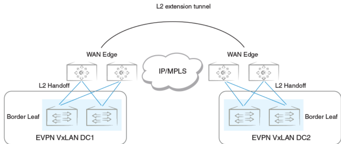
Figure 32: Layer 2 handoff-based DCI
