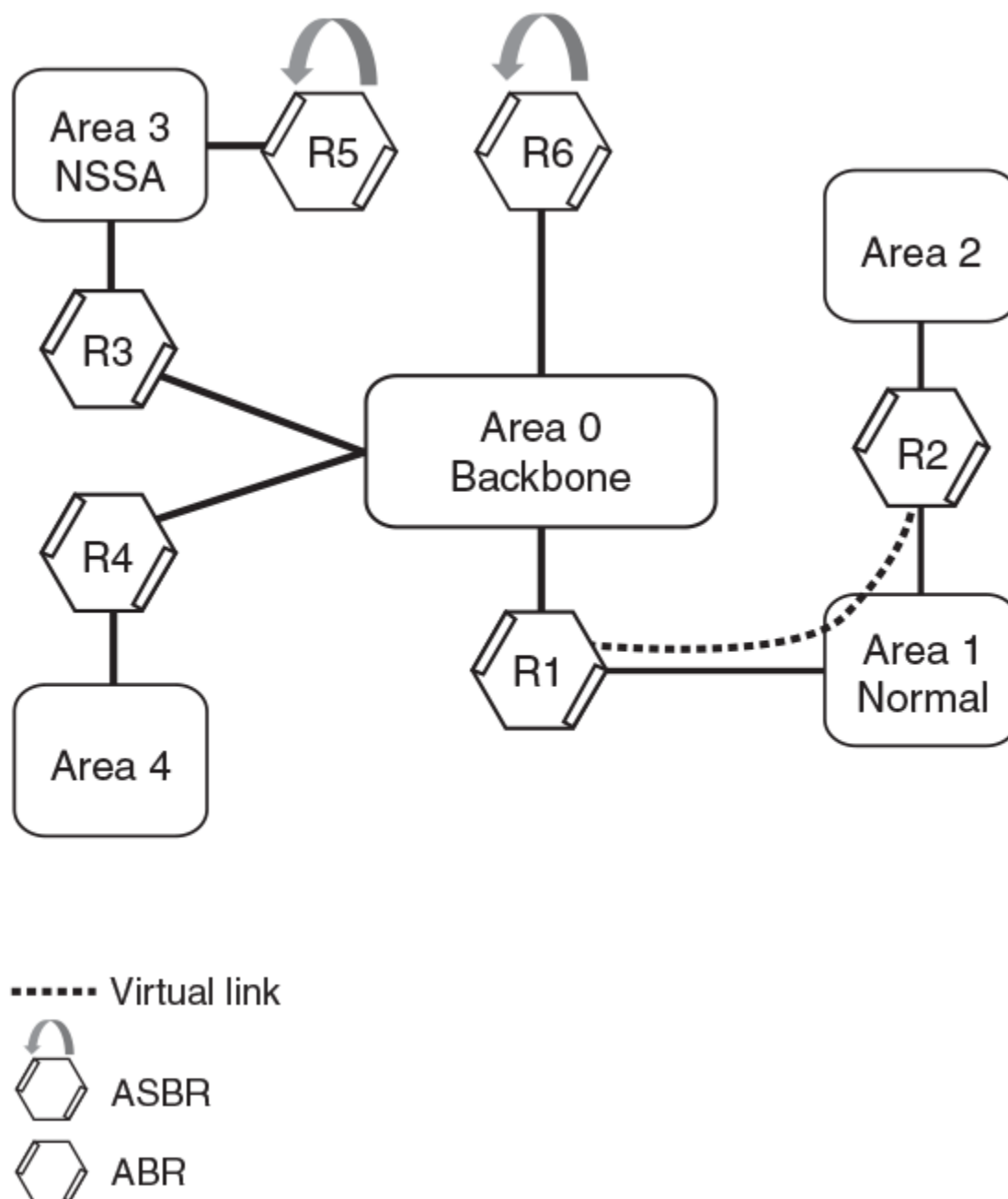
Figure 60: OSPFv3 virtual link
