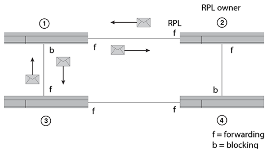
Figure 39: Initializing an ERP topology - II
