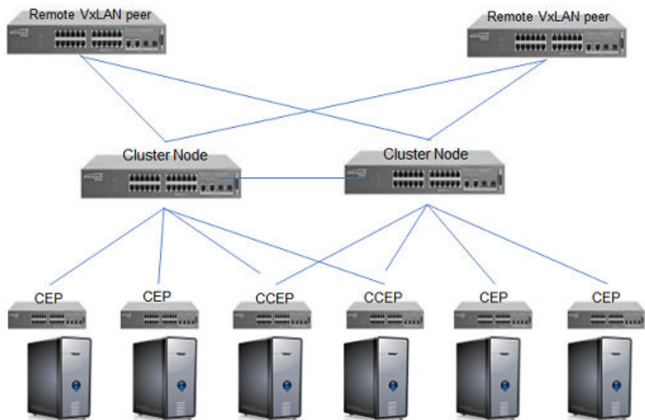
Figure 2: LVTEP topology
