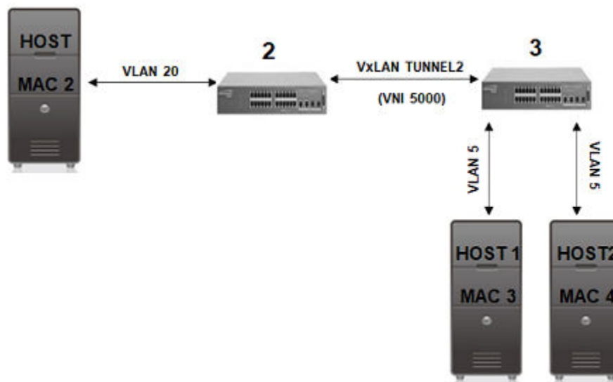
Figure 1: Layer 2 gateway topology
