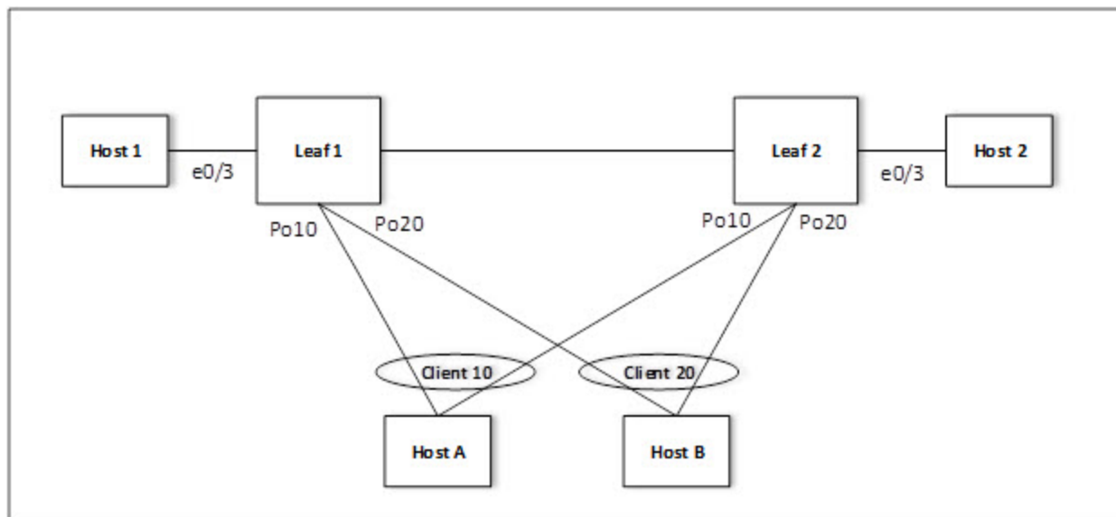
Figure 5: MCT data plane topology example
