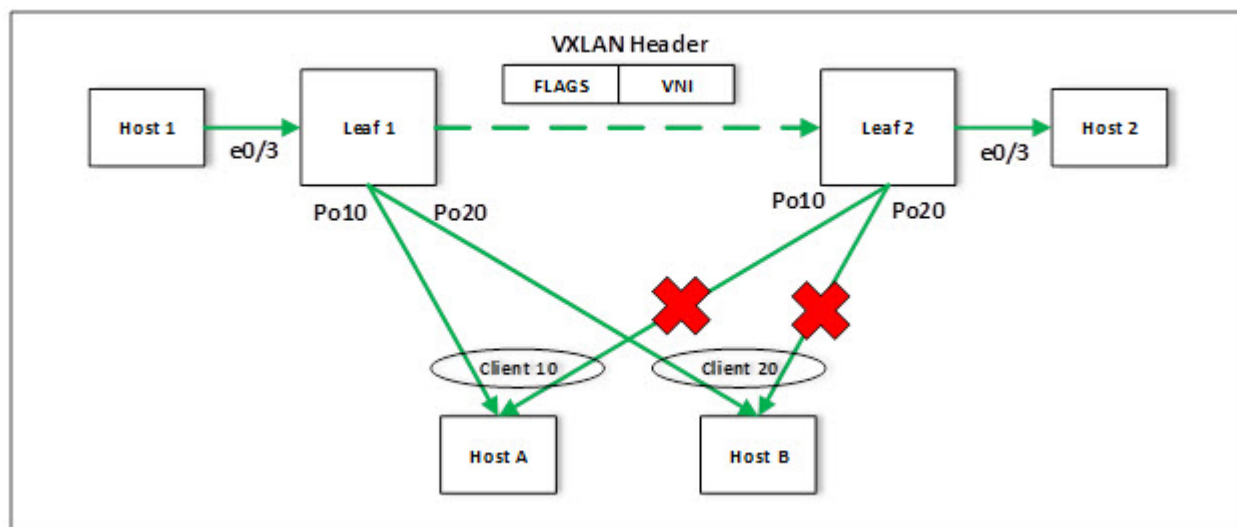
Figure 9: BUM forwarding between cluster edge ports
