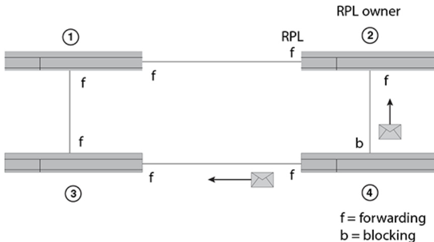
Figure 38: Initializing an ERN topology - I
