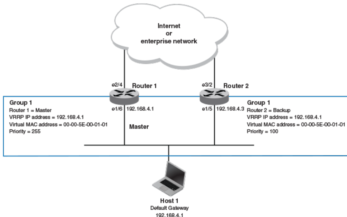
Figure 63: Devices configured as VRRP virtual routers for redundant network access for Host 1
