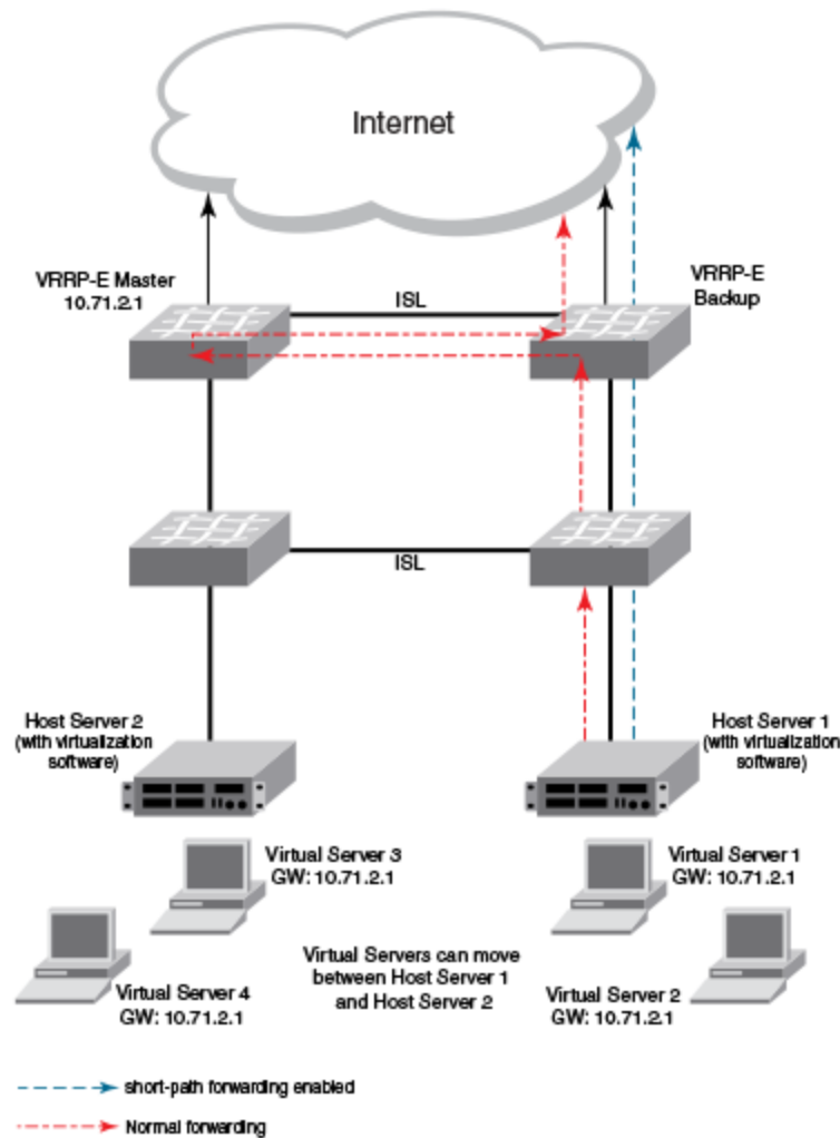
Figure 67: Short-path forwarding
