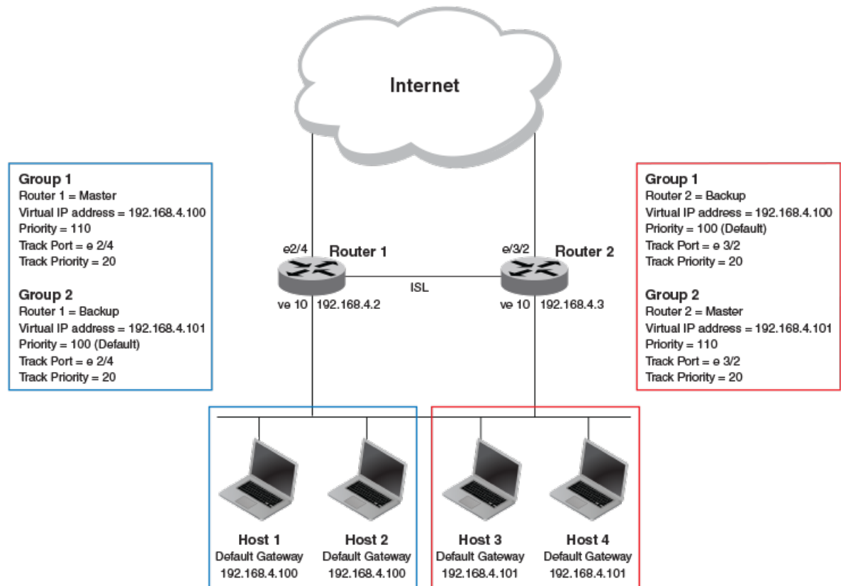
Figure 65: Two routers configured for dual redundant network access for the host
