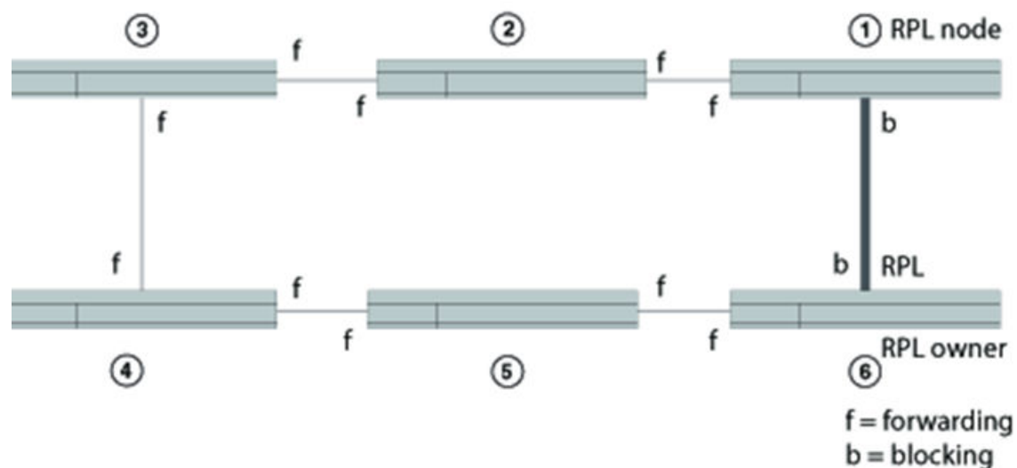
Figure 45: ERP topology
