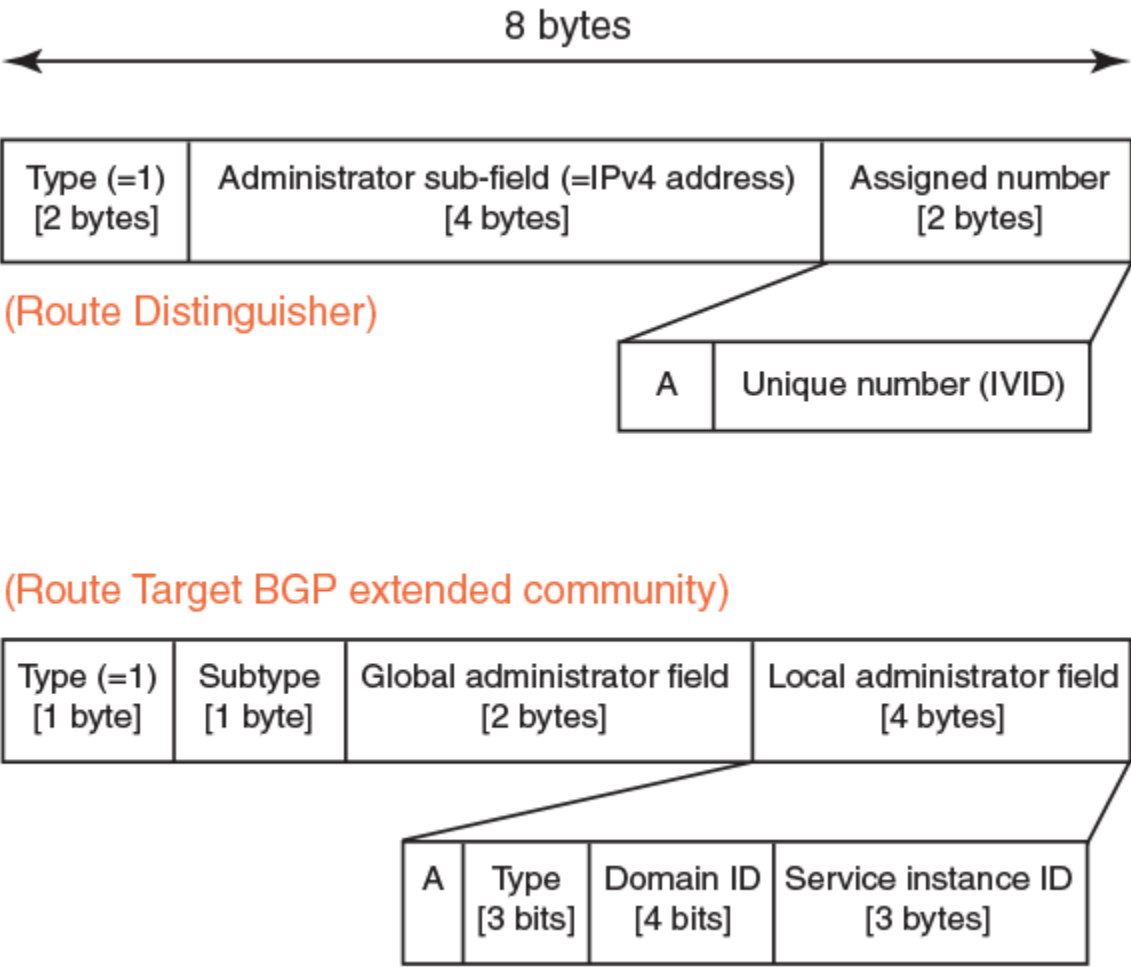
Figure 24: RD and RT formats
