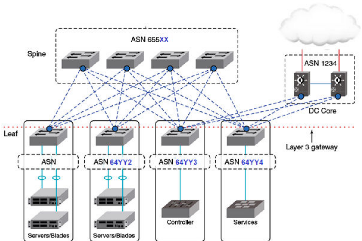
Figure 28: eBGP spine and leaf
