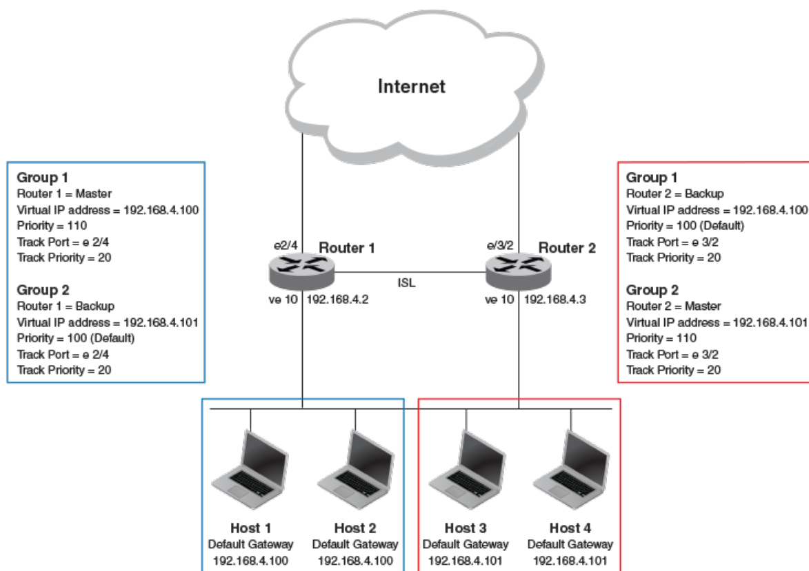
Figure 67: Multigroup VRRP routing topology
