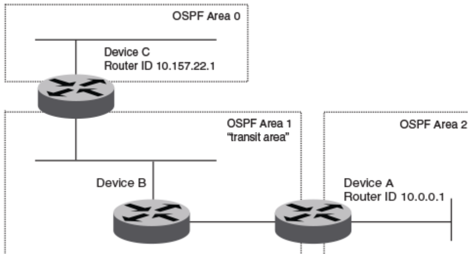
Figure 59: Defining OSPF virtual links within a network
