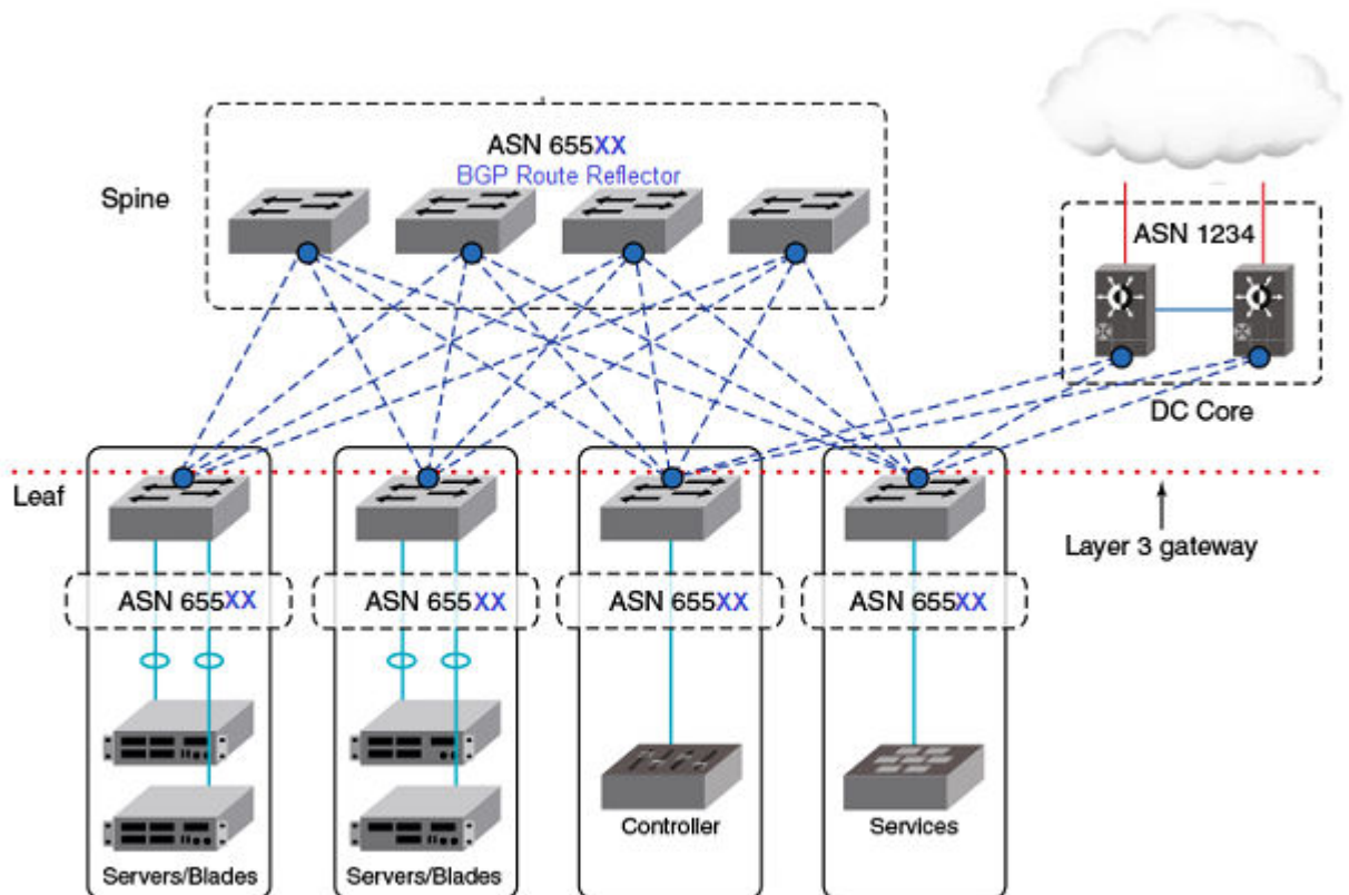
Figure 27: iBGP spine and leaf
