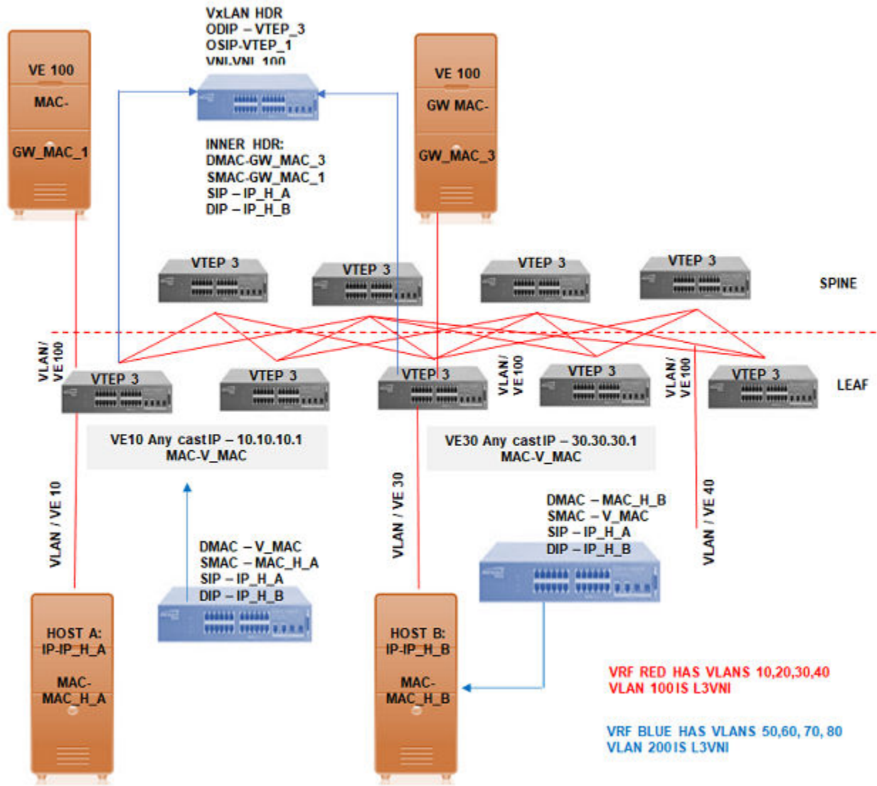
Figure 71: Layer 3 VNI on a single VTEP
