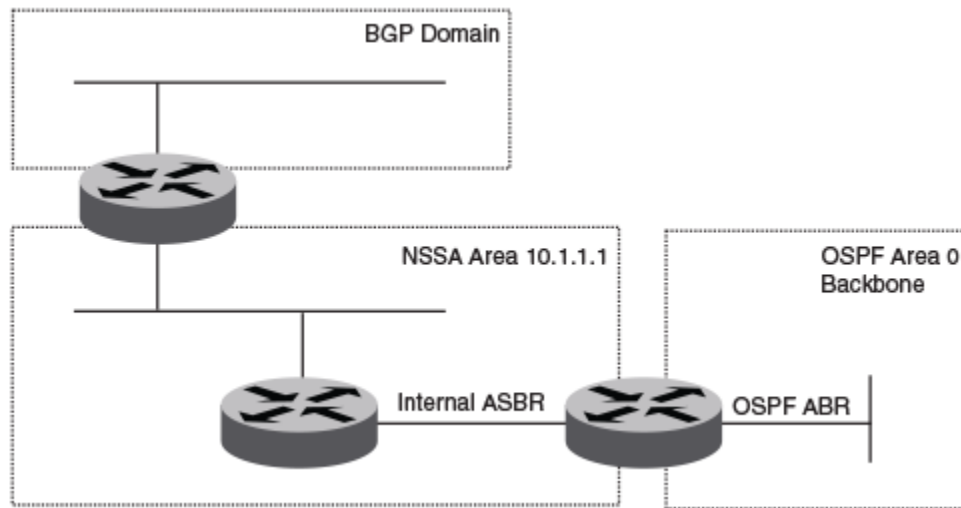
Figure 58: OSPF network containing an NSSA
