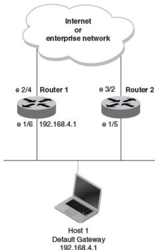
Figure 63: Single point of failure with Device 1 being the Host1 default gateway
