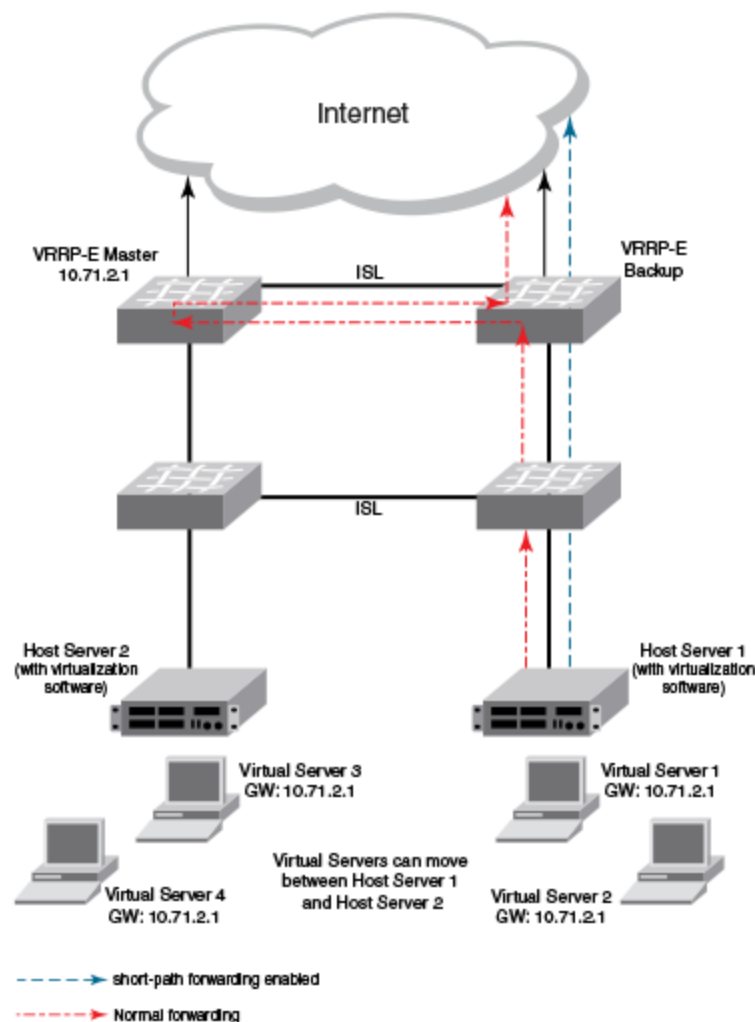
Figure 69: Short-path forwarding
