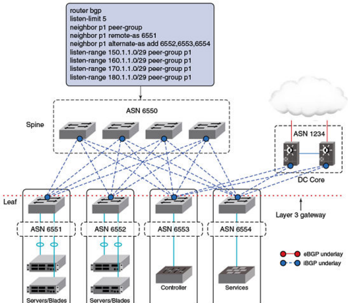
Figure 26: Minimum configuration at the spine level for BGP dynamic neighbors
