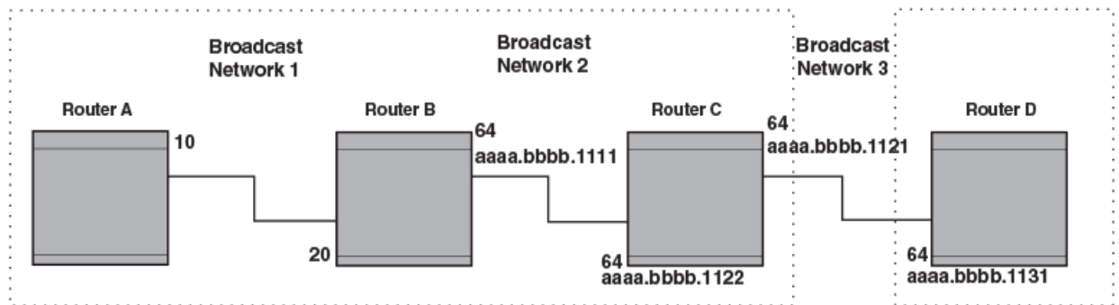
Figure 44: Each broadcast network has a Level-1 Designated IS and a Level-2 Designated IS
