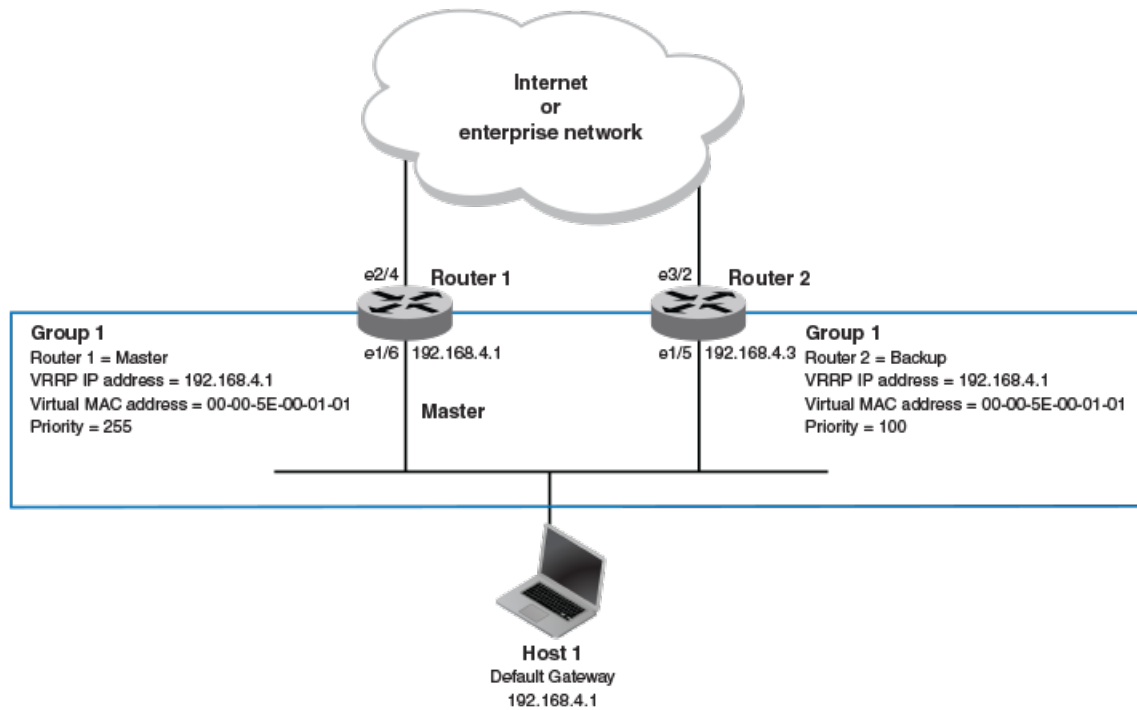
Figure 65: Basic VRRP topology
