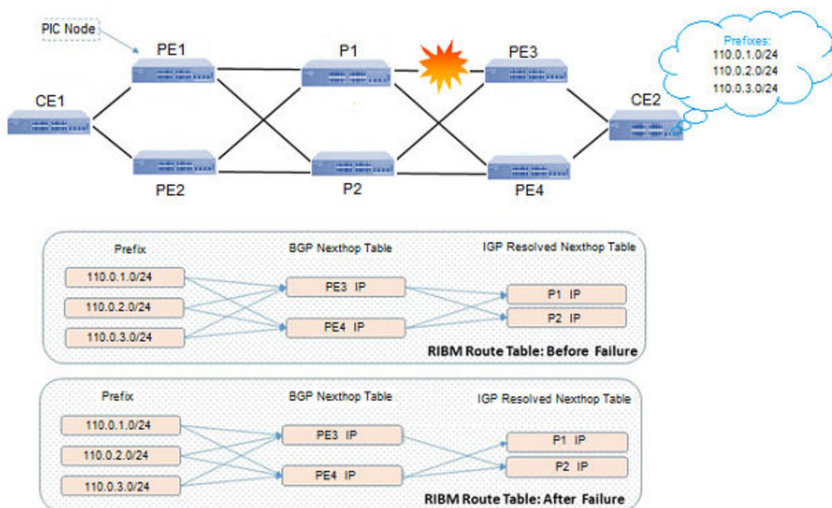
Figure 18: BGP PIC core node failure
