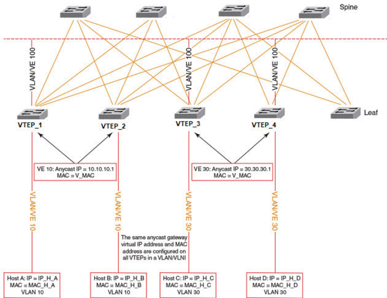
Figure 37: Static anycast gateway
