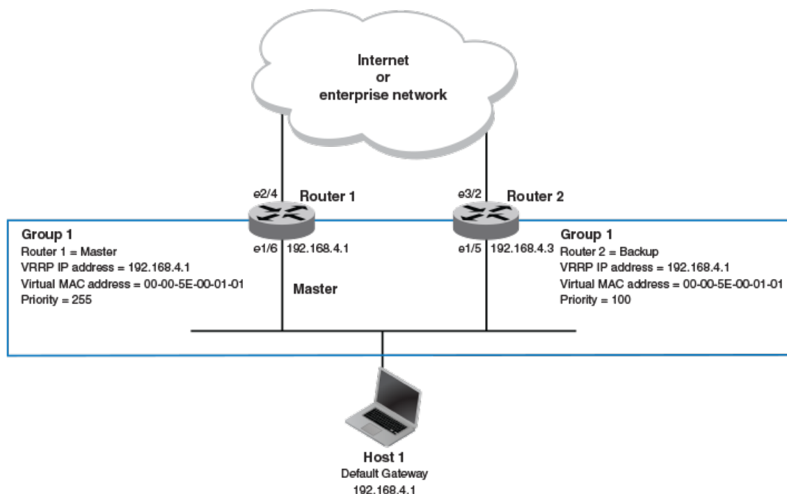
Figure 64: Devices configured as VRRP virtual routers for redundant network access for Host 1
