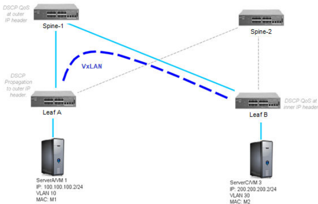
Figure 74: VxLAN L3 gateway support of intersubnet communication
