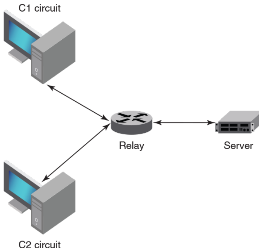
Figure 40: IP DHCP relay function
