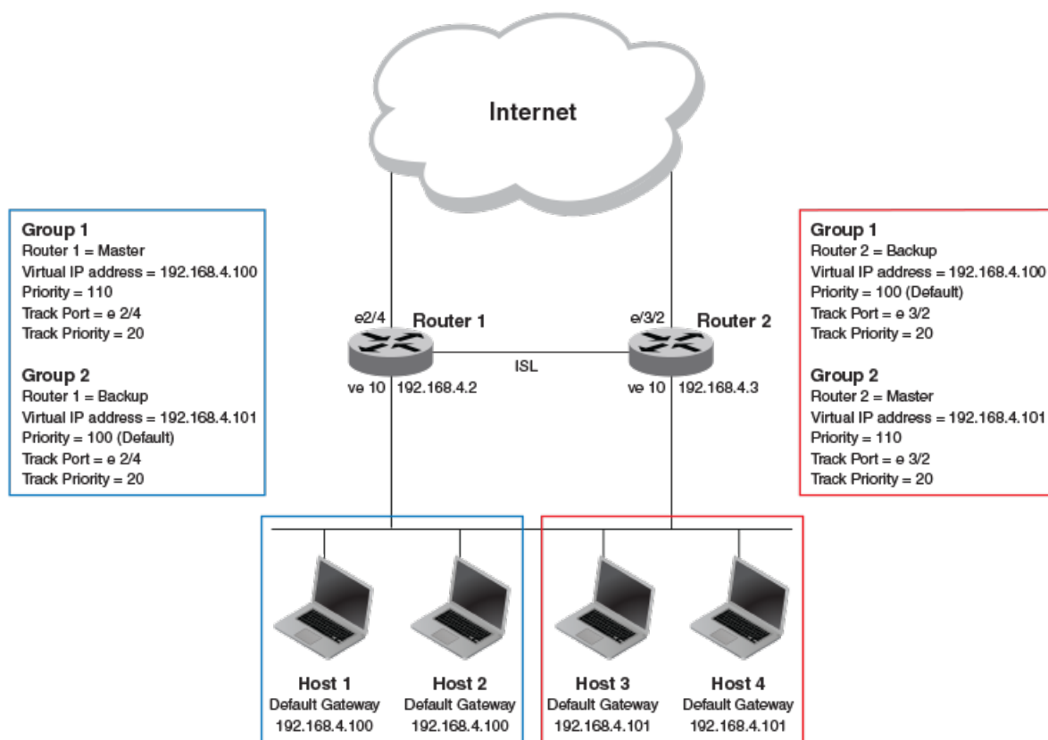
Figure 66: Two routers configured for dual redundant network access for the host
