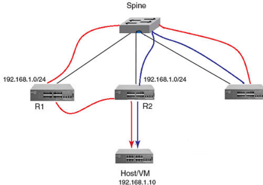
Figure 31: Avoiding suboptimal paths by converting MACIP routes to host routes
