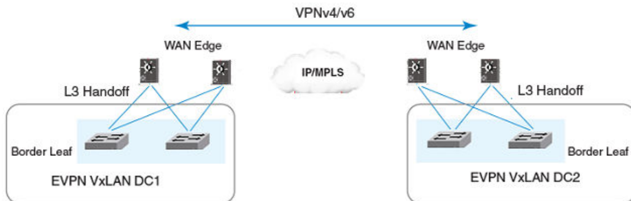
Figure 34: Layer 3 handoff-based DCI
