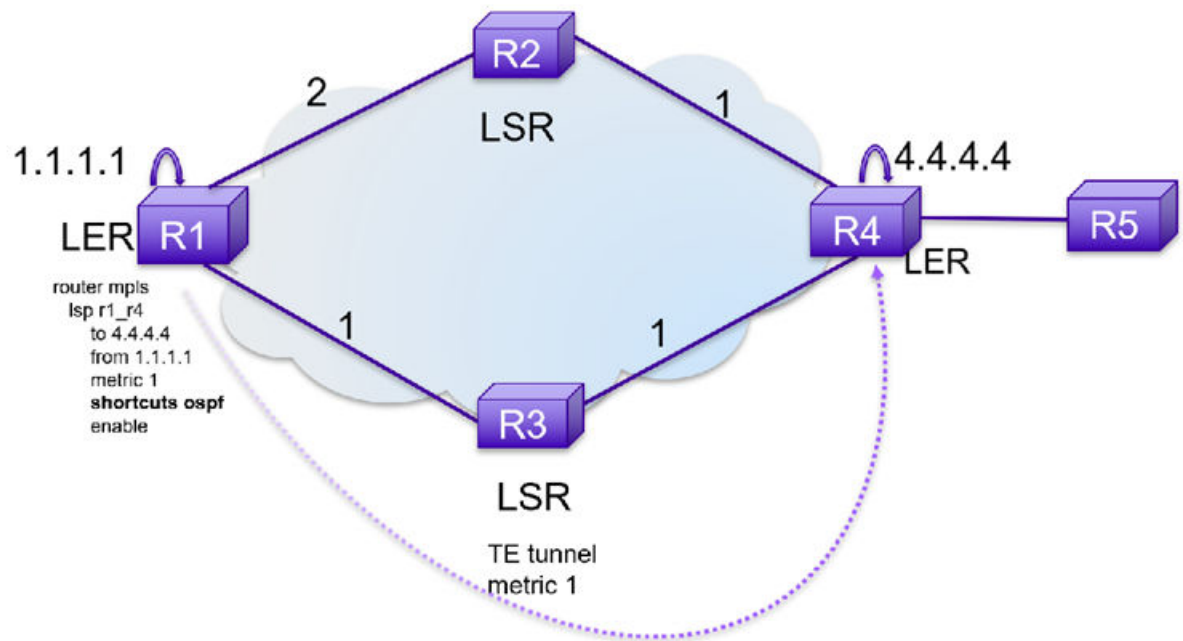
Figure 61: OSPF Shortcuts
