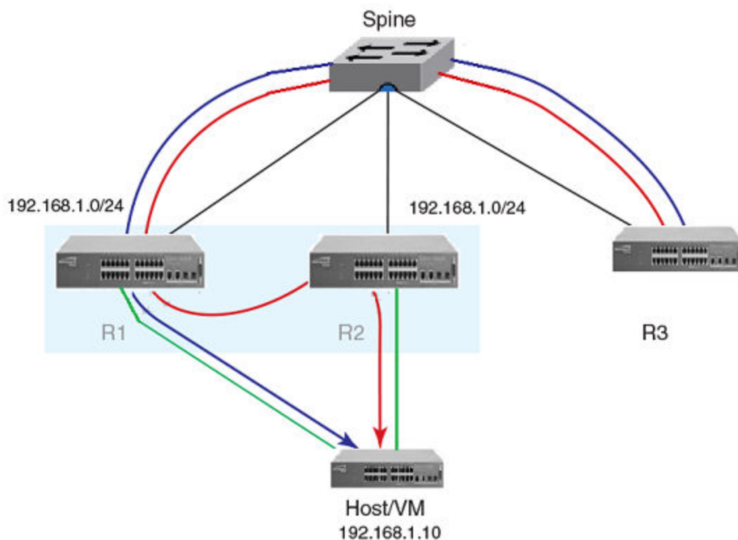
Figure 32: Avoiding traffic tromboning for EVPN Layer 3 traffic in an MCT cluster
