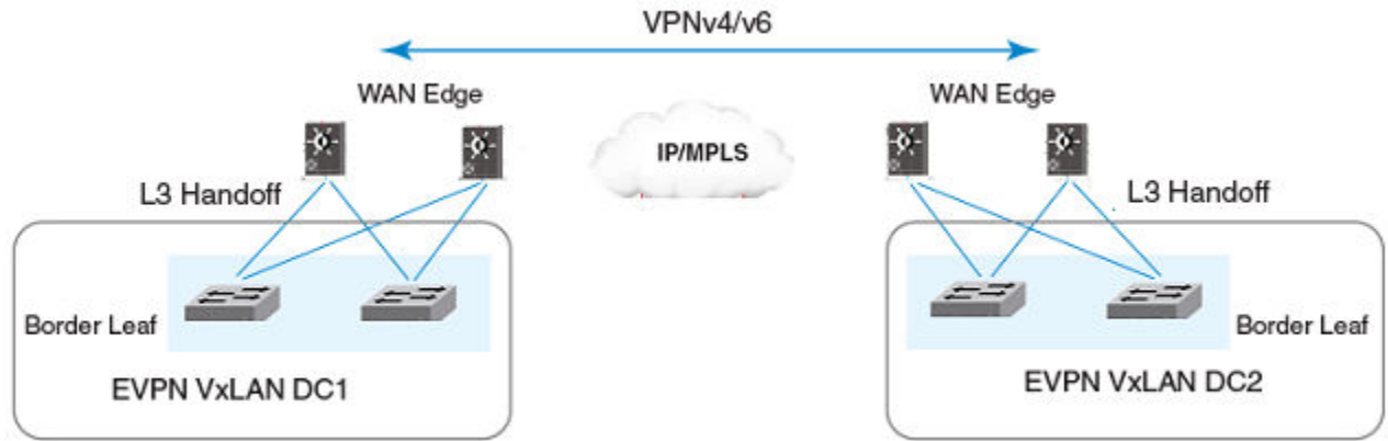
Figure 36: Layer 3 handoff-based DCI
