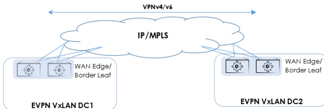
Figure 38: Data center Layer 3 interconnect with EVPN VxLAN and VPNv4/v6
