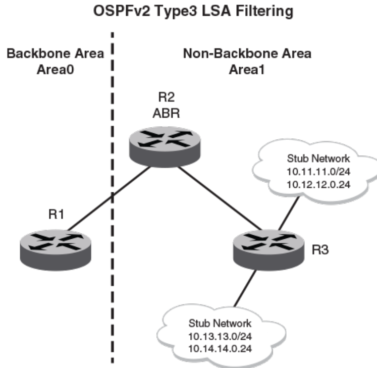
Figure 66: OSPFv2 type 3 LSA filtering
