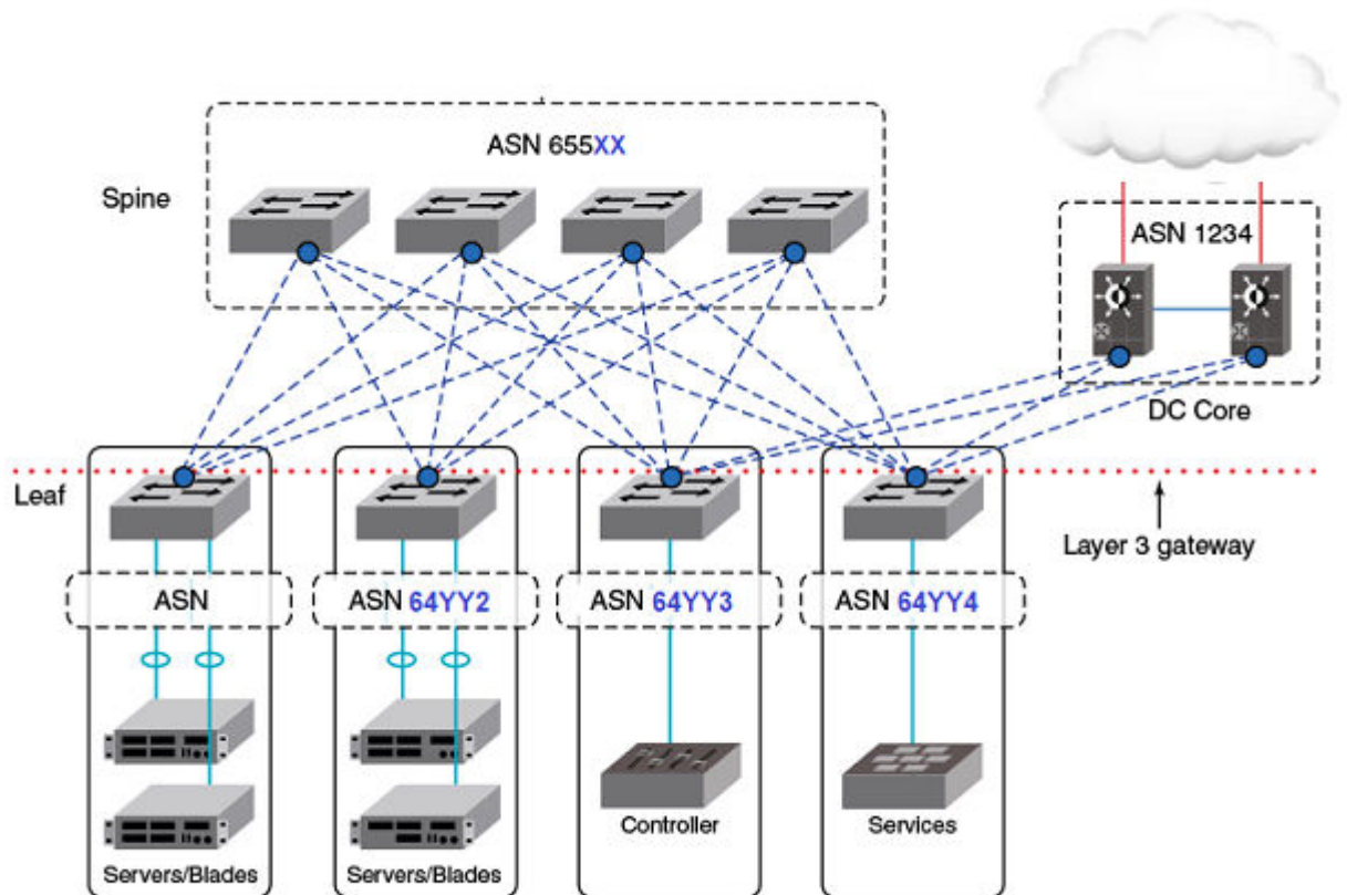
Figure 30: eBGP spine and leaf
