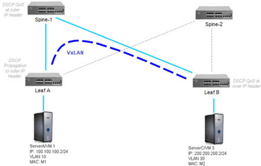
Figure 80: VxLAN L3 gateway support of intersubnet communication
