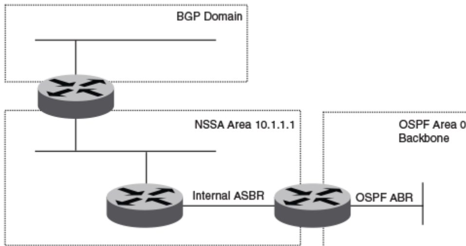
Figure 64: OSPF network containing an NSSA
