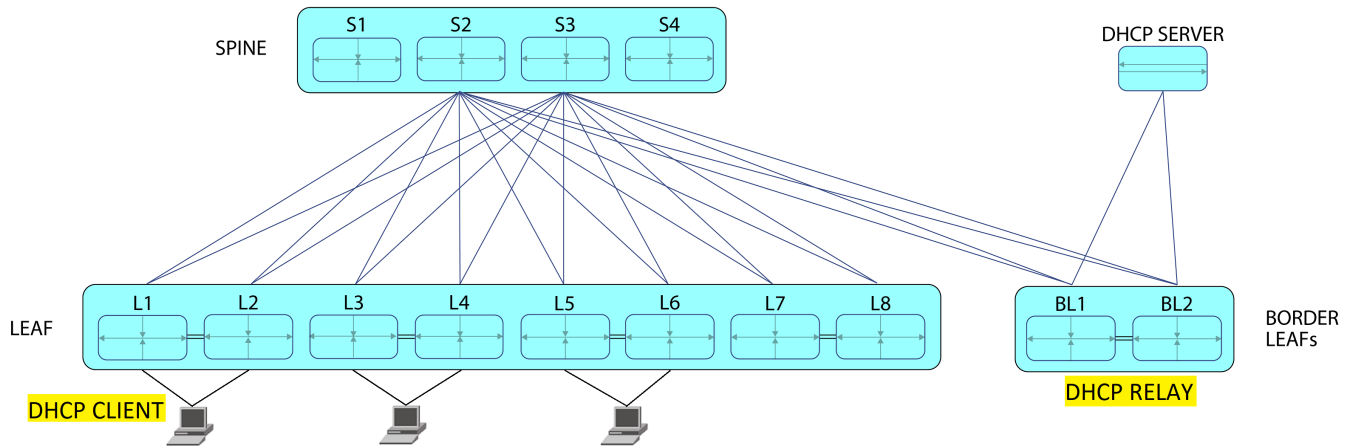
Figure 46: DHCP Relay Deployed in Centralized Routing Mode
