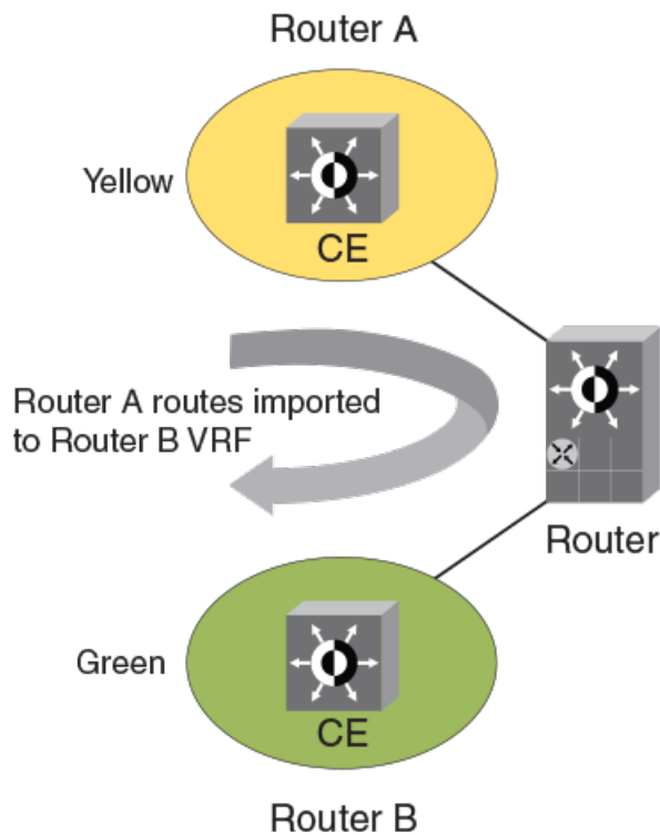
Figure 61: Dynamic inter-VRF route leaking
