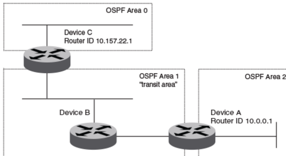
Figure 65: Defining OSPF virtual links within a network
