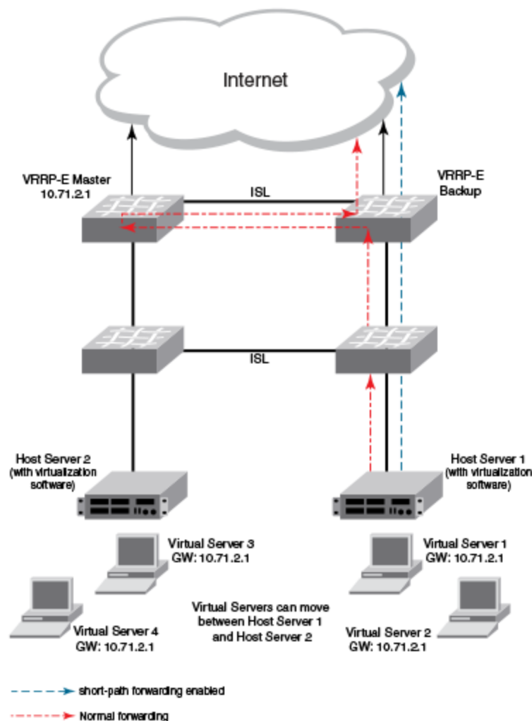
Figure 75: Short-path forwarding
