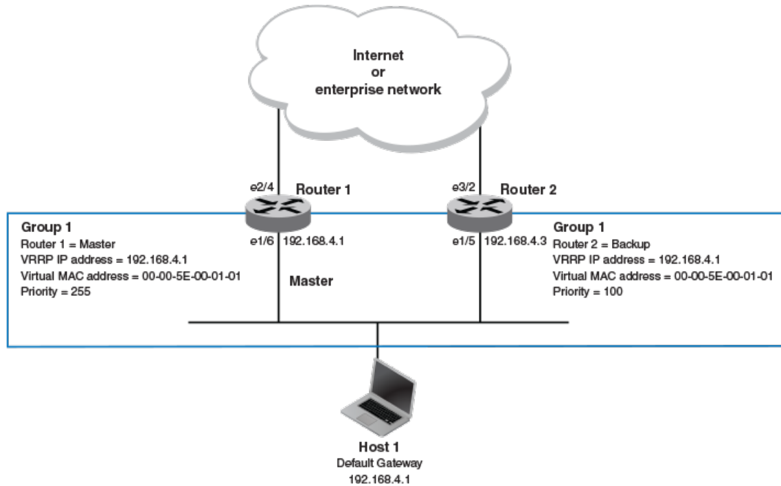
Figure 71: Basic VRRP topology
