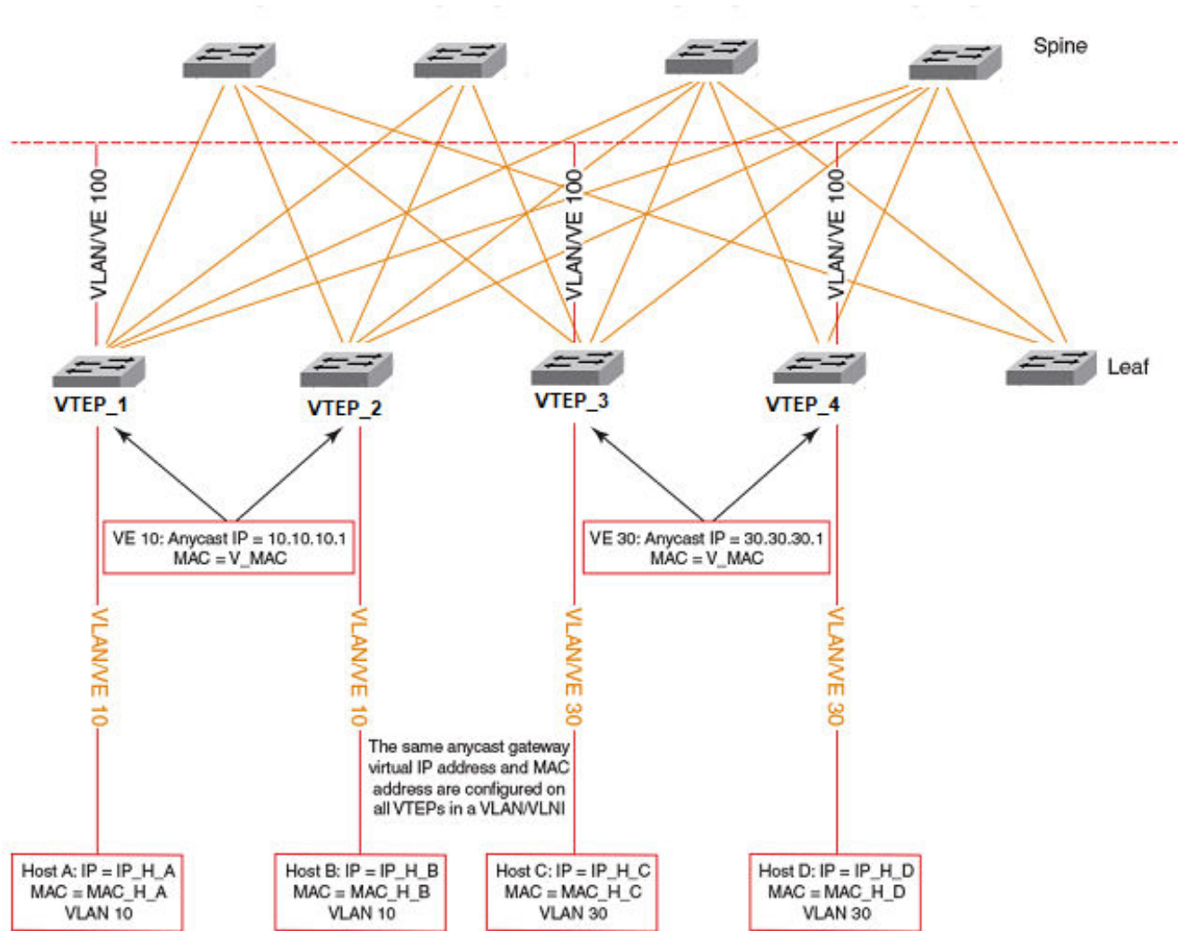
Figure 39: Static anycast gateway
