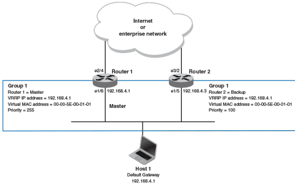
Figure 70: Devices configured as VRRP virtual routers for redundant network access for Host 1
