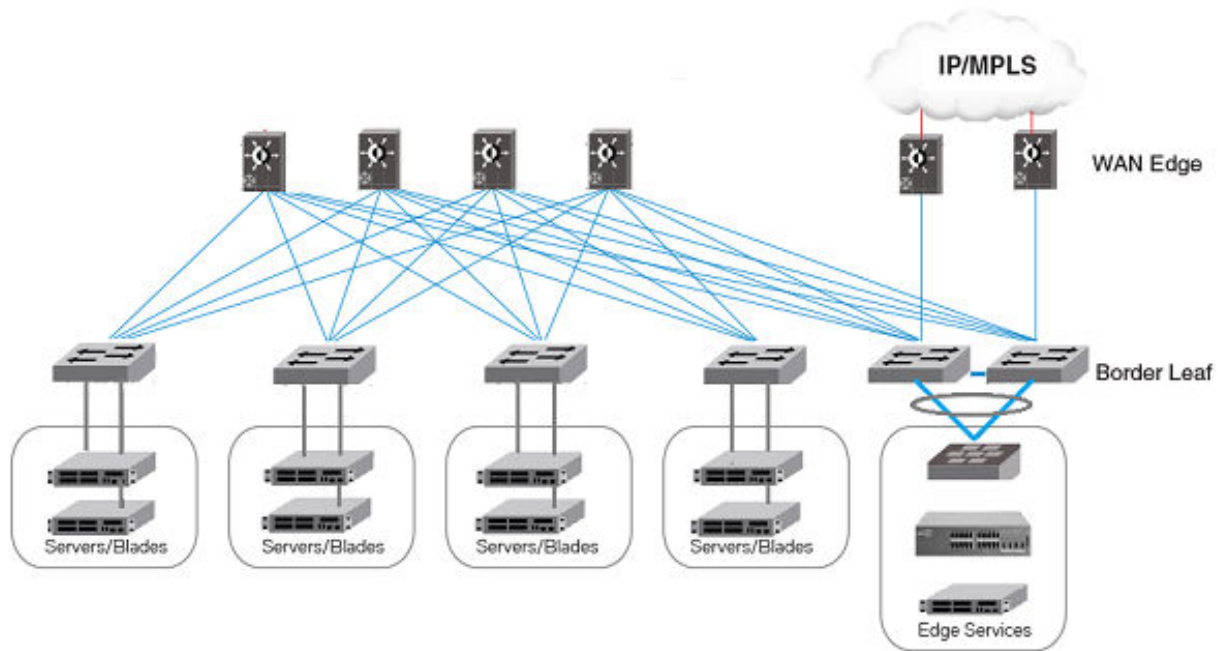
Figure 31: Border and service leaf
