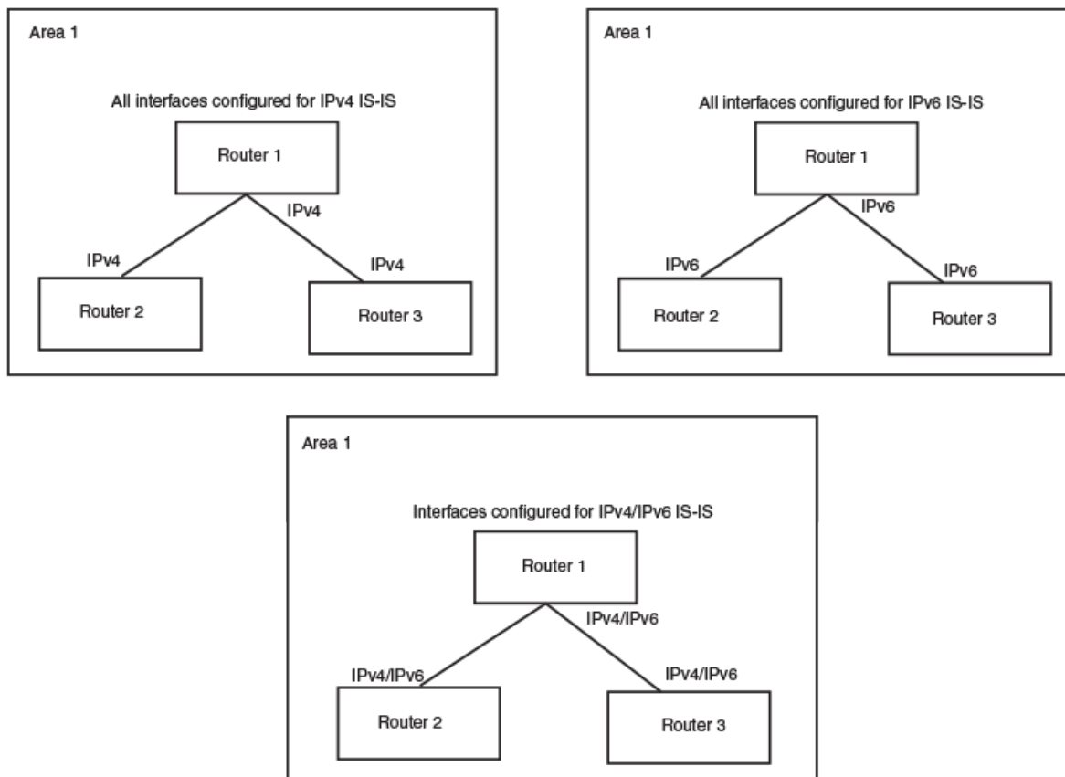
Figure 53: IPv6 IS-IS in single-topology mode
