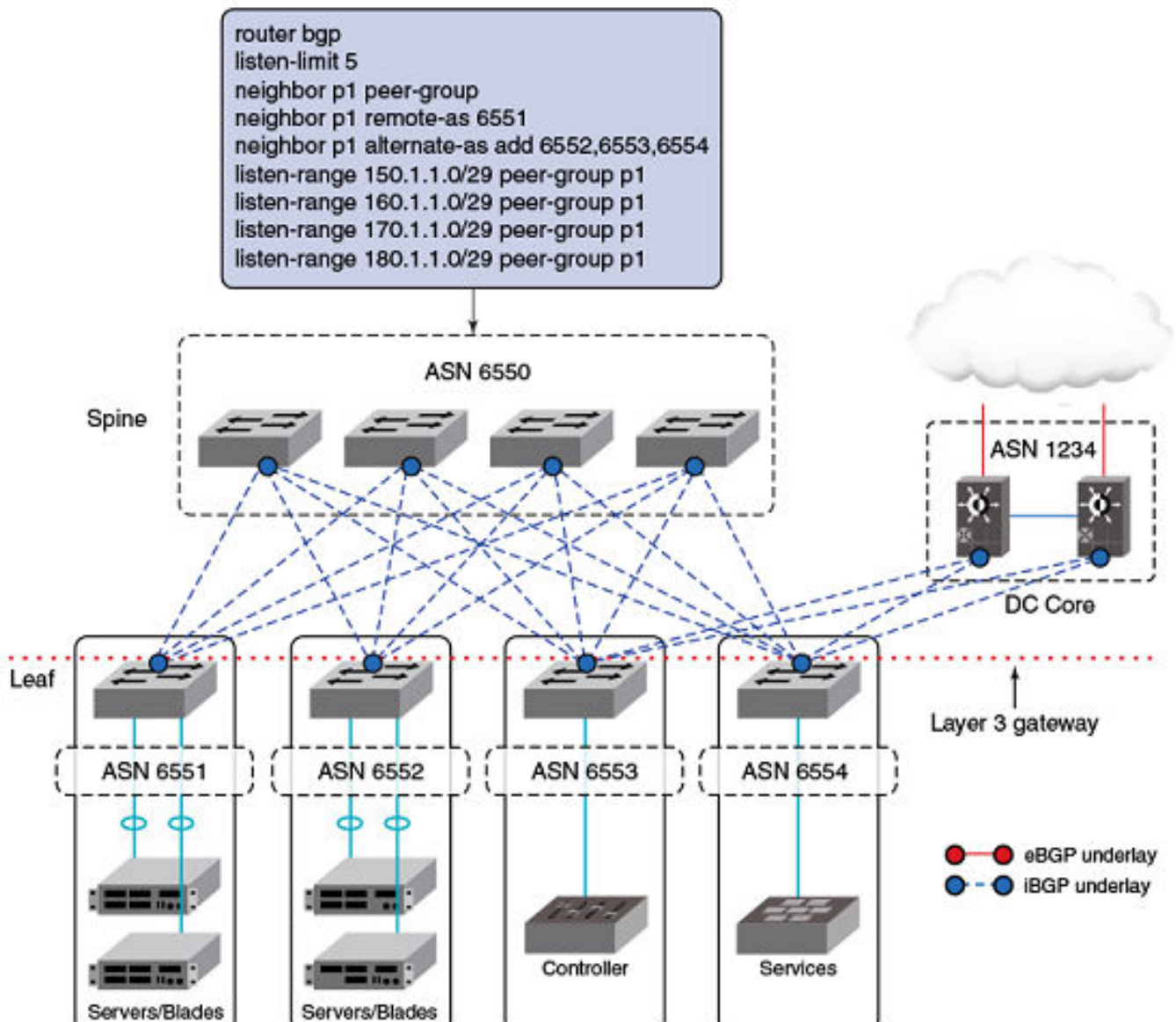
Figure 28: Minimum configuration at the spine level for BGP dynamic neighbors
