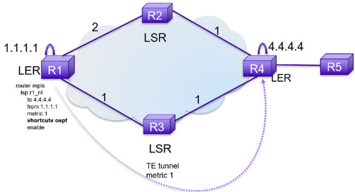
Figure 67: OSPF Shortcuts
