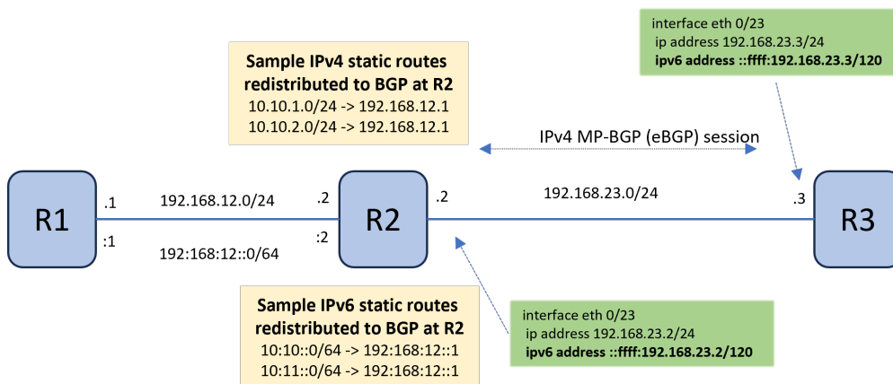
Figure 22: Configuration to successfully reach IPv6 nexthop for MP-BGP sessions
