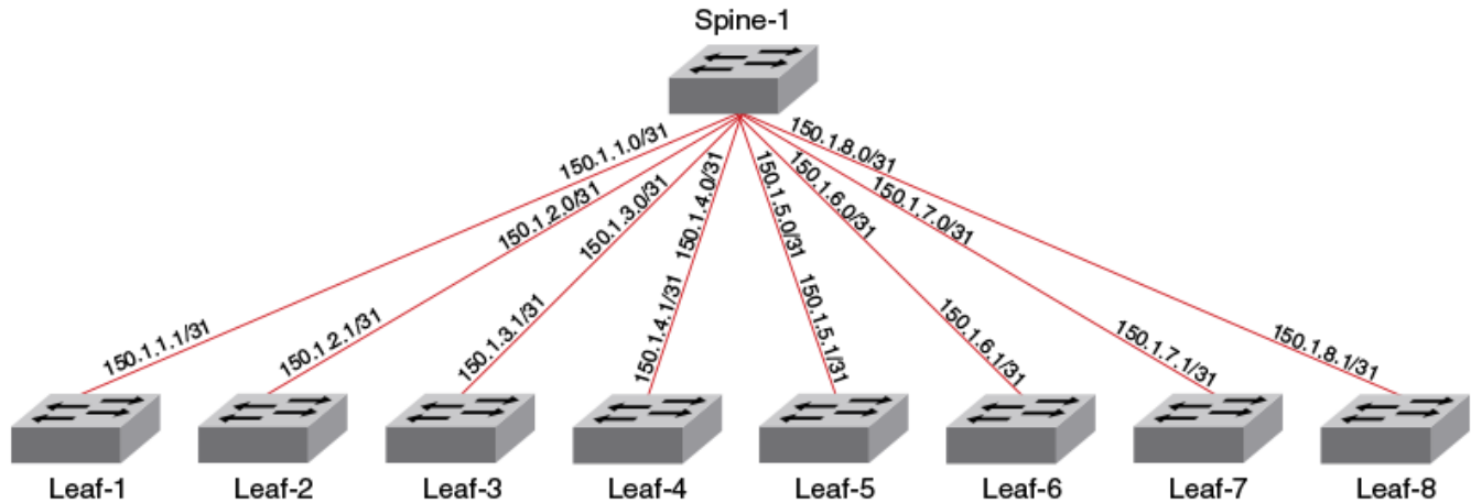
Figure 27: BGP session between spine and leaf nodes
