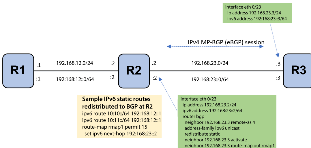
Figure 24: Using outbound route-map
