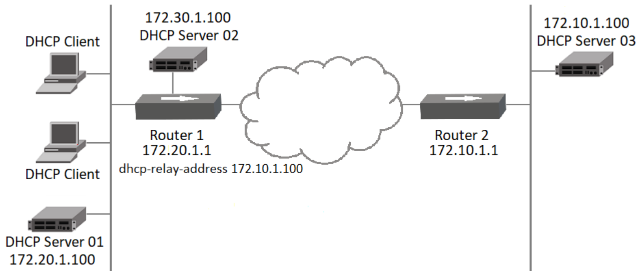
Figure 44: DHCP Relay Deployments
