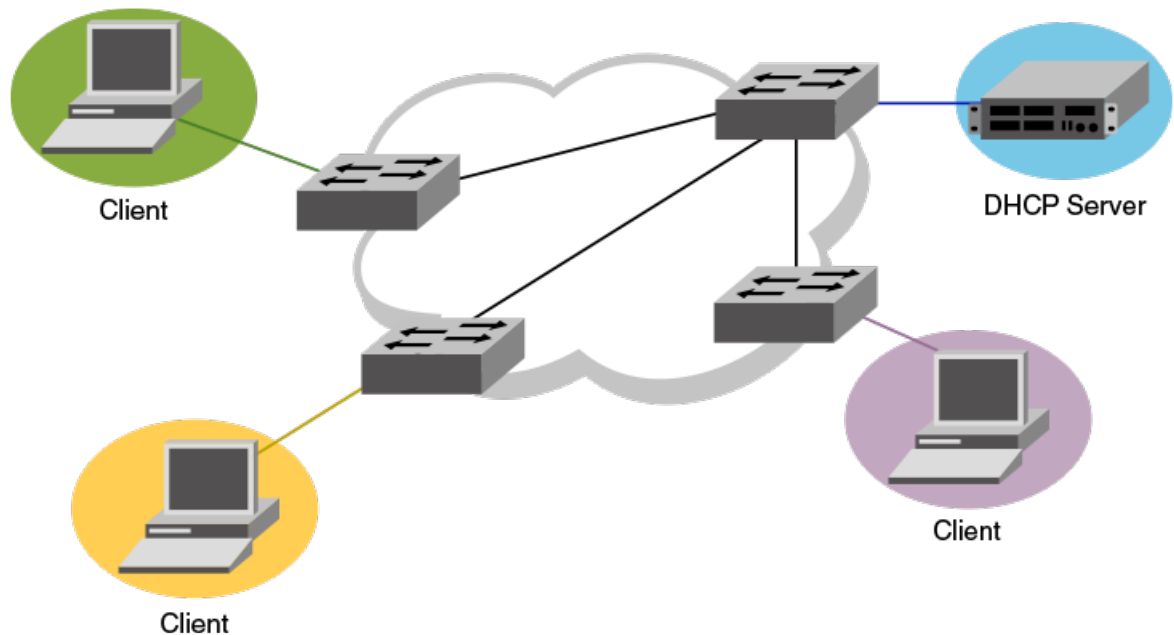
Figure 60: Inter-VRF route leaking example for connecting clients to a DHCP server in a different VRF.
