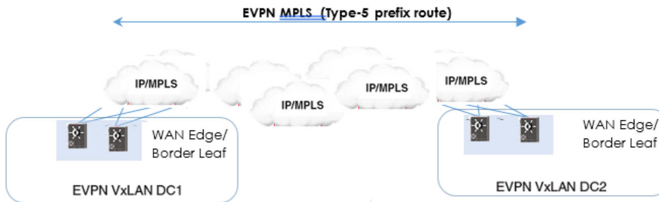
Figure 37: EVPN Type-5 prefix route termination and reorigination on the WAN edge
