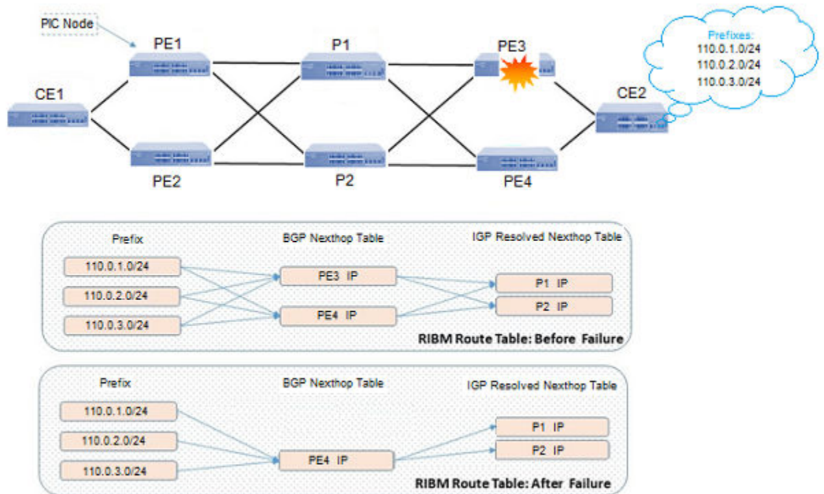
Figure 19: BGP PIC edge node failure
