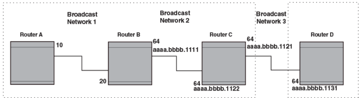
Figure 50: Each broadcast network has a Level-1 Designated IS and a Level-2 Designated IS
