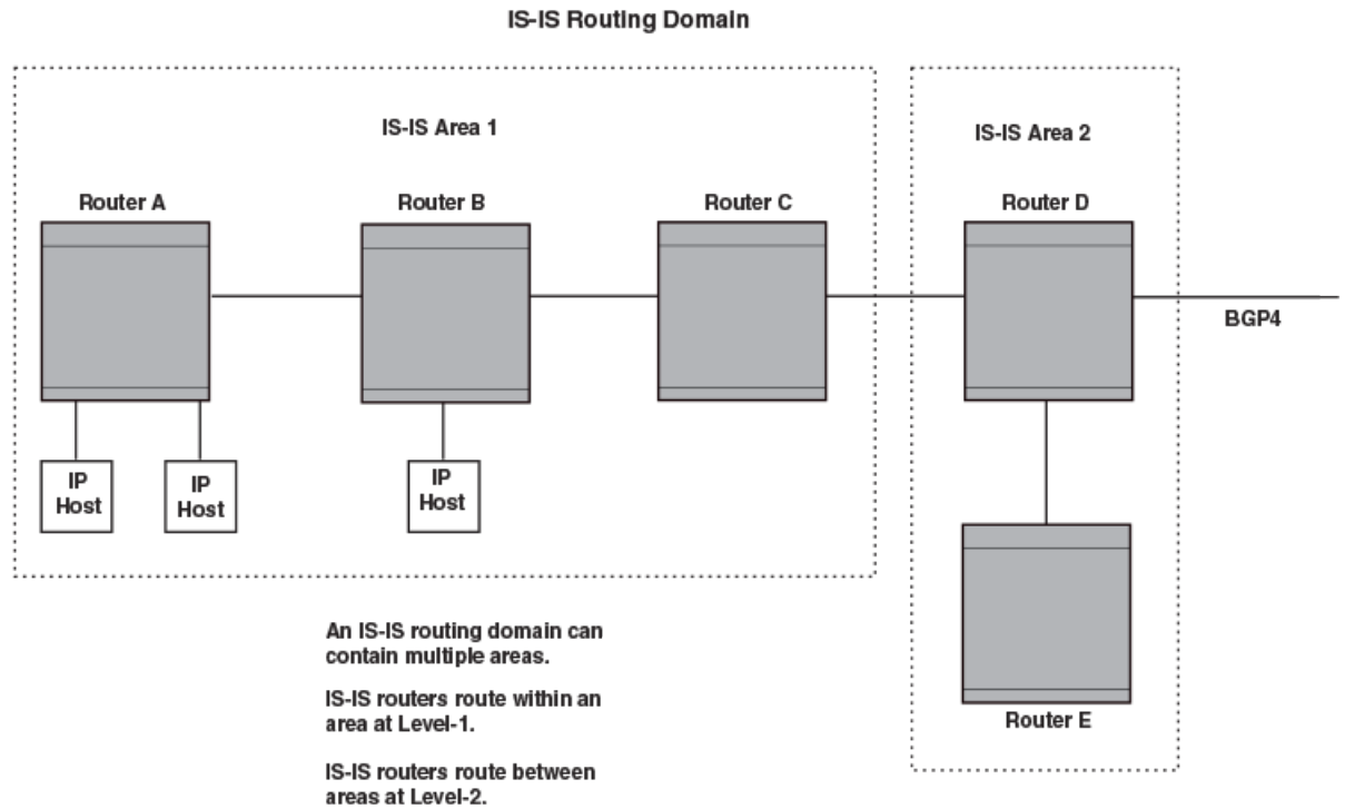
Figure 49: An IS-IS network contains Intermediate Systems (ISs) and host systems
