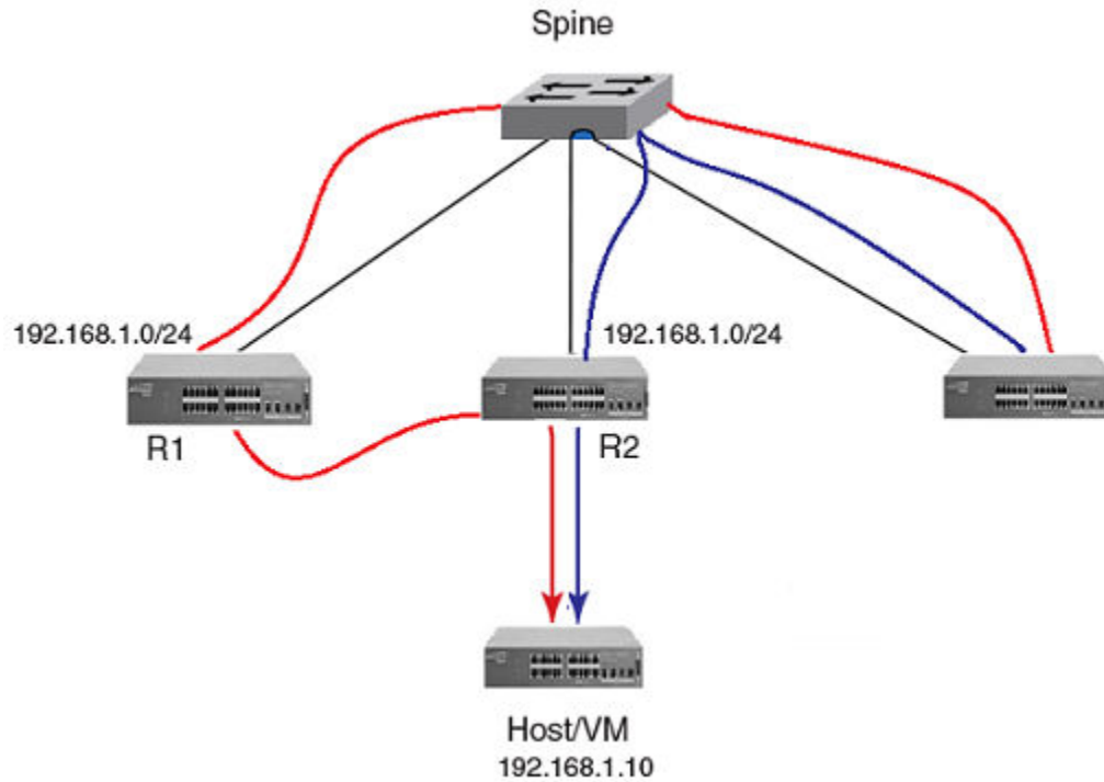
Figure 33: Avoiding suboptimal paths by converting MACIP routes to host routes
