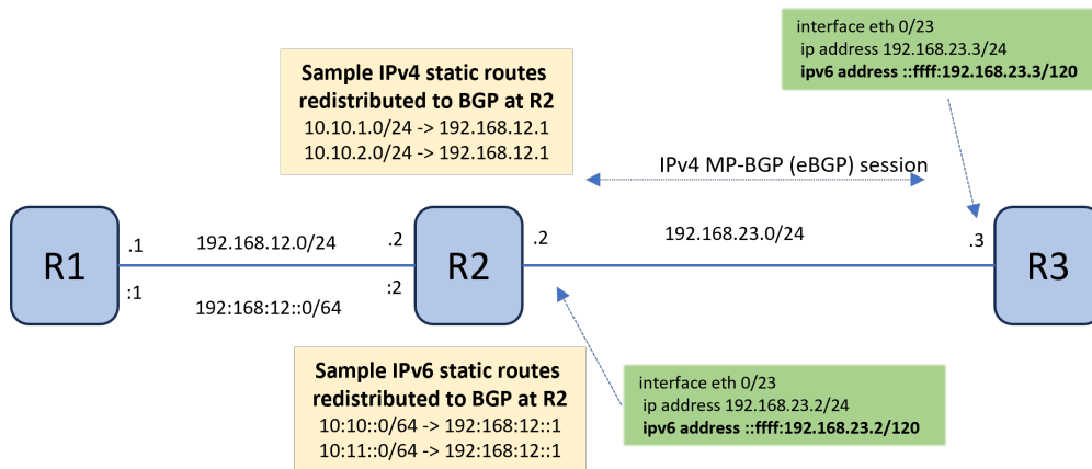
Figure 23: Configuration to successfully reach IPv6 nexthop for MP-BGP sessions
