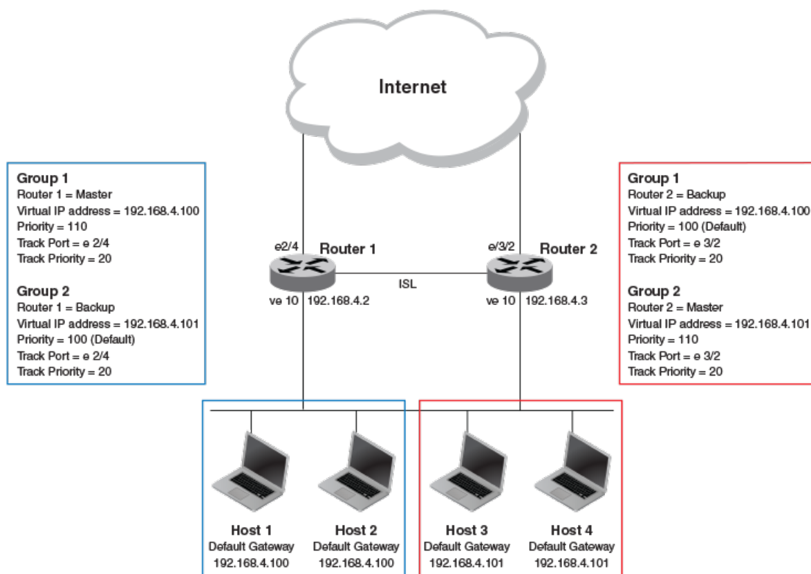
Figure 72: Two routers configured for dual redundant network access for the host
