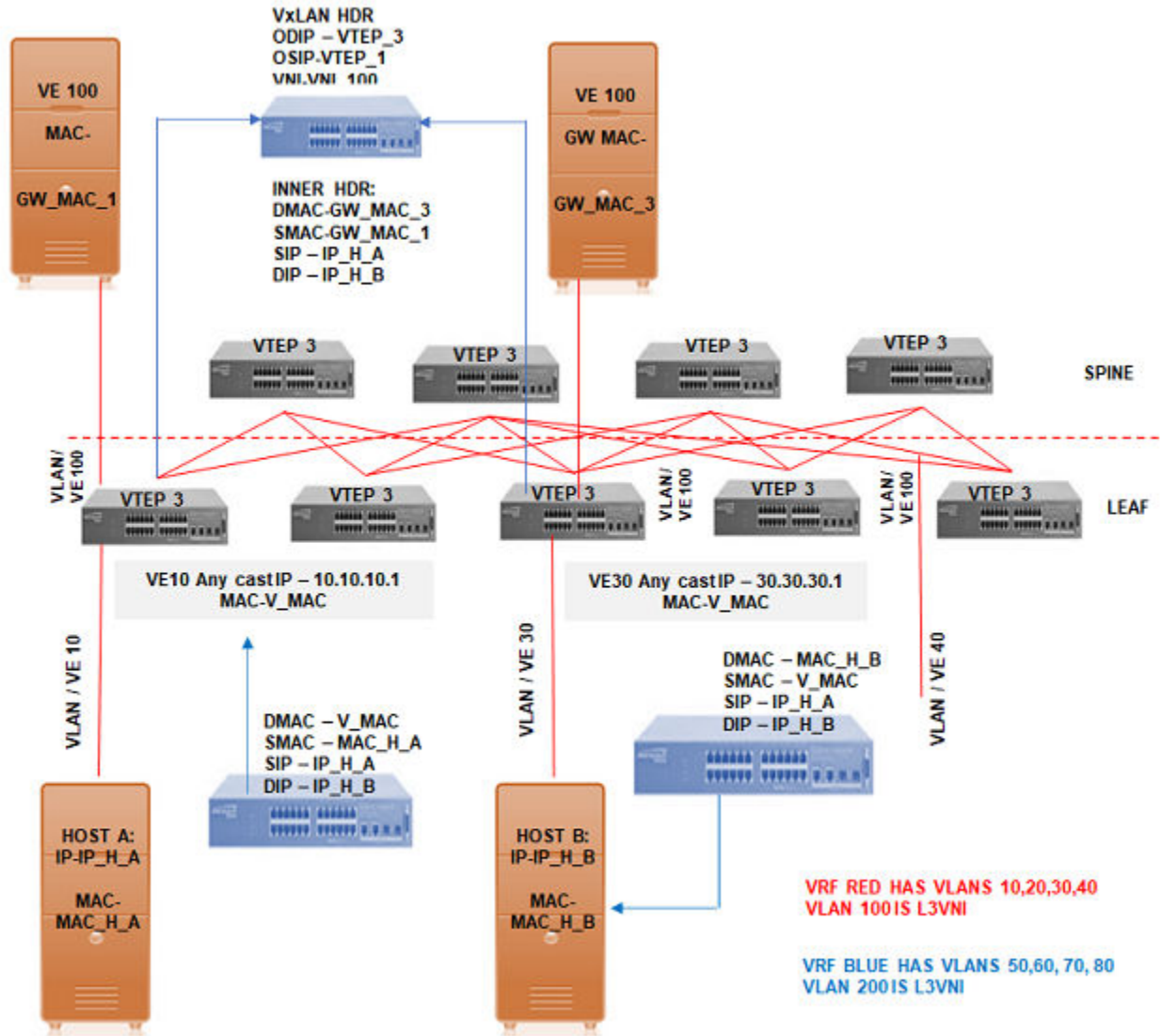
Figure 77: Layer 3 VNI on a single VTEP
