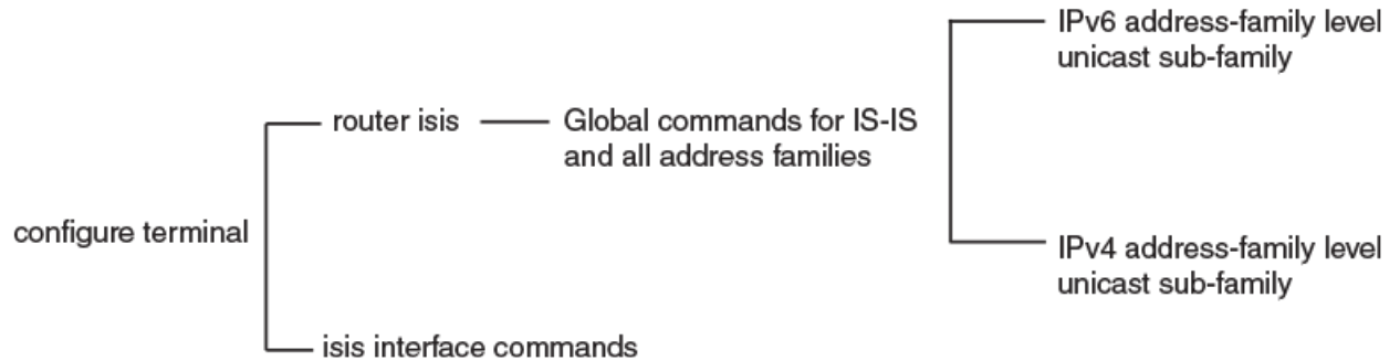
Figure 54: IPv6 IS-IS CLI levels
