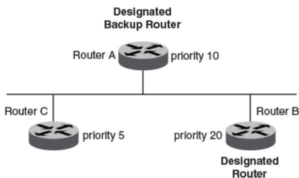
Figure 63: Designated and backup router election
