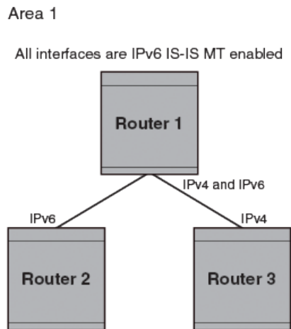
Figure 55: IS-IS non-congruent topology
