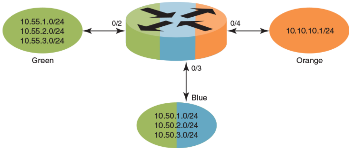
Figure 59: Static inter-VRF route leaking
