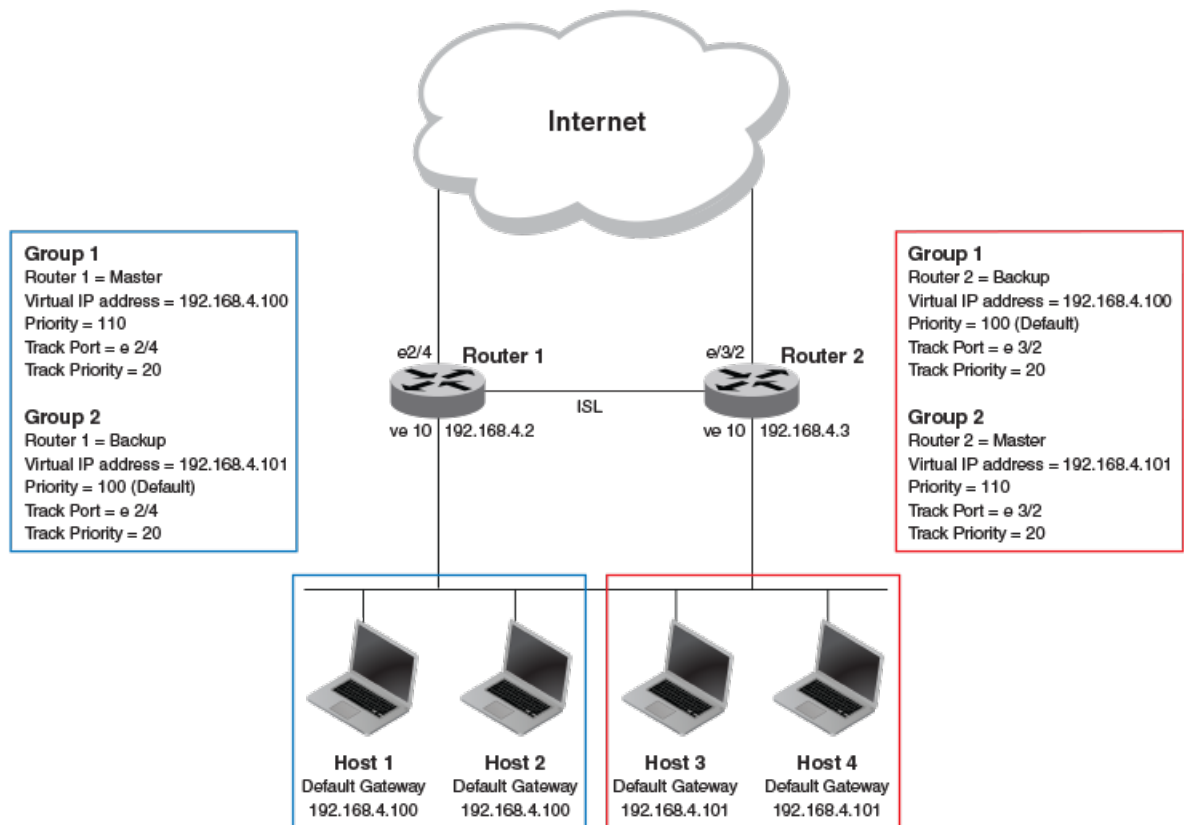
Figure 73: Multigroup VRRP routing topology
