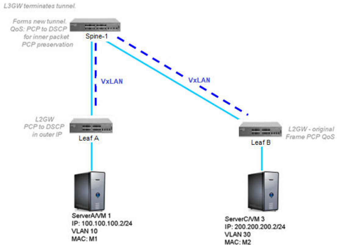
Figure 79: QoS for VxLAN Layer 2 and Layer 3 gateway interconnections
