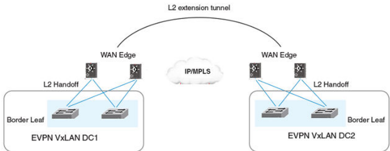
Figure 35: Layer 2 handoff-based DCI
