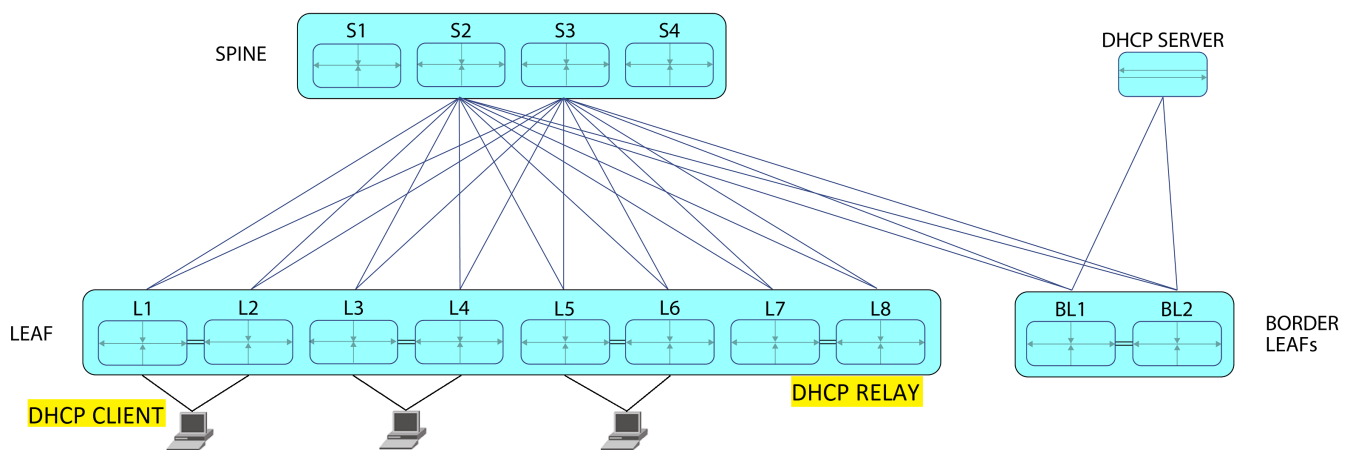
Figure 47: DHCP Relay Deployed in Distributed Routing Mode
