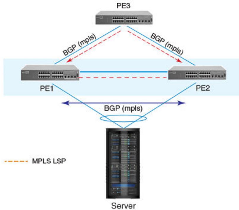
Figure 32: Aliasing in MPLS
