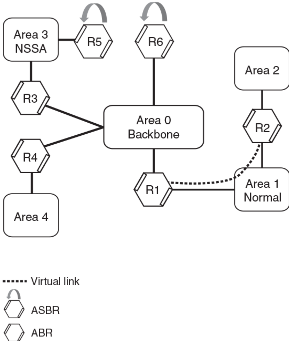
Figure 68: OSPFv3 virtual link
