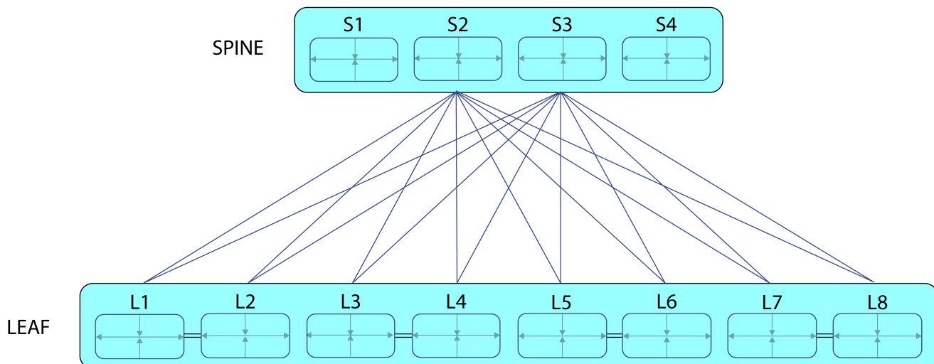
Figure 45: Typical IP Fabric Deployment
