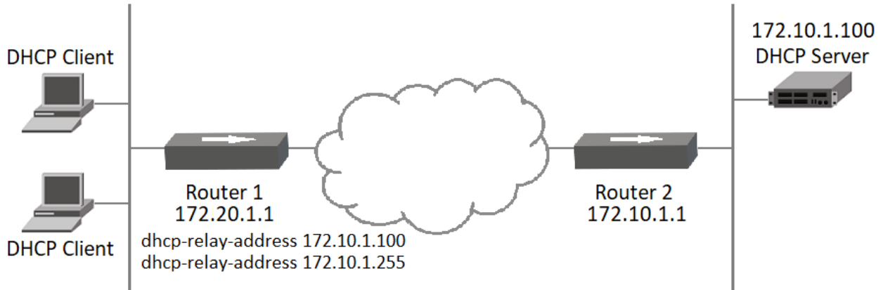
Figure 43: DHCP Relay Configuration
