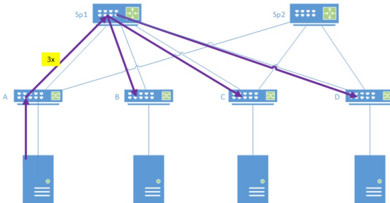
Figure 10: Overview of Ingress Replication
