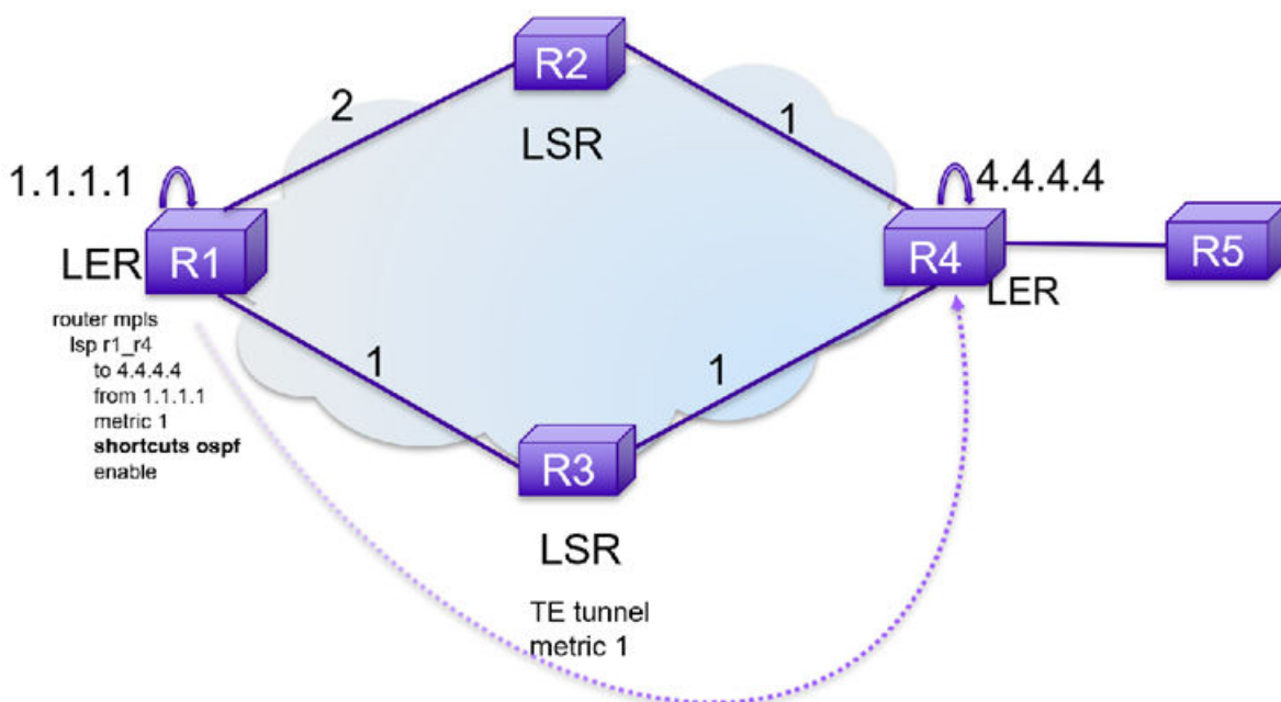
Figure 66: OSPF Shortcuts
