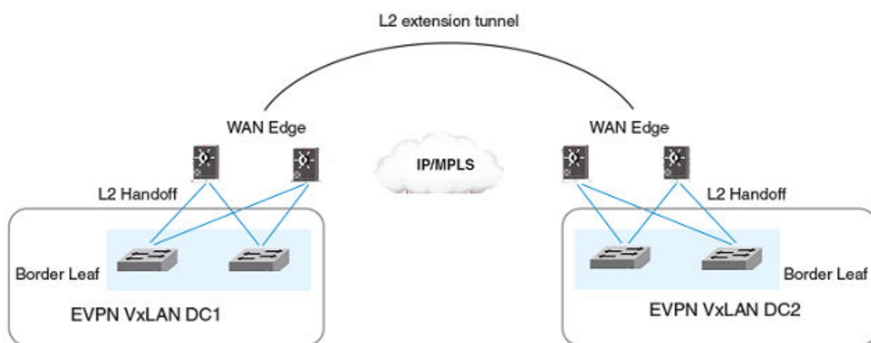
Figure 34: Layer 2 handoff-based DCI
