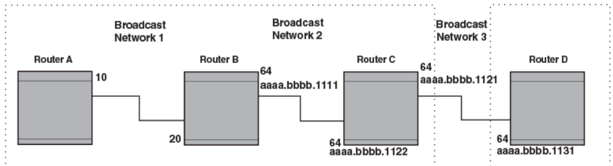
Figure 49: Each broadcast network has a Level-1 Designated IS and a Level-2 Designated IS
