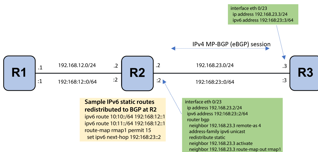
Figure 23: Using outbound route-map
