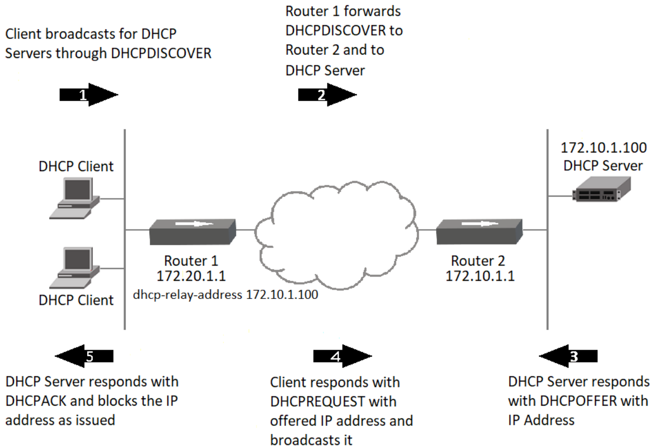
Figure 41: DHCP Message Exchange
