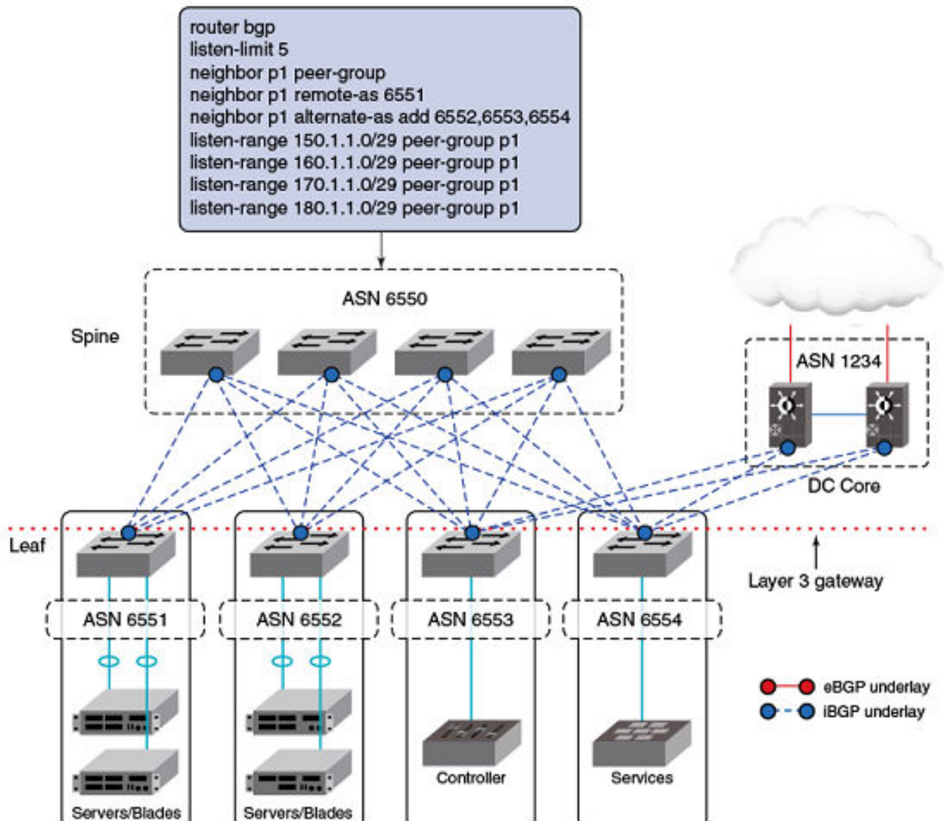
Figure 27: Minimum configuration at the spine level for BGP dynamic neighbors
