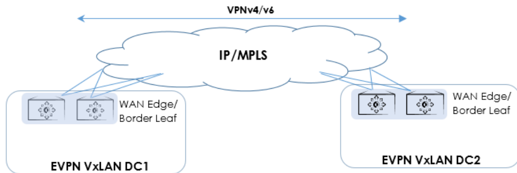
Figure 37: Data center Layer 3 interconnect with EVPN VxLAN and VPNv4/v6
