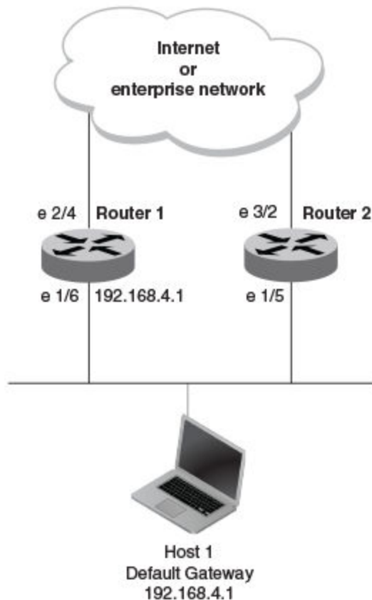
Figure 68: Single point of failure with Device 1 being the Host1 default gateway
