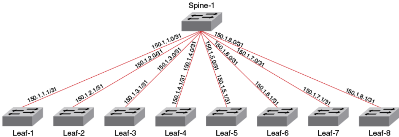
Figure 26: BGP session between spine and leaf nodes
