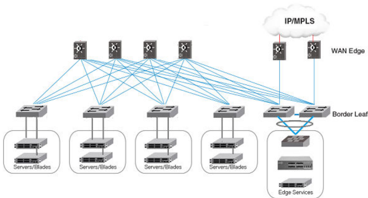
Figure 30: Border and service leaf
