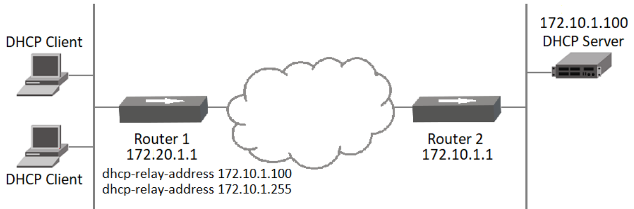
Figure 42: DHCP Relay Configuration
