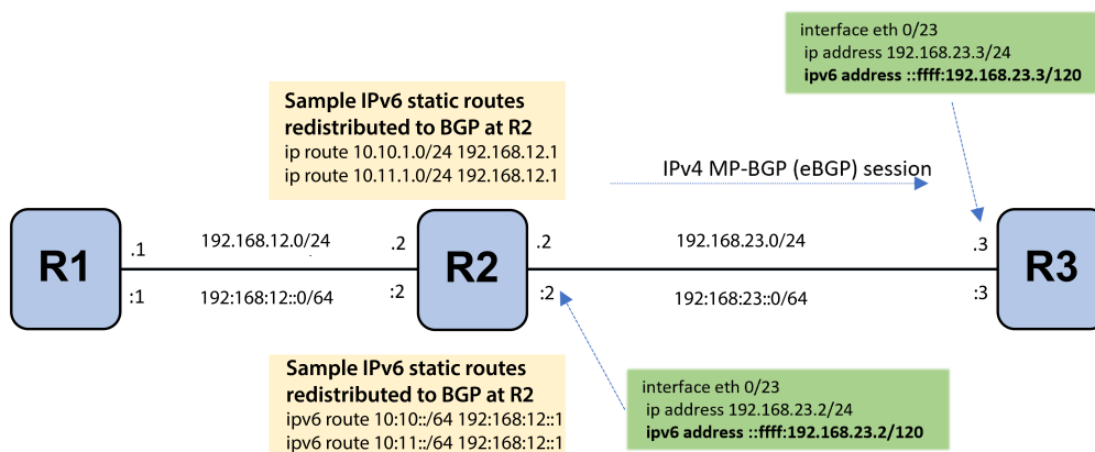
Figure 22: Configuration to successfully reach IPv6 nexthop for MP-BGP sessions
