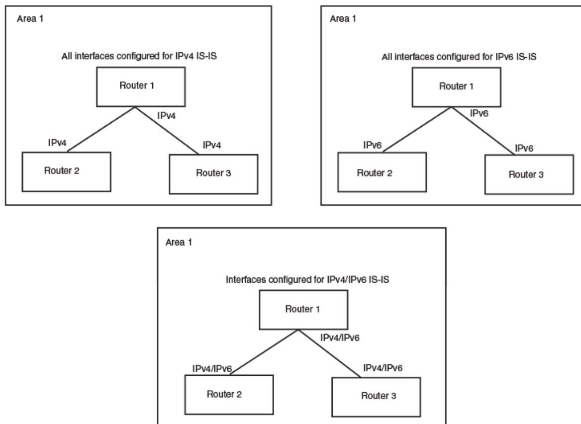
Figure 52: IPv6 IS-IS in single-topology mode
