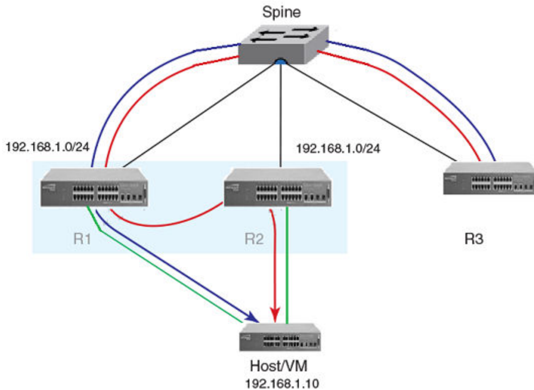
Figure 33: Avoiding traffic tromboning for EVPN Layer 3 traffic in an MCT cluster
