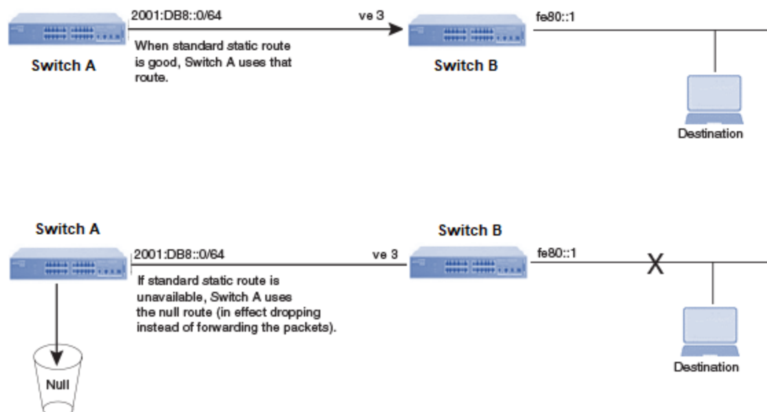
Figure 6: Null route and standard route to same destination
