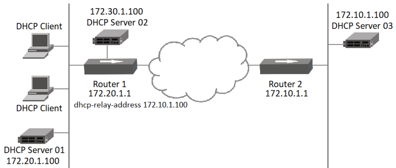
Figure 43: DHCP Relay Deployments
