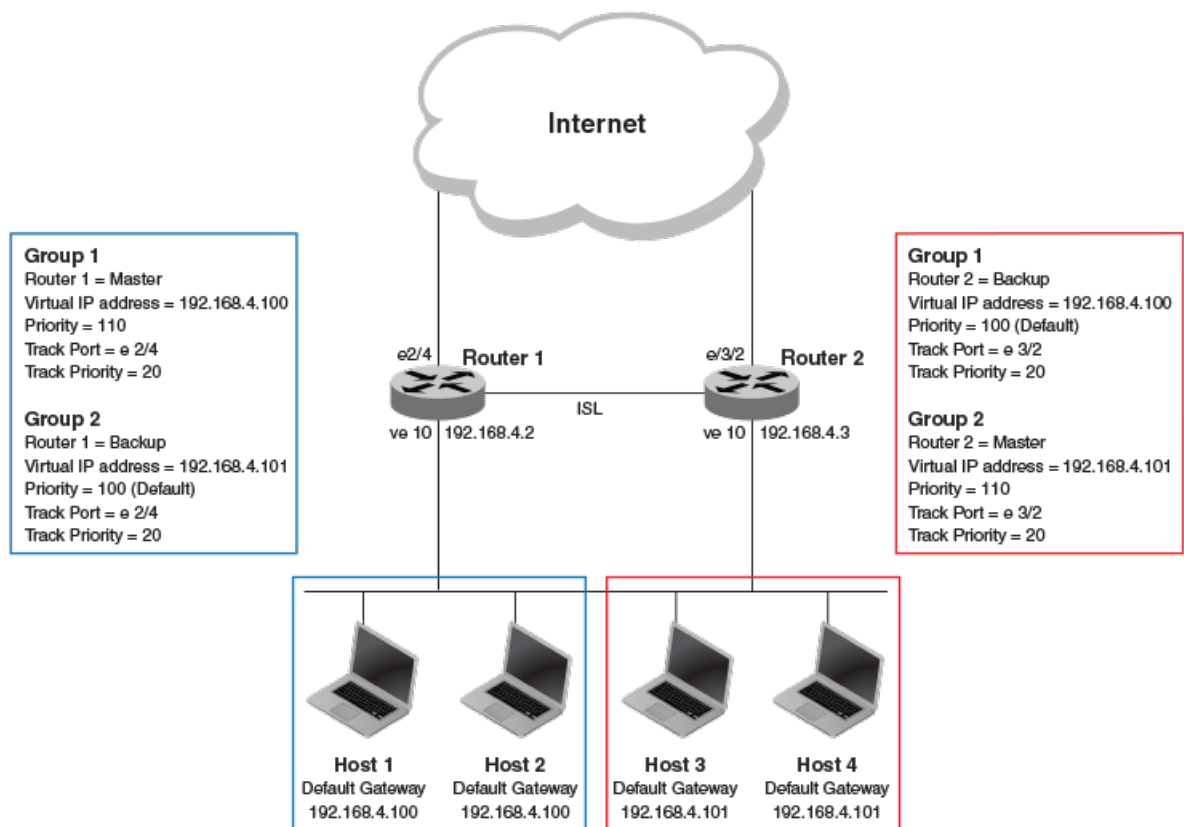
Figure 72: Multigroup VRRP routing topology
