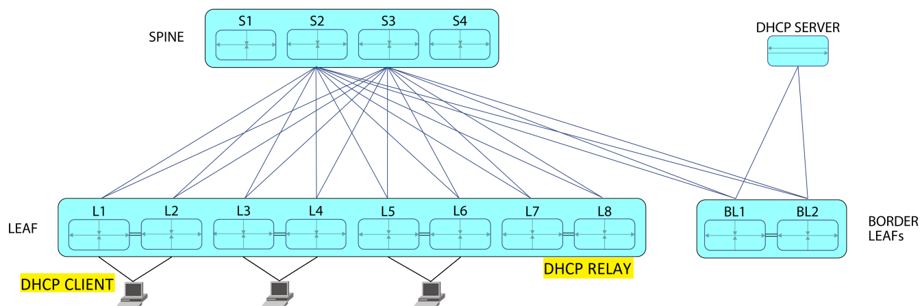
Figure 46: DHCP Relay Deployed in Distributed Routing Mode
