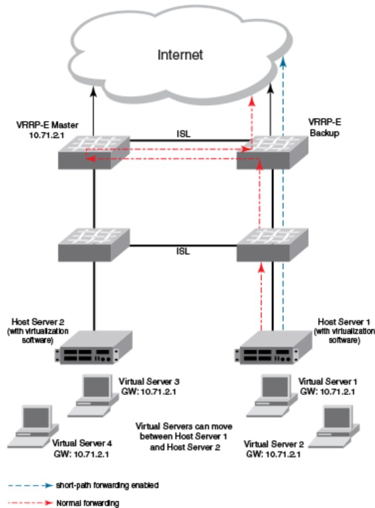
Figure 73: Short-path forwarding
