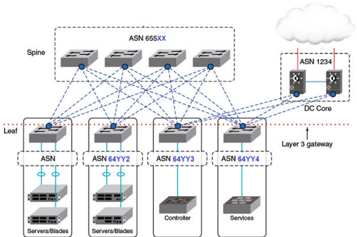
Figure 29: eBGP spine and leaf
