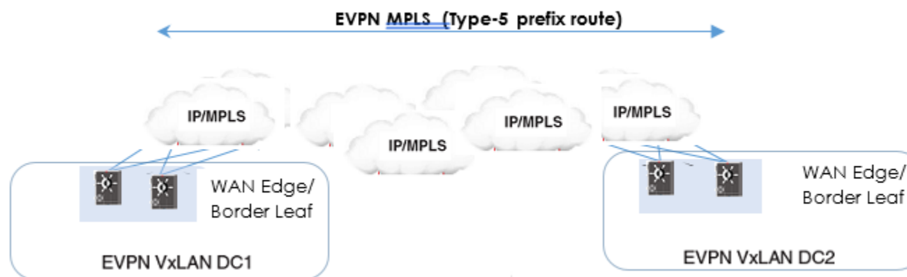
Figure 36: EVPN Type-5 prefix route termination and reorigination on the WAN edge
