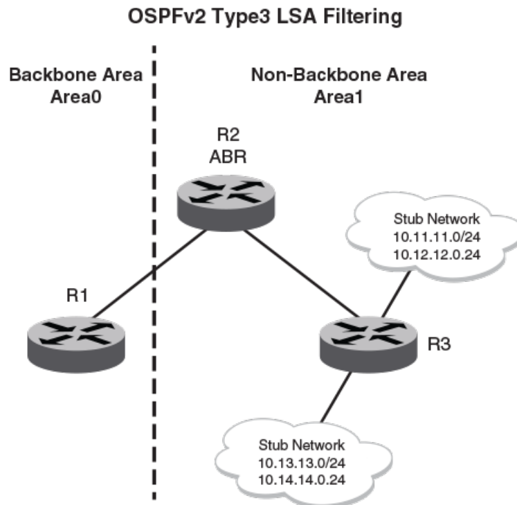
Figure 65: OSPFv2 type 3 LSA filtering
