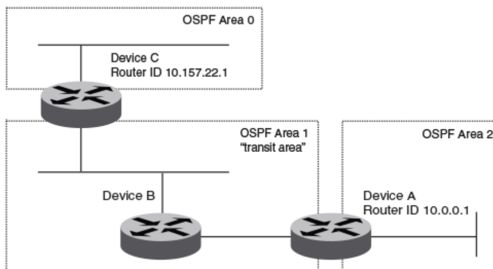
Figure 64: Defining OSPF virtual links within a network
