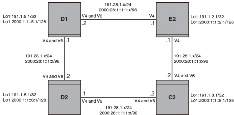
Figure 55: IPv6 IS-IS MT configuration
