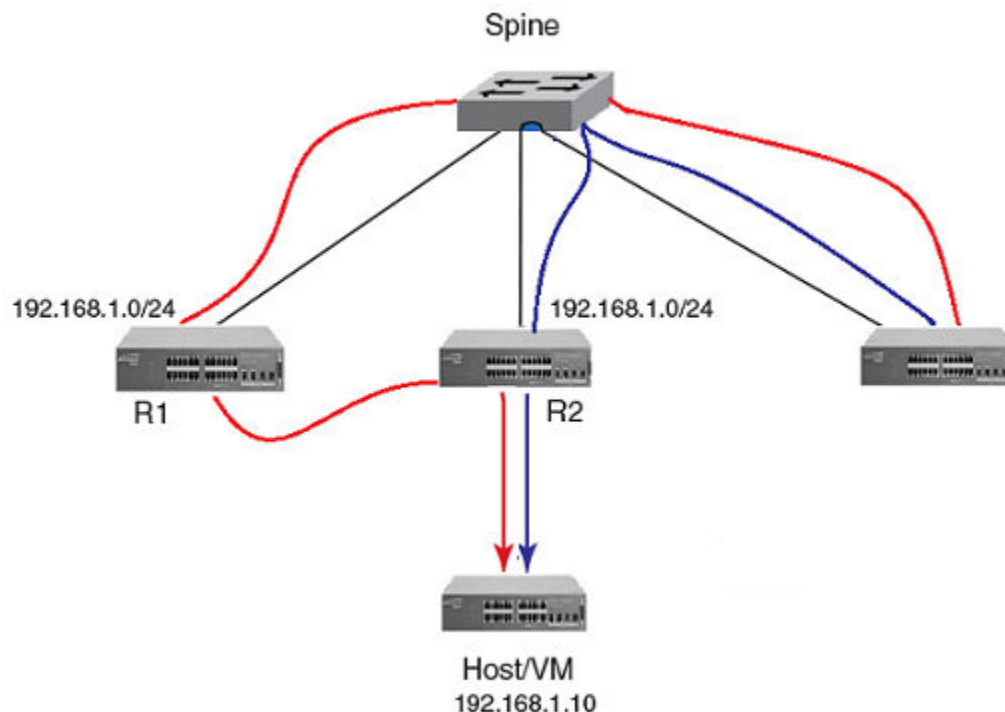
Figure 32: Avoiding suboptimal paths by converting MACIP routes to host routes
