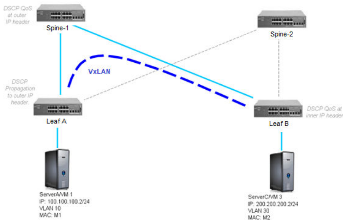
Figure 79: VxLAN L3 gateway support of intersubnet communication
