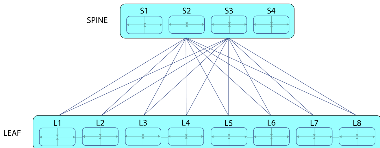
Figure 44: Typical IP Fabric Deployment
