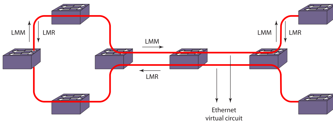
Figure 55: Two-Way Frame-Loss Measurement
