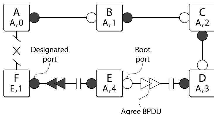
Figure 174: Communicating Port Status to Neighbors
