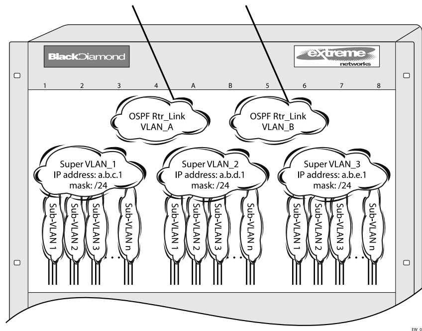
Figure 229: VLAN Aggregation
