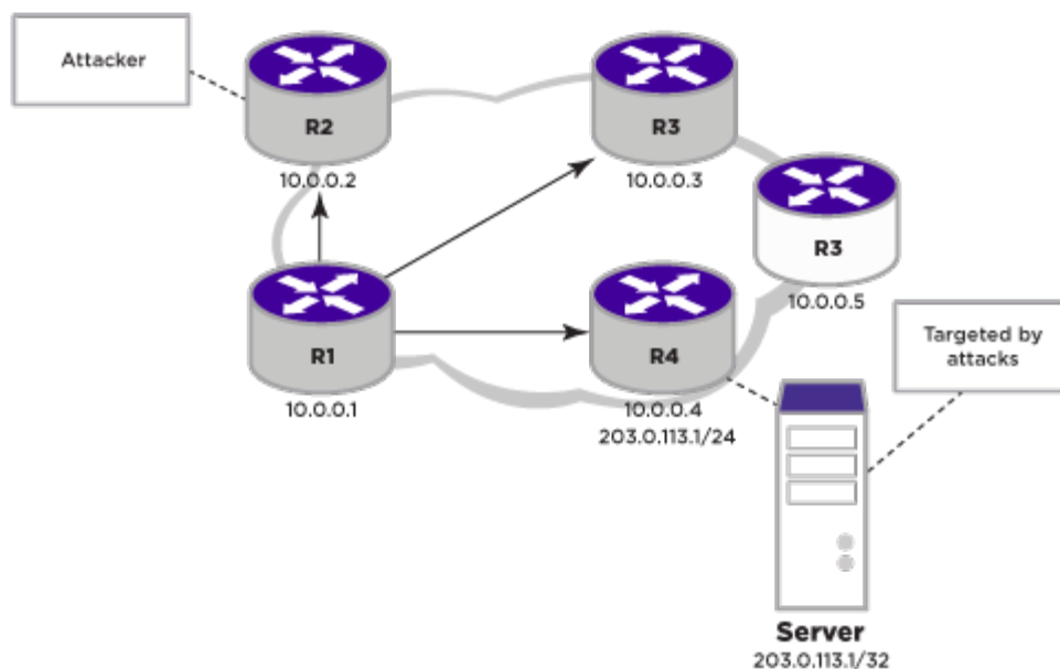
Figure 261: Black Hole Routing Using BGP
