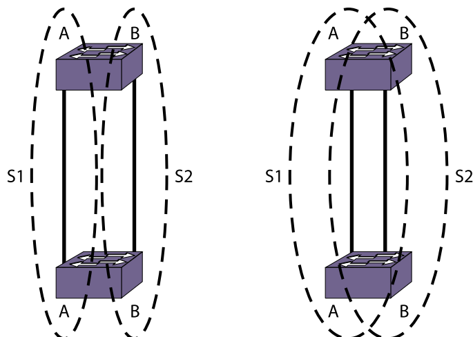
Figure 164: Limitations of Traditional STPD
