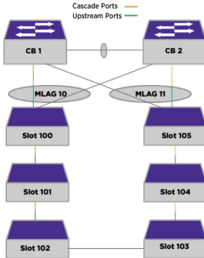
Figure 38: Cross-Connect MLAG
