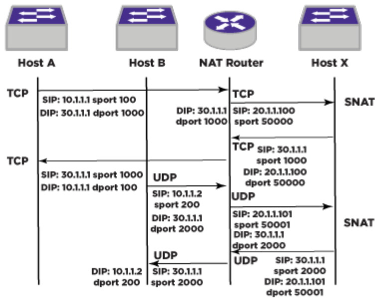
Figure 232: NAPT Example
