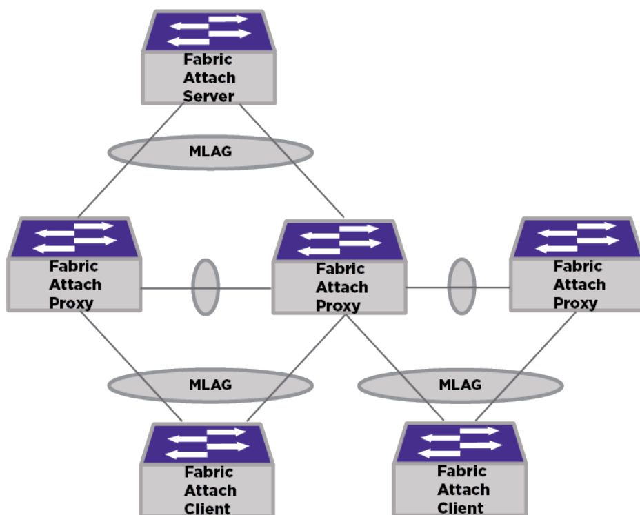
Figure 89: Fabric Attach with W-MLAG
