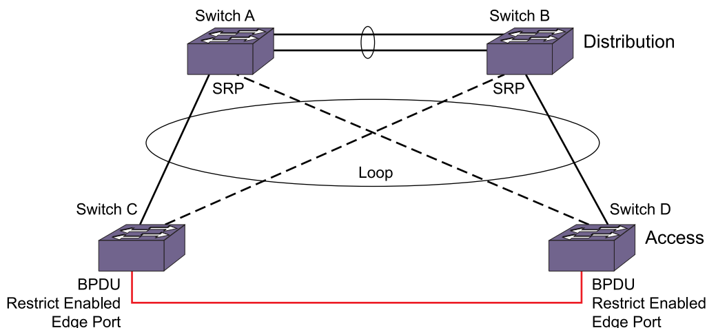
Figure 161: BPDU Restrict
