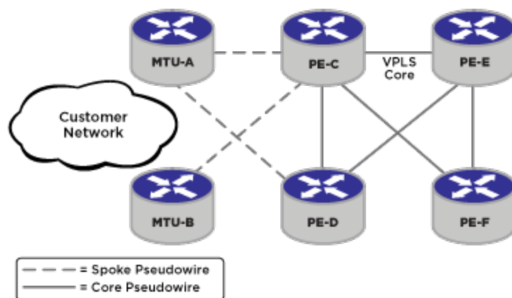
Figure 212: Example Redundant Edge H-VPLS Network
