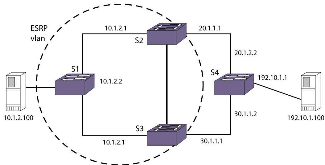
Figure 119: MAC Address Limits and VLANs Participating in ESRP
