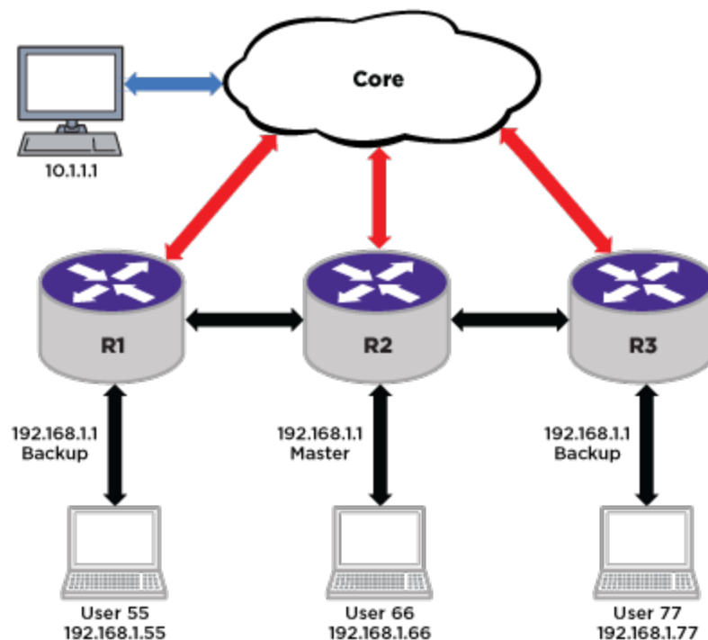
Figure 197: Asymmetric Routing and VRRP (1)
