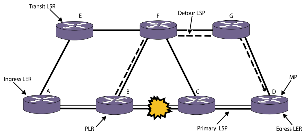
Figure 217: Fast-Reroute Terminology
