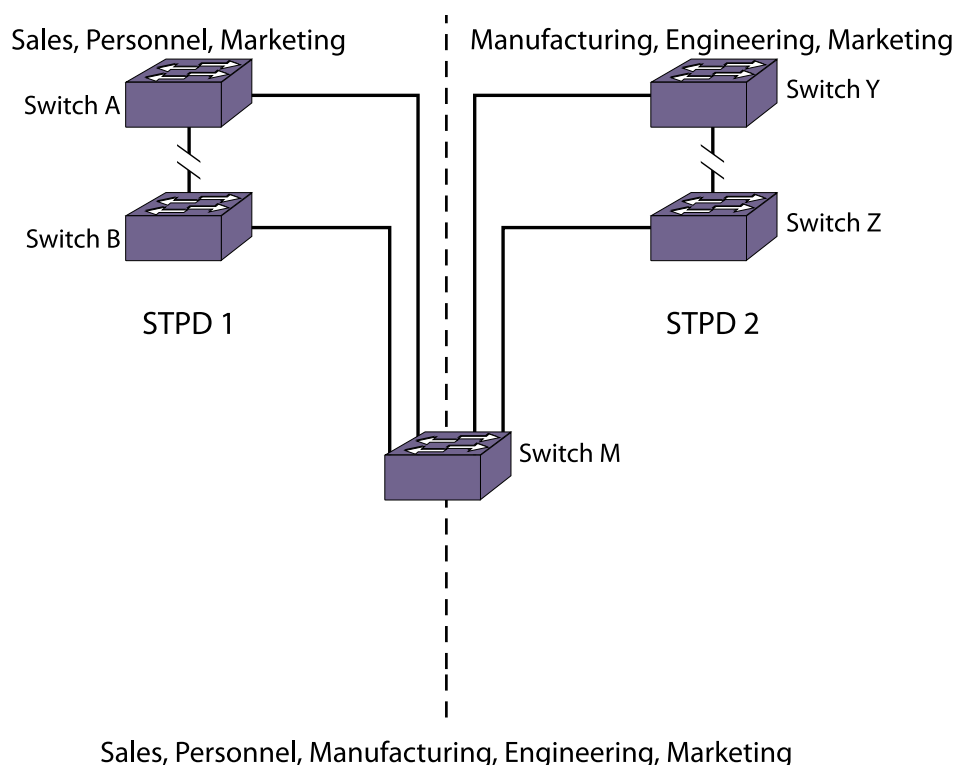
Figure 162: Multiple STPDs
