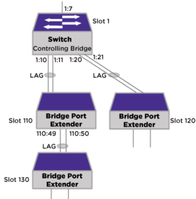
Figure 42: CB with Two-Tier BPEs Topology
