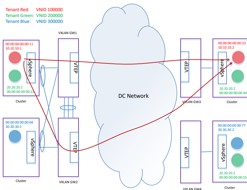
Figure 115: VXLAN Gateways with Three Tenants
