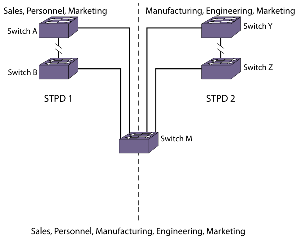
Figure 185: RSTP Example
