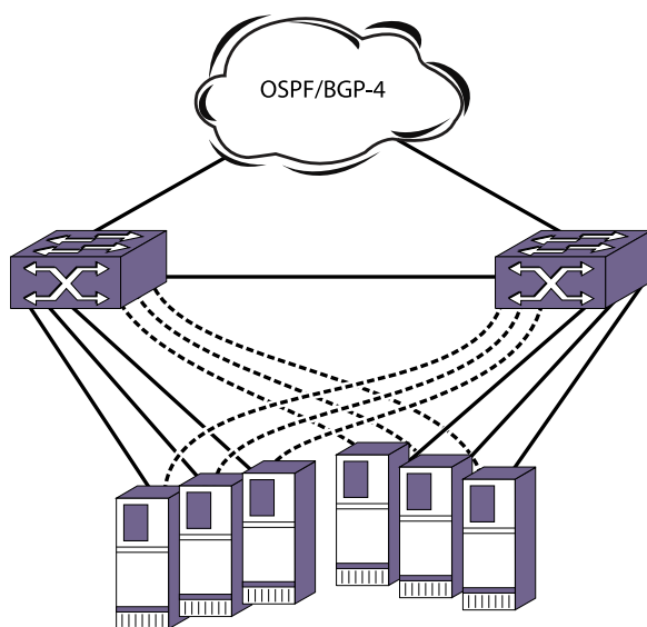
Figure 190: ESRP Host Attach
