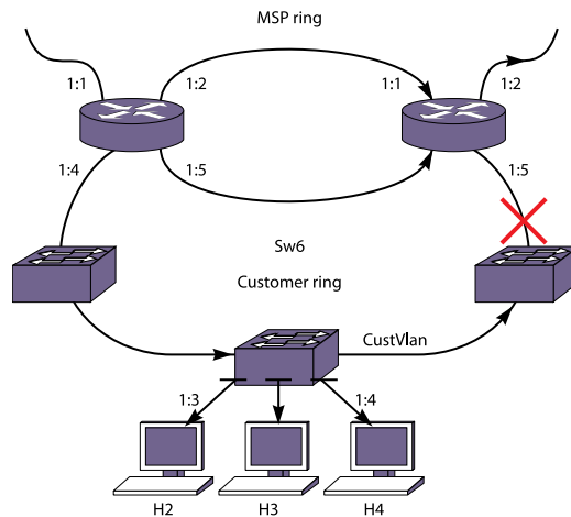
Figure 277: Inter-Multicast VLAN Forwarding
