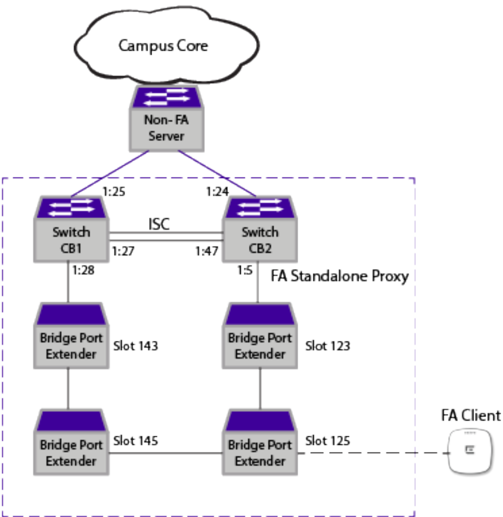
Figure 92: FA Clients Connected to BPEs with Extended Edge Switching Ring MLAG-Connected CBs FA Standalone Peers
