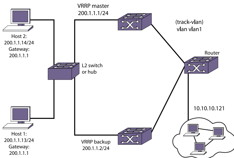
Figure 200: VRRP Tracking
