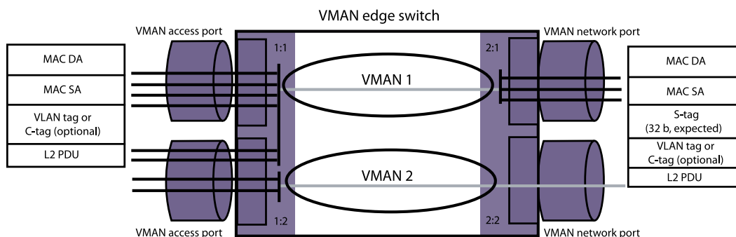
Figure 81: Tag Usage at the VMAN Access Switch
