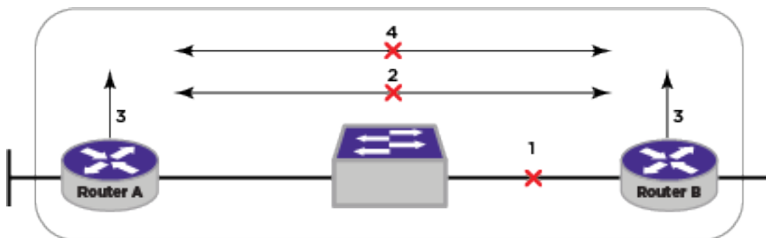
Figure 59: BFD Failure Detection
