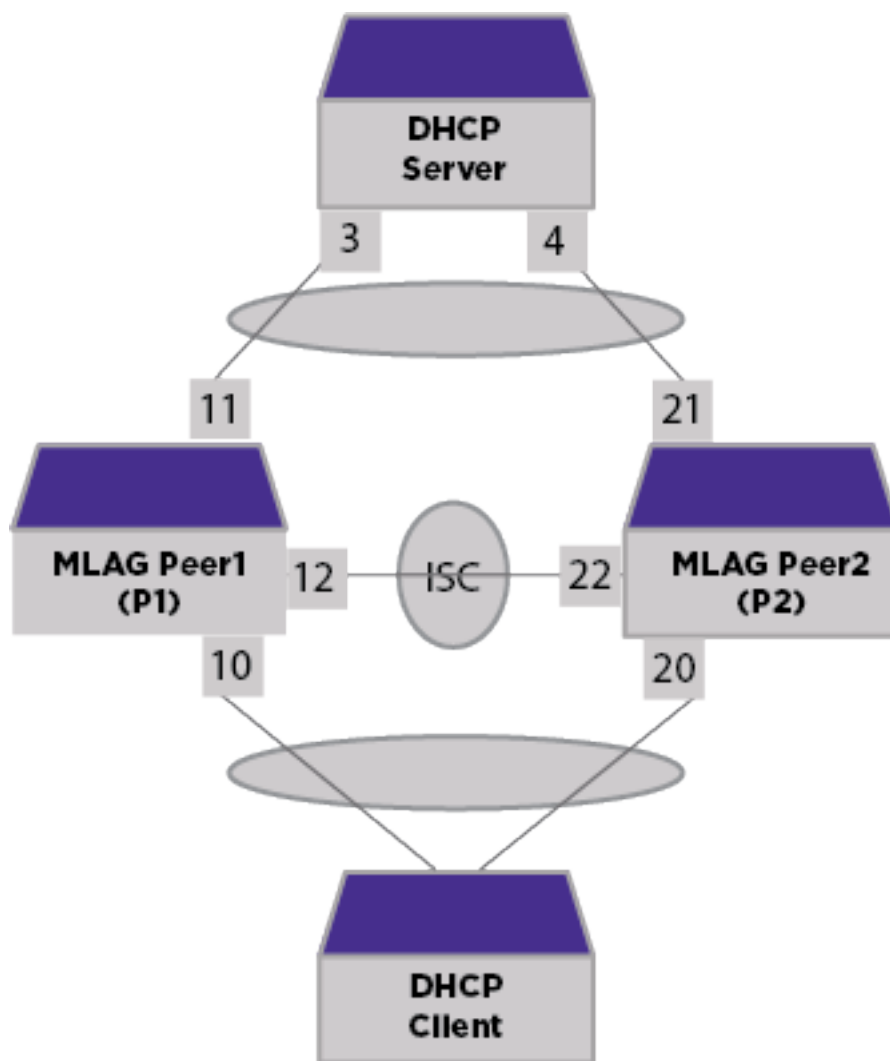
Figure 124: MLAG Topology
