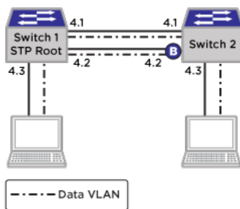
Figure 145: Sample STP Network for Migration to EAPS
