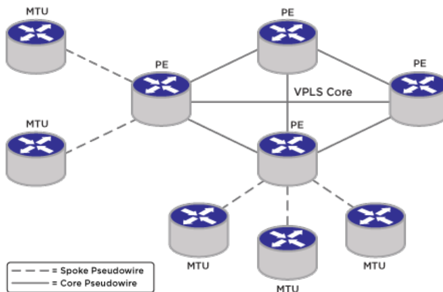
Figure 208: Example H-VPLS Network
