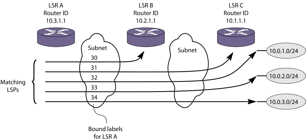
Figure 207: Matching and Calculated LSP Next Hops
