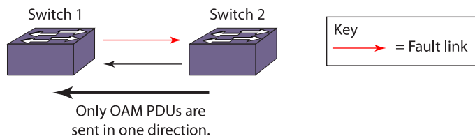
Figure 57: Normal Link and Unidirectional Operation
