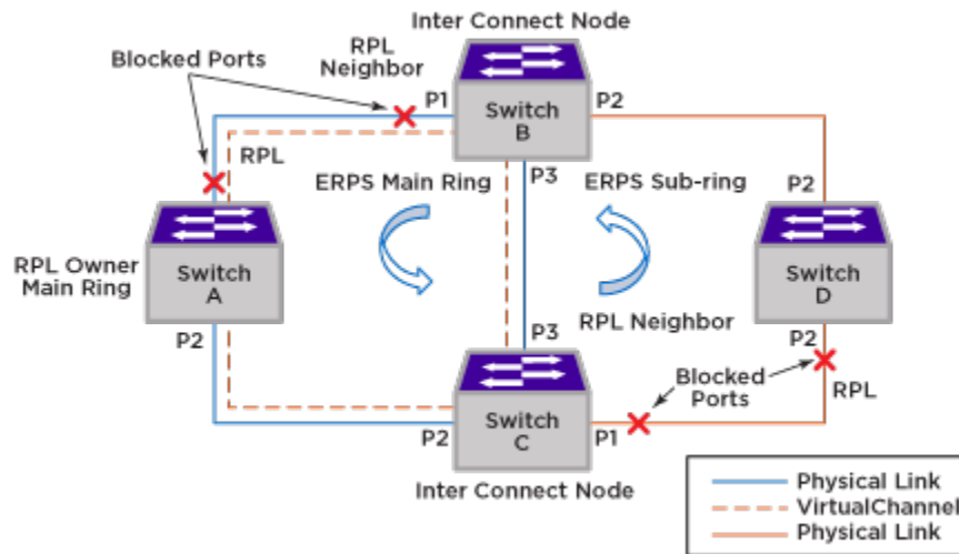
Figure 157: Sample ERPS Configuration
