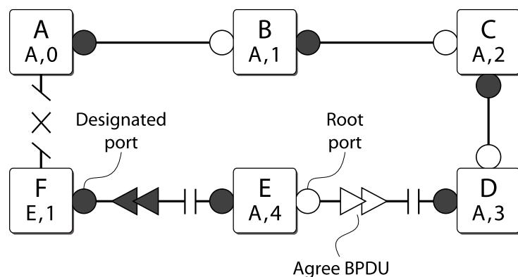
Figure 177: Communicating Port Status to Neighbors
