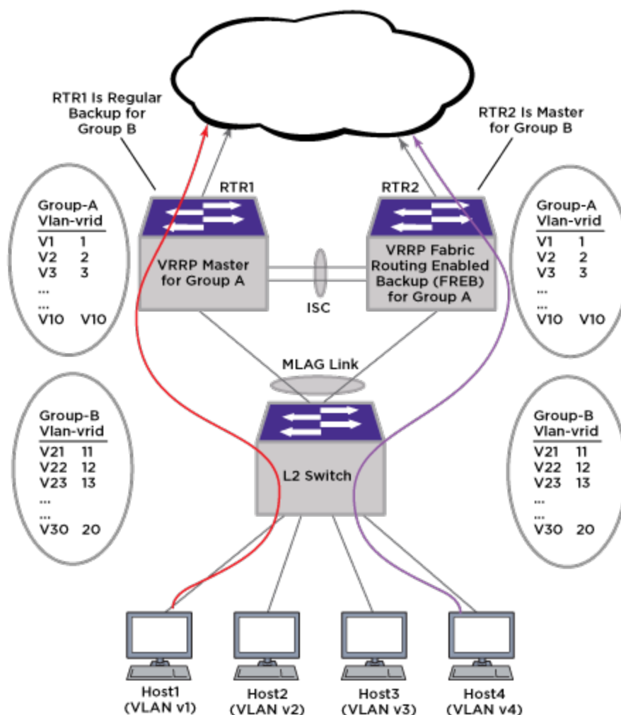
Figure 202: Example VRRP Group Configuration
