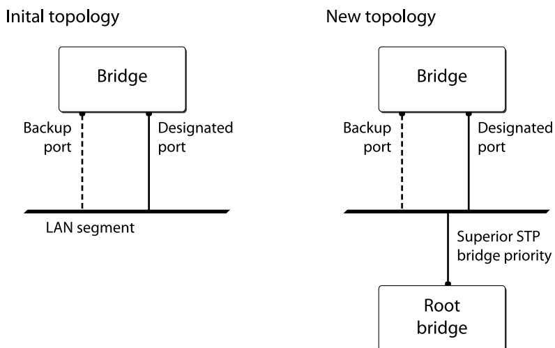
Figure 171: Example of Root Port Rapid Behavior
