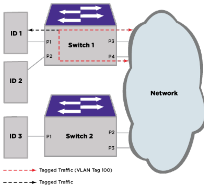
Figure 120: Untagged Traffic Topology
