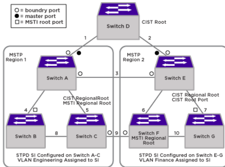
Figure 189: MSTP Configuration Example
