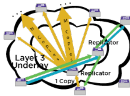
Figure 115: Assisted Replication with Multiple Replicators
