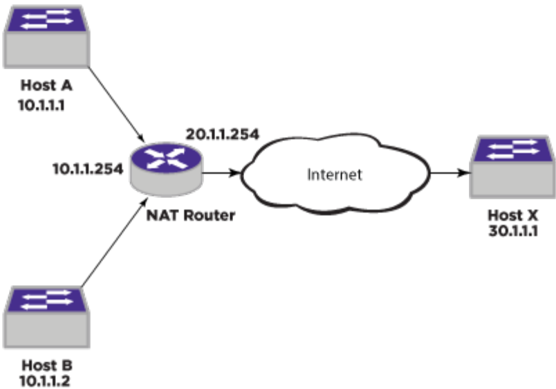
Figure 233: Example Network for NAT and NATP
