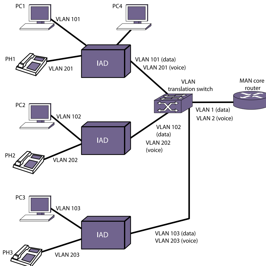
Figure 69: VLAN Translation Application
