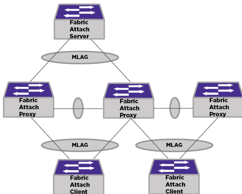
Figure 92: Fabric Attach with W-MLAG
