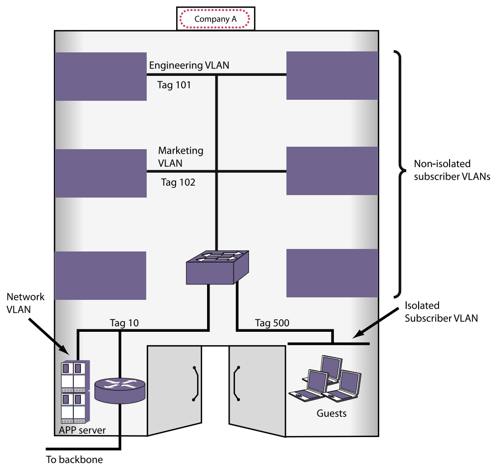
Figure 70: VLAN Isolation Application
