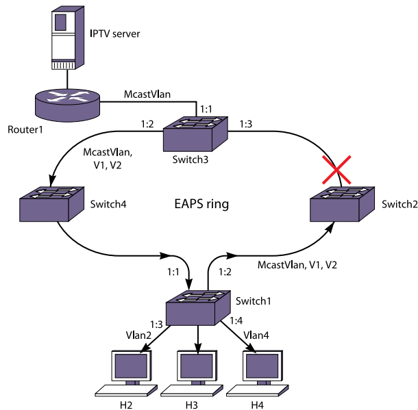
Figure 281: MVR on an EAPS Ring
