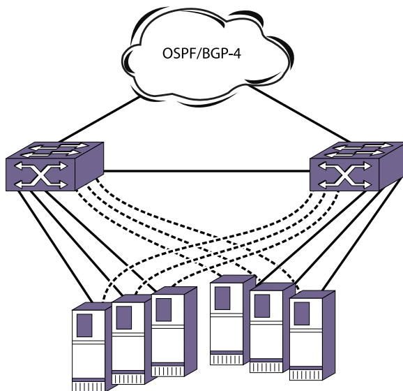
Figure 193: ESRP Host Attach
