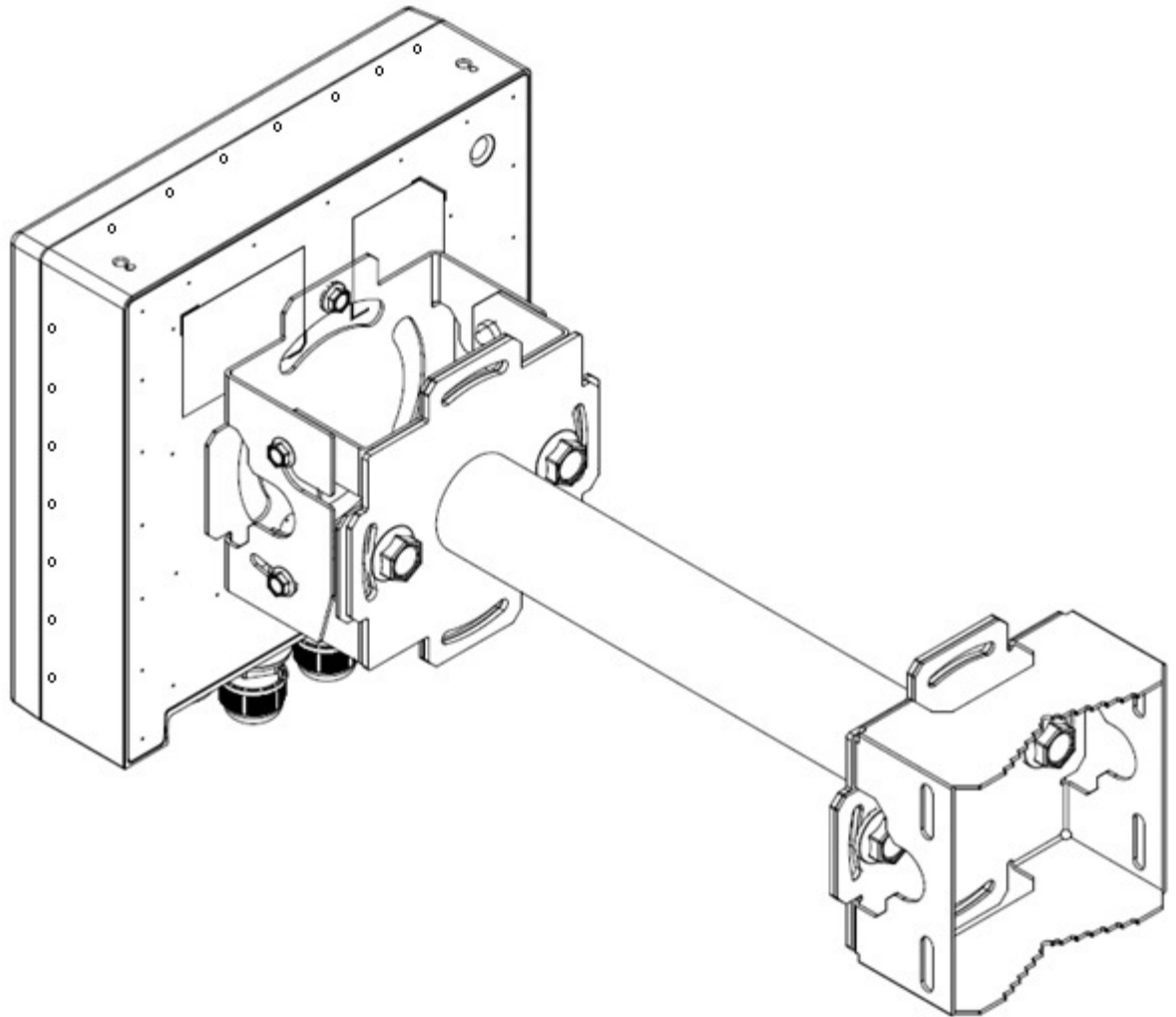
Figure 11: Attaching the KT-150173-01 extension arm to the 1-axis tilt part of the KT-147407-02 bracket
