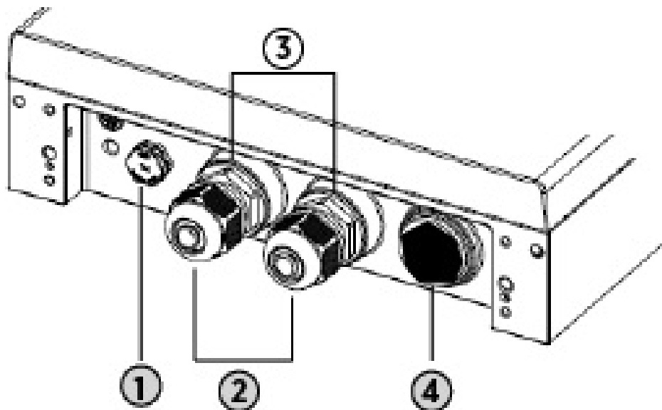
Figure 3: AP5050D Gland Body
