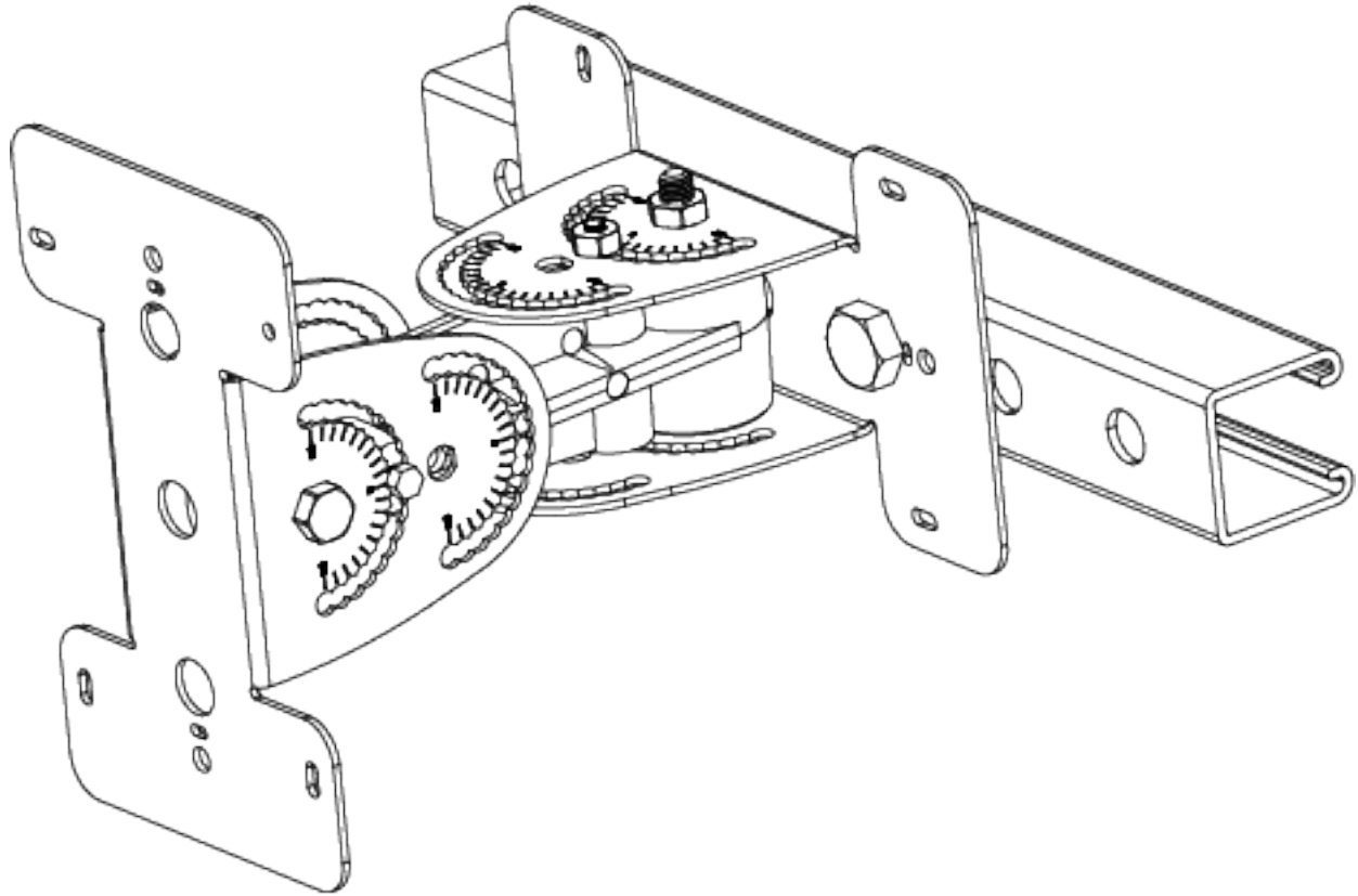
Figure 13: MBO-ART03 bracket angular adjustments
