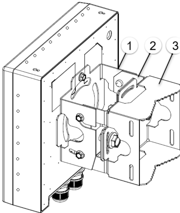
Figure 10: AP5050U access point with KT-147407-02 bracket parts
