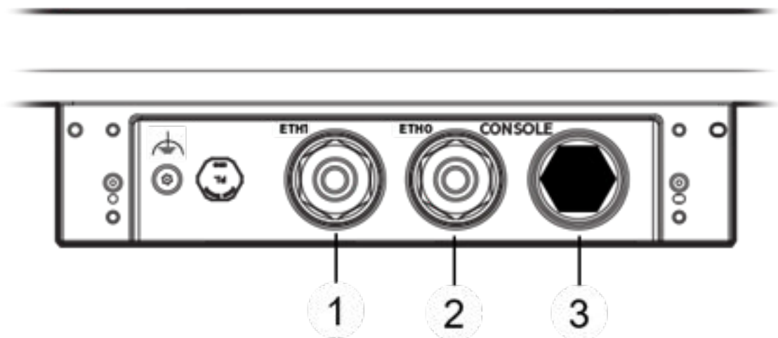
Figure 1: AP5050D Side Ports
