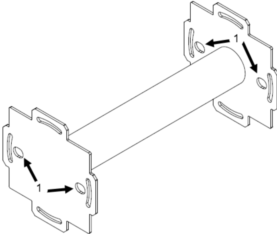
Figure 7: KT-1501730-01 Extension Arm Attachment Holes
