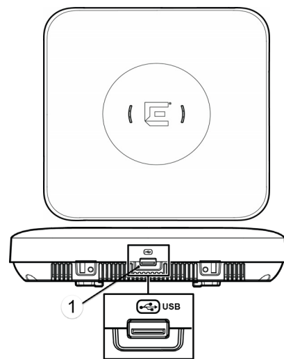
Figure 1 Top and Side View of AP505i
