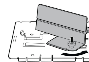
Figure 4 Attaching the adapter to the main bracket
