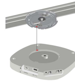
Figure 3 Access point alignment against the red dot on the -TB bracket
