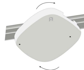
Figure 4 AP410C access point ceiling install
