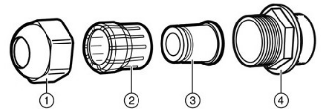
Figure 4 AP5050U Glands
