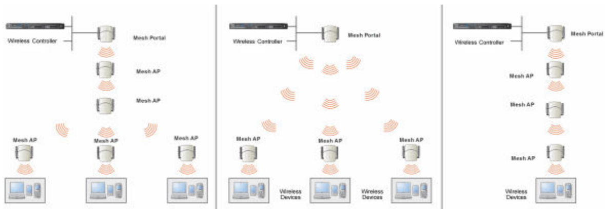
Figure 151: Examples of Mesh Deployment
