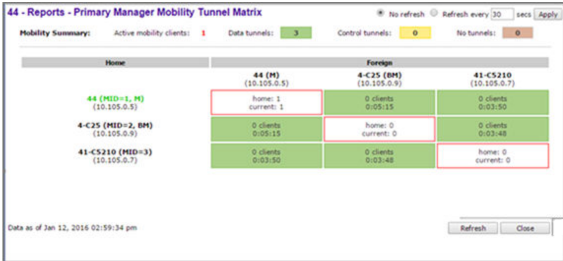
Figure 208: Primary/Backup Manager Mobility Tunnel Matrix
