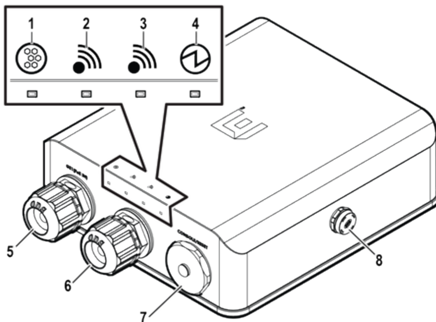
Figure 59: AP3917i LEDs and Features
