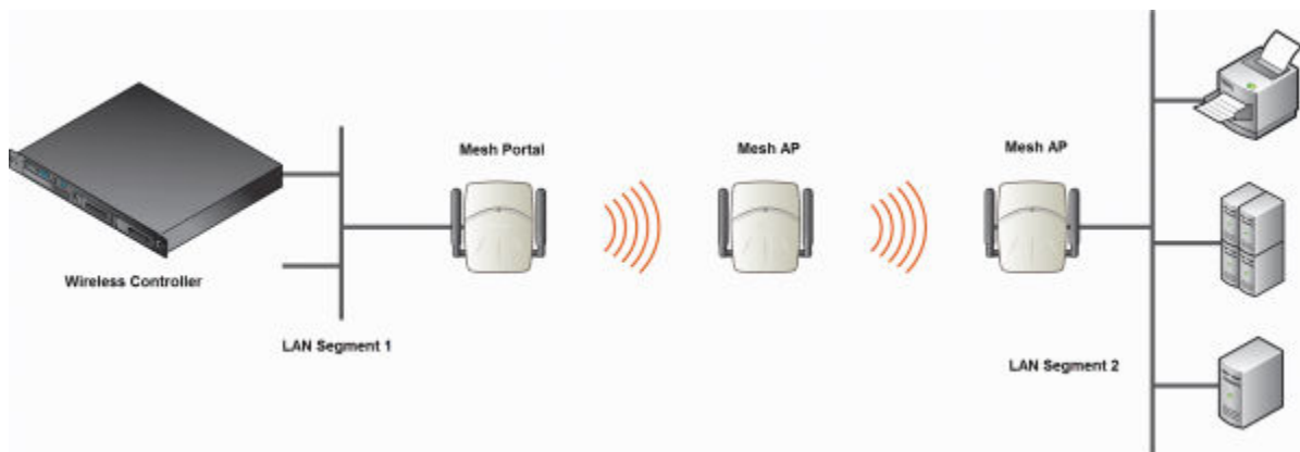
Figure 160: Wireless Bridge Configuration
