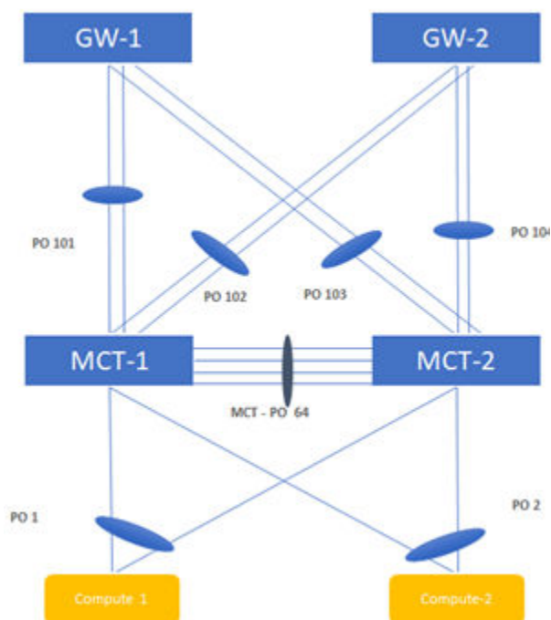
Figure 23: Topology
